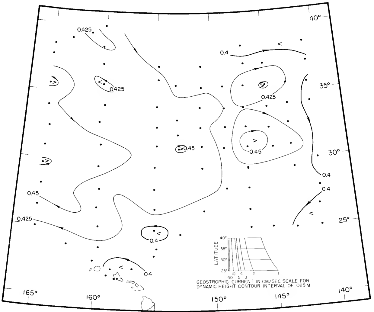
Figure 21. --Anomaly of geopotential topography of the 600-db. surface relative to the 1,000-db. surface. Points indicate computed values.
