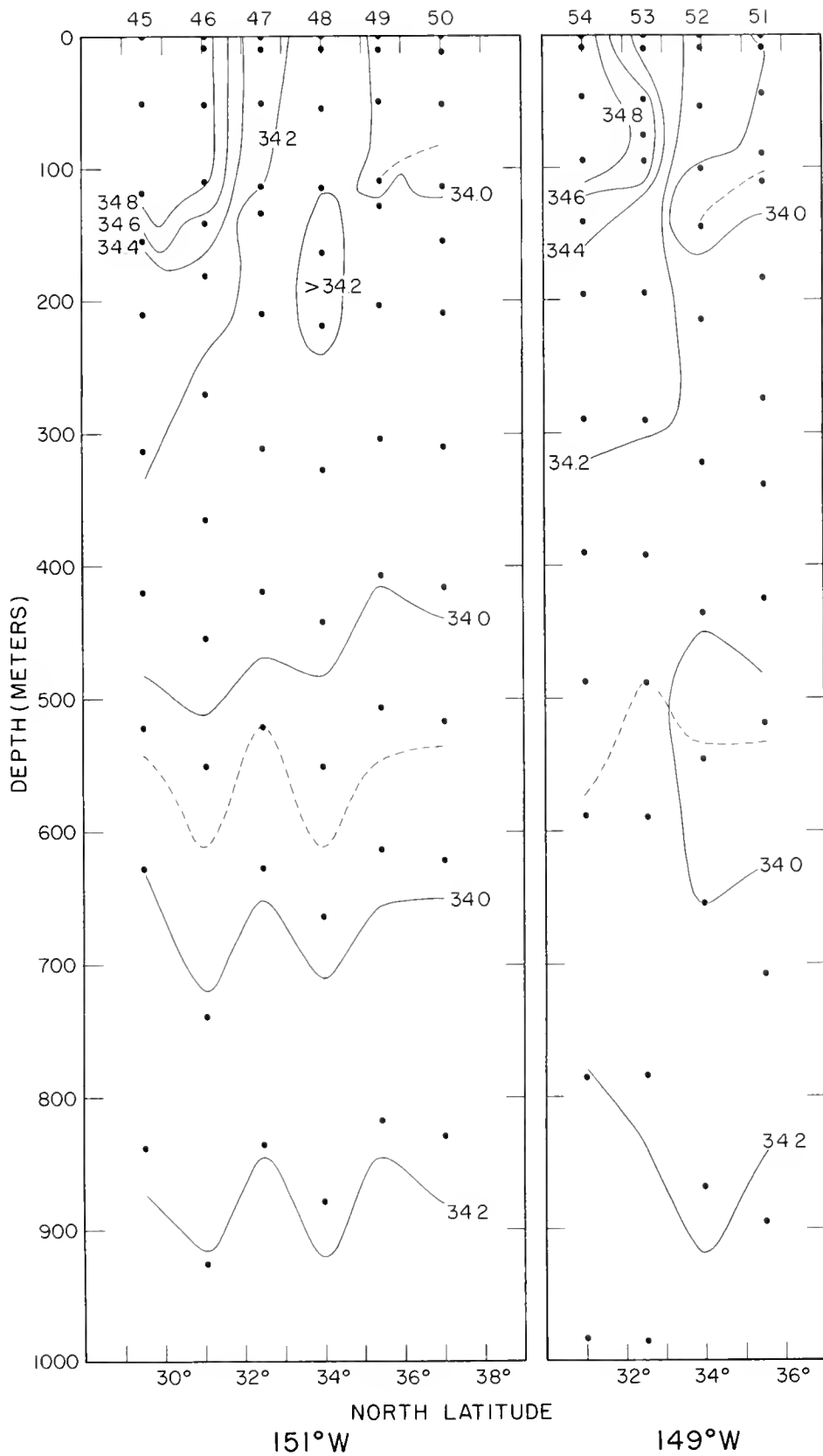
Figure 56.--Vertical section of salinity in parts per thousand along 151°W. longitude, stations 45-50. Dotted lines indicate depths of salinity minima. Points indicate observed values. Figure 57.--Same for 149°W. longitude, stations 51-54.
