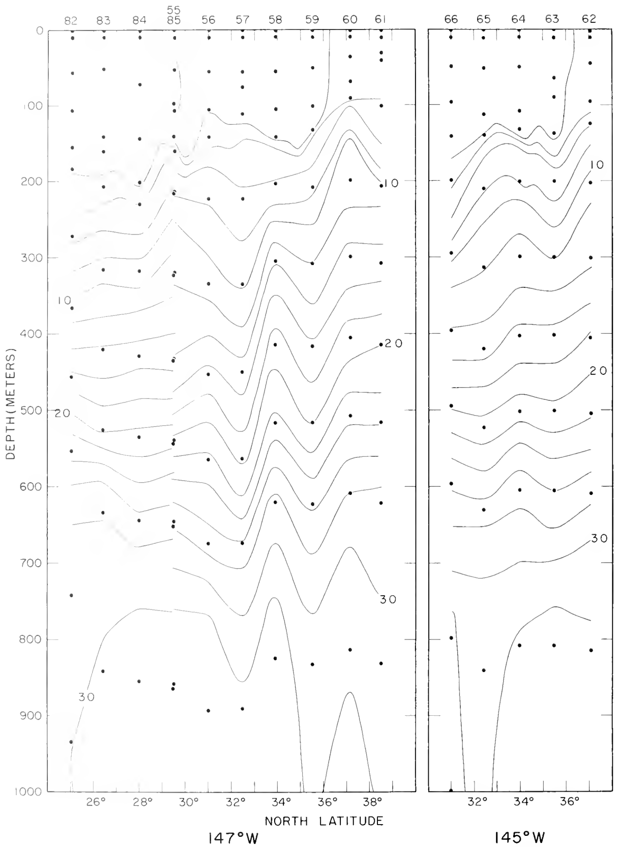
Figure 90. -- Vertical section of inorganic phosphate in microgram-atoms per liter along 147°W. longitude, stations 55-61 and 82-85. Points indicate observed values. Figure 91. -- Same for 145°W. longitude, stations 62-66.
