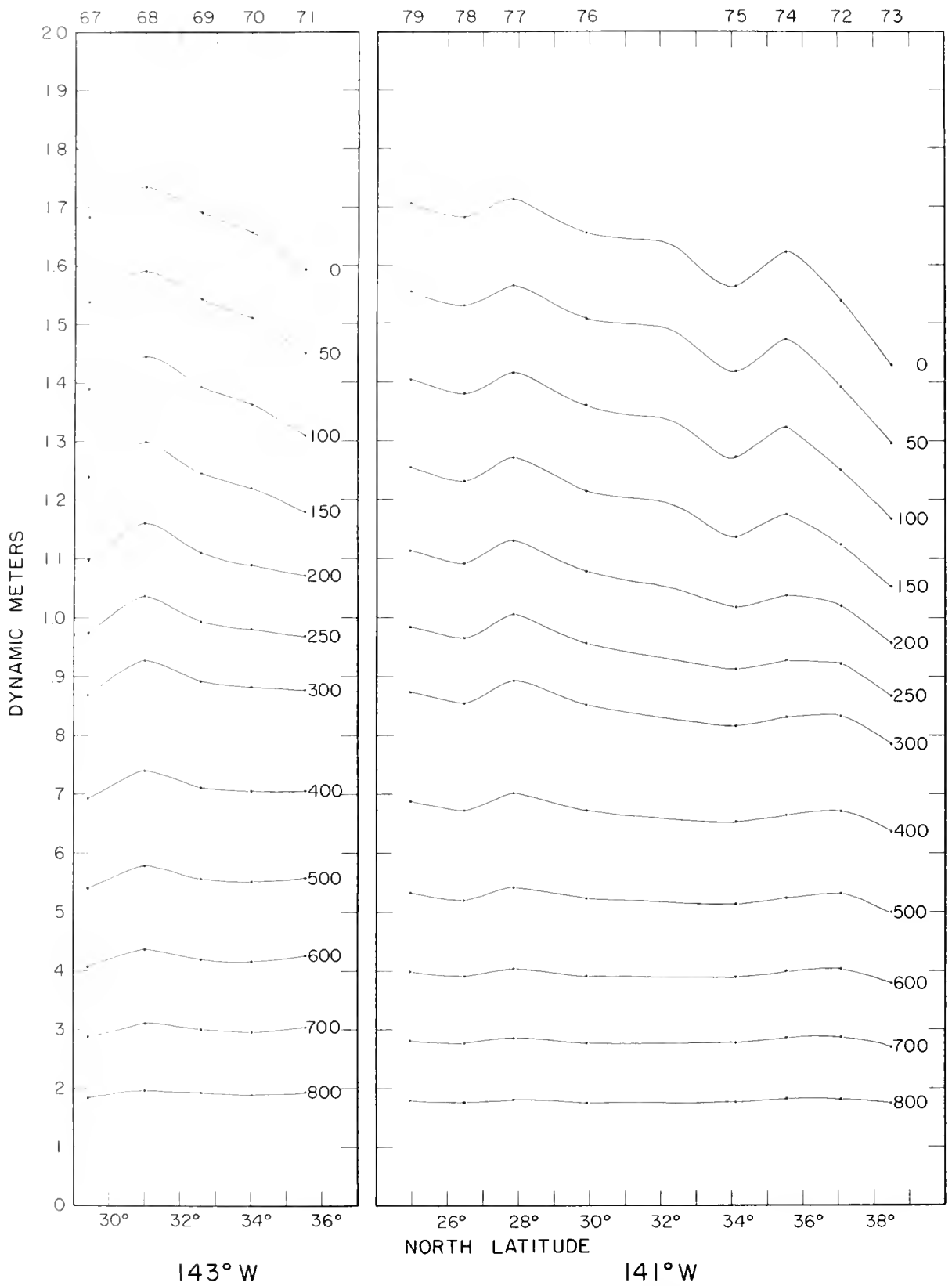
Figure 15. --Smoothed geopotential anomaly of isobaric surfaces relative to the 1,000-db. surface along 143° W. longitude, stations 67-71. Points represent computed values. Figure 16. --Same for 141° W. longitude, stations 72-79.
