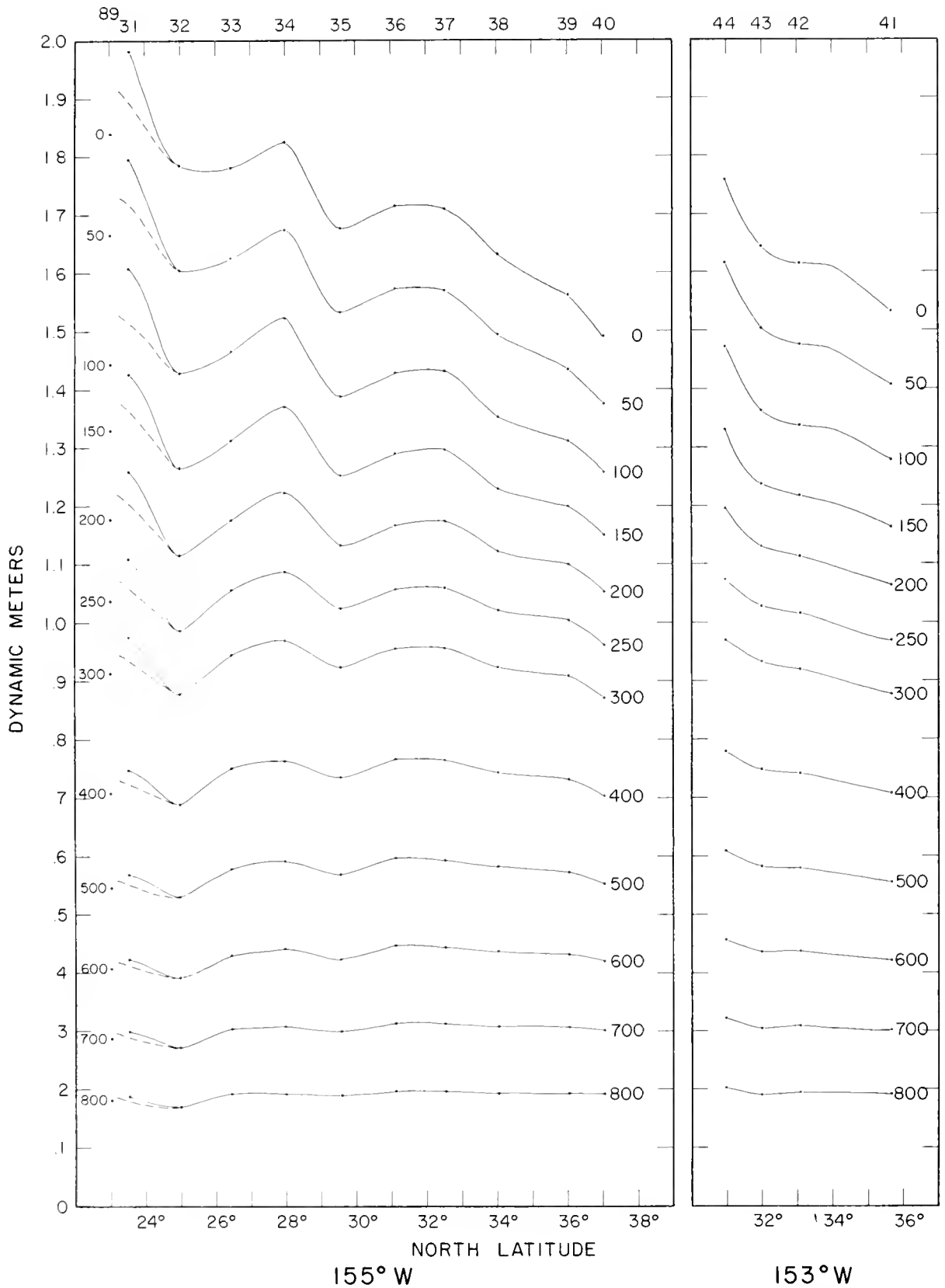
Figure 9. --Smoothed geopotential anomaly of isobaric surfaces relative to the 1,000-db. surface, along 155°W. longitude, stations 31-40. Points represent computed values. Figure 10. --Same for 153°W. longitude, stations 41-44.
