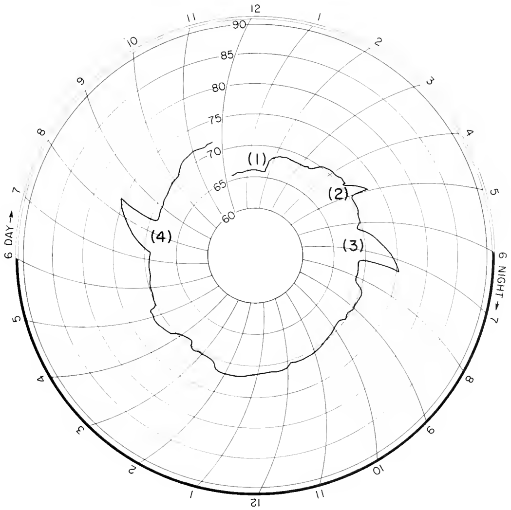
Figure 35. --Sample trace from surface recording thermograph. (1) Period of rapid temperature change; (2), (3), and (4) periods when vessel was stopped. Note: instrument was adjusted to read approximately 8^{\circ} high, in order to keep the trace on scale.
