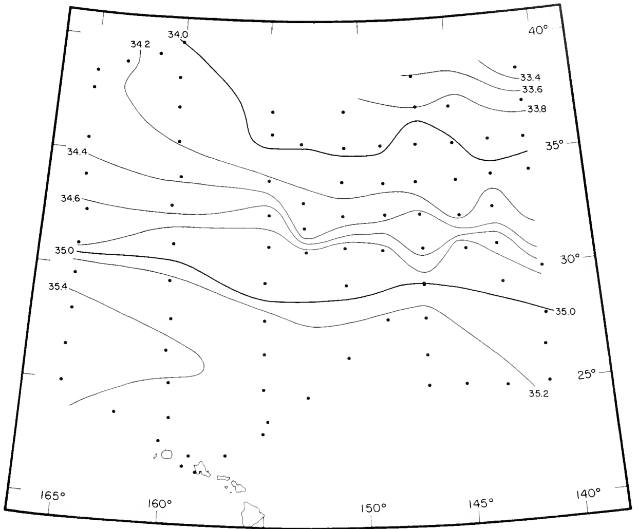
Figure 51. --Surface salinity in parts per thousand. Points indicate observed values.
