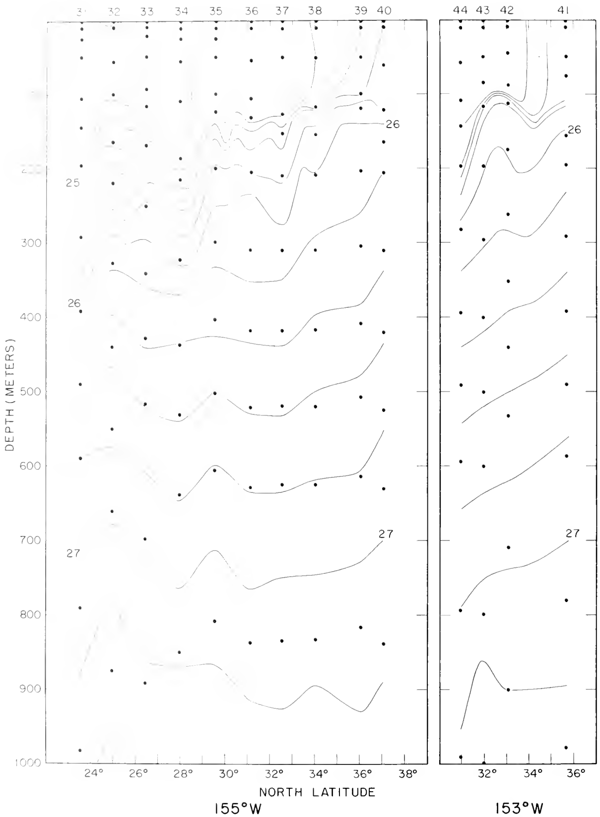
Figure 40.--Vertical section of \sigma\text{-t} along 155^{\circ}\text{W} . longitude, stations 31-40. Points indicate observed values. Figure 41.--Same for 153^{\circ}\text{W} . longitude, stations 41-44.
