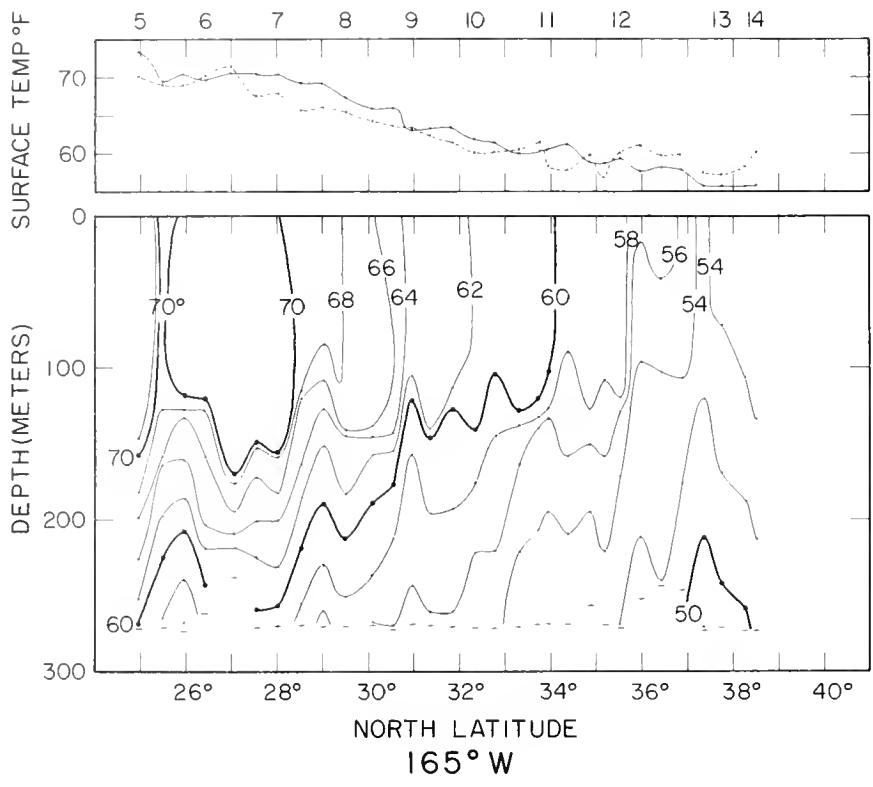
Figure 24. --Temperature sections from BT casts along 165^{\circ}\text{W} . longitude, stations 5-14. Upper panel air (dotted) and surface (solid) temperatures. Lower panel temperature from BT slides. Dashes indicate depth of casts.
