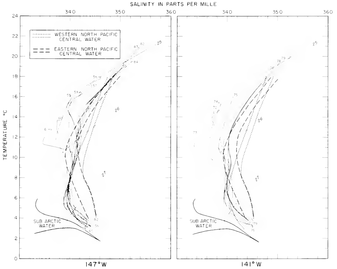
Figure 70.--Superimposed temperature-salinity curves for the meridional station series along 147°W. longitude, stations 55-61 and 82-85.
