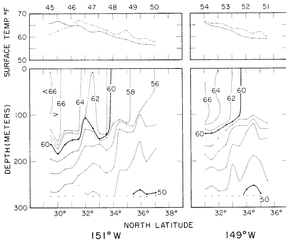
Figure 28.--Temperature sections from BT casts along 151^{\circ}\text{W} . longitude, stations 45-50. Upper panel air (dotted) and surface (solid) temperatures. Lower panel temperatures from BT slides. Dashes indicate depth of casts.
