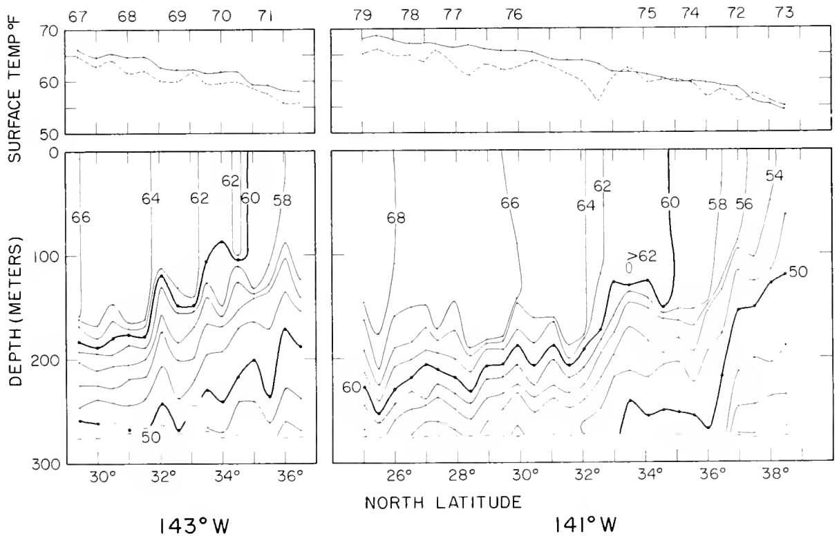
Figure 32. --Temperature sections from BT casts along 143^{\circ}\text{W} . longitude, stations 67-71. Upper panel air (dotted) and surface (solid) temperatures. Lower panel temperature from BT slides. Dashes indicate depth of casts.
