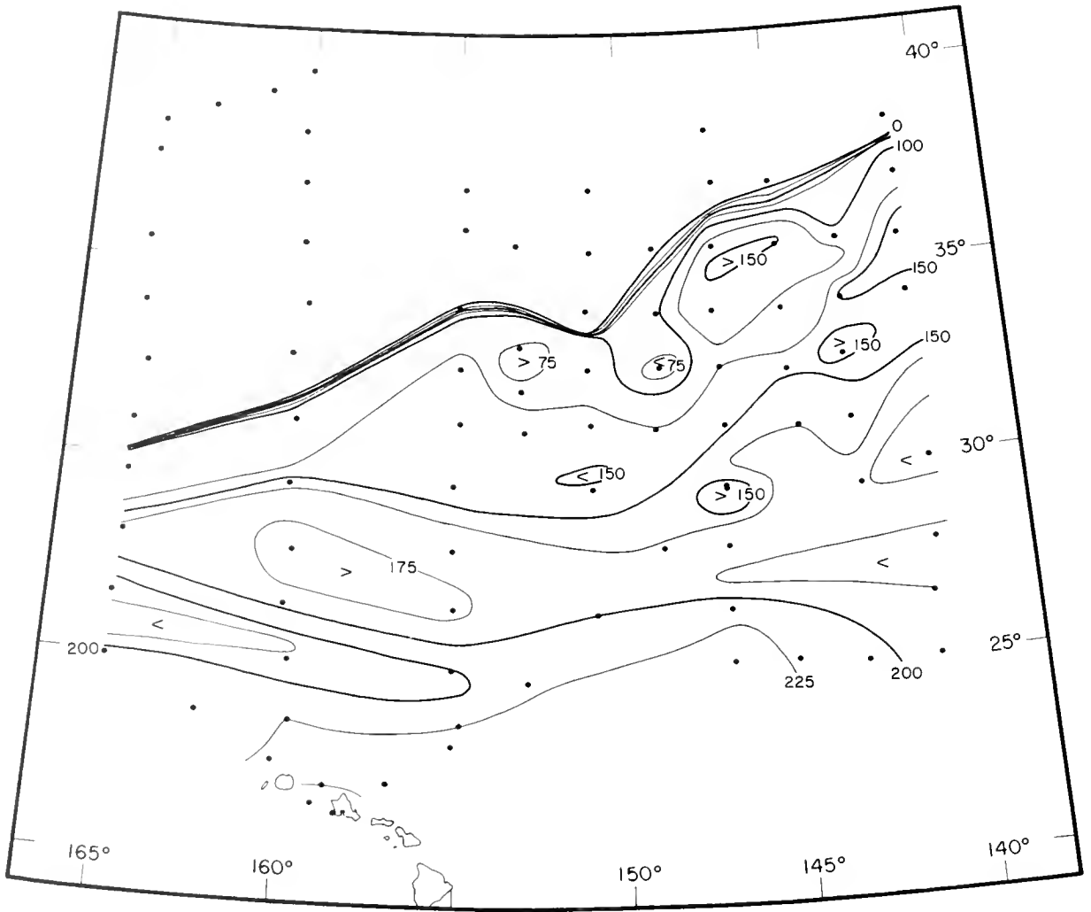
Figure 48. --Depth of 25.2 sigma-t surface in meters. Points indicate station positions.
