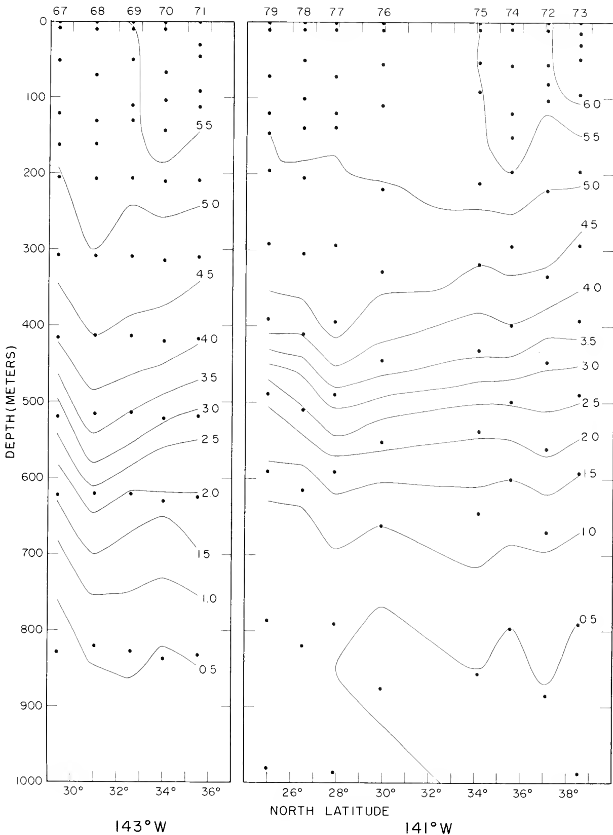
Figure 80.--Vertical section of oxygen in milliliters per liter along 143°W. longitude, stations 67-71. Points indicate observed values.
