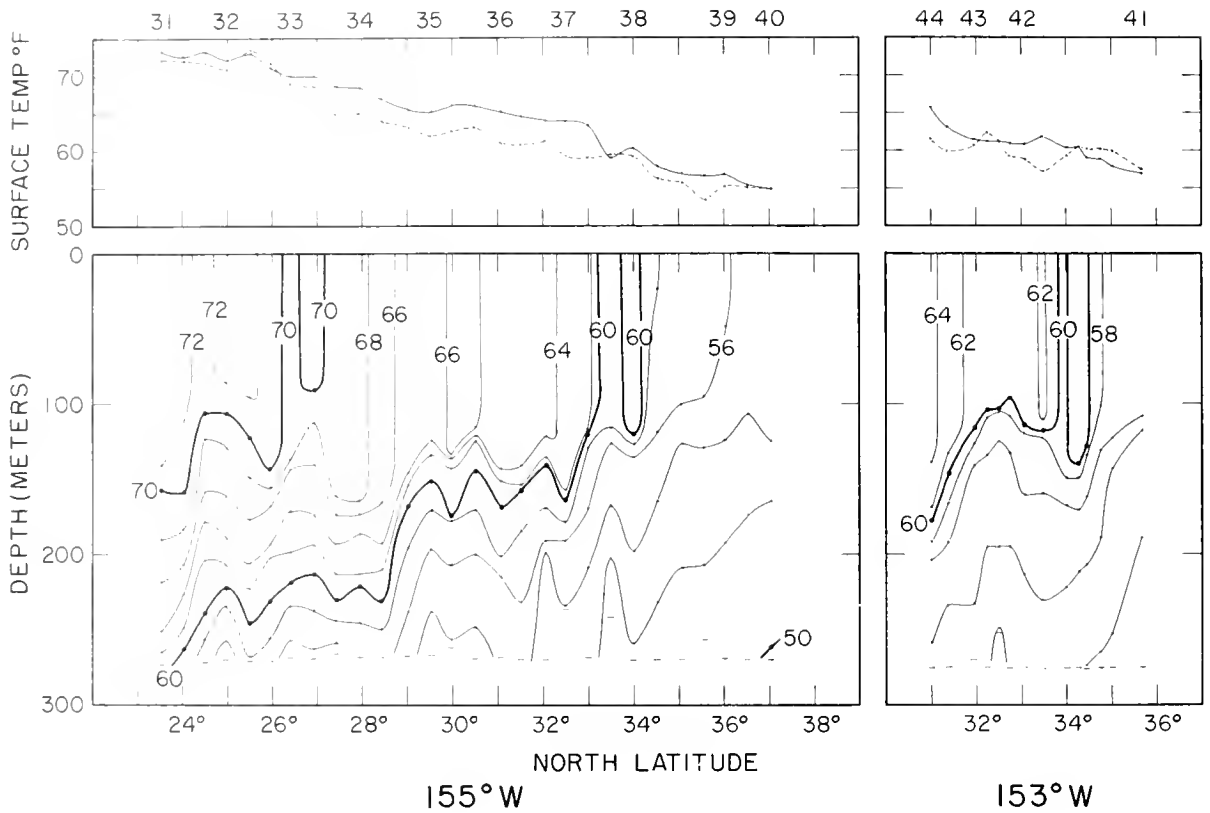
Figure 26. --Temperature sections from BT casts along 155°W. longitude, stations 31-40. Upper panel air (dotted) and surface (solid) temperatures. Lower panel temperatures from BT slides. Dashes indicate depth of casts.
