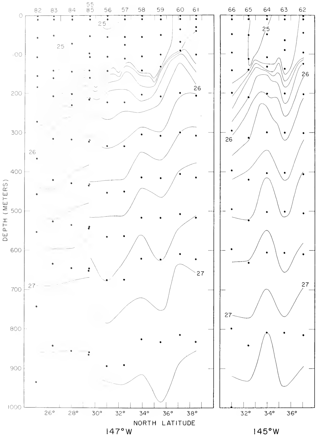
Figure 44.--Vertical section of \sigma\text{-t} along 147^{\circ}\text{W} . longitude, stations 55-61.
