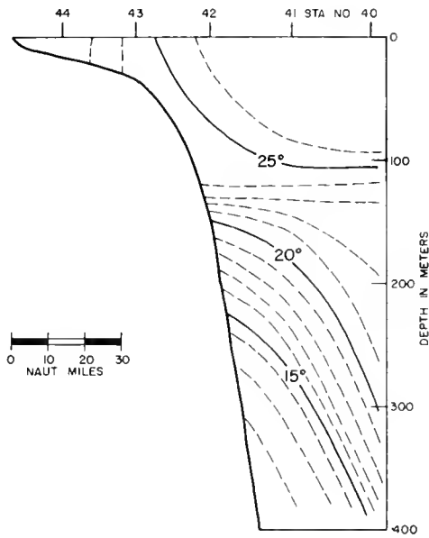
Figure 13.--Distribution of temperature (°C) across section of stations 40, 41, 42, 43, and 44 (Charleston Section).
