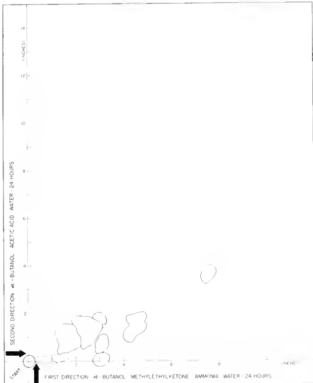
Figure 4. -- Two-dimensional chromatogram of adult albacore.
