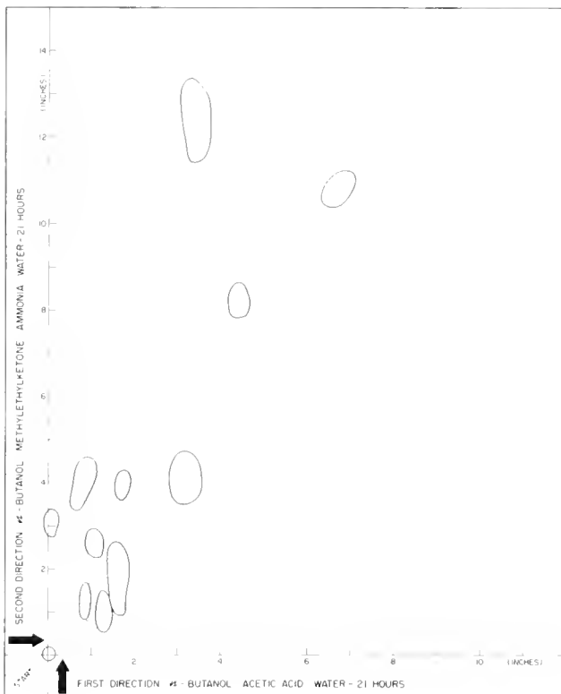
Figure 9. --Two-dimensional chromatogram of adult yellowfin run in reverse order of solvents.
