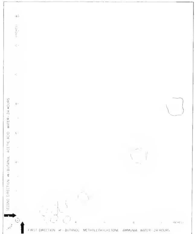
Figure 11. --Two-dimensional chromatogram of larval skipjack.
