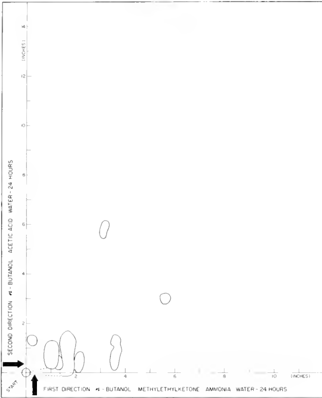
Figure 6. -- Two-dimensional chromatogram of adult yellowfin.
