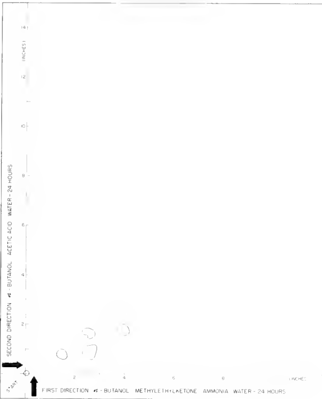
Figure 10. --Two-dimensional chromatogram of larval yellowfin.
