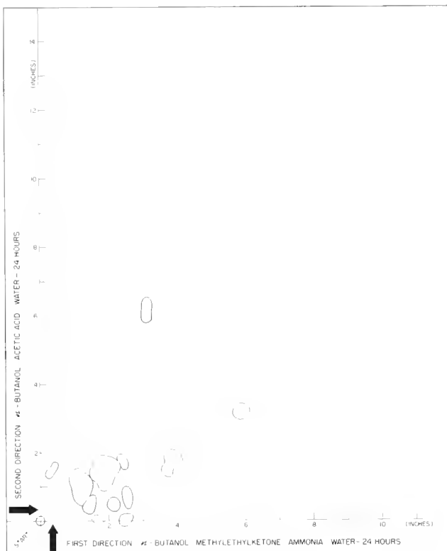
Figure 5. -- Two-dimensional chromatogram of adult bigeye.
