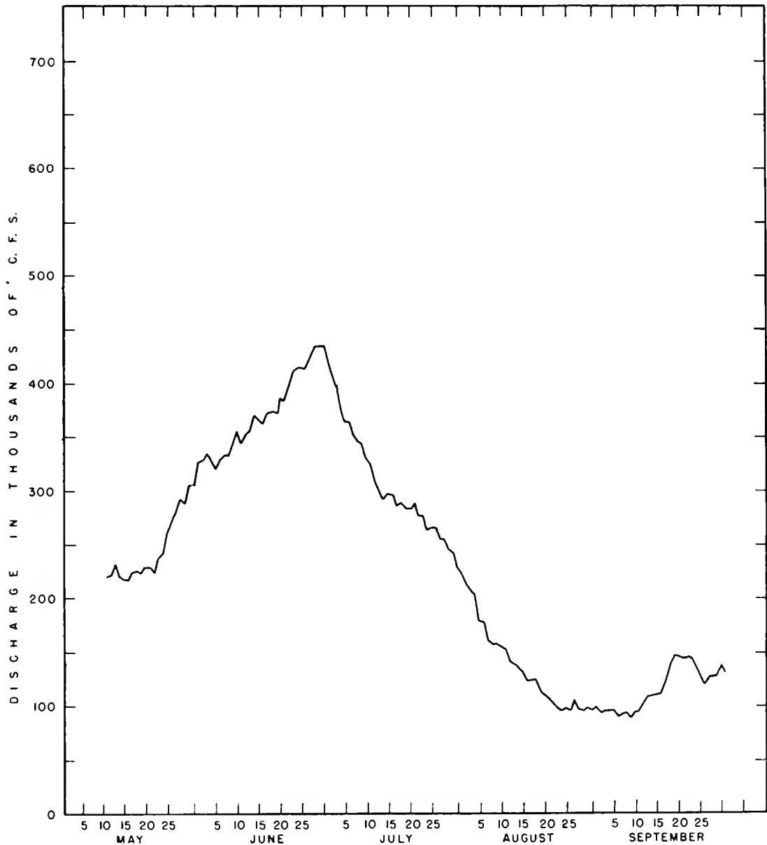
Figure 3.--Daily river discharge, Rock Island Dam, May 10-September 30, 1959
