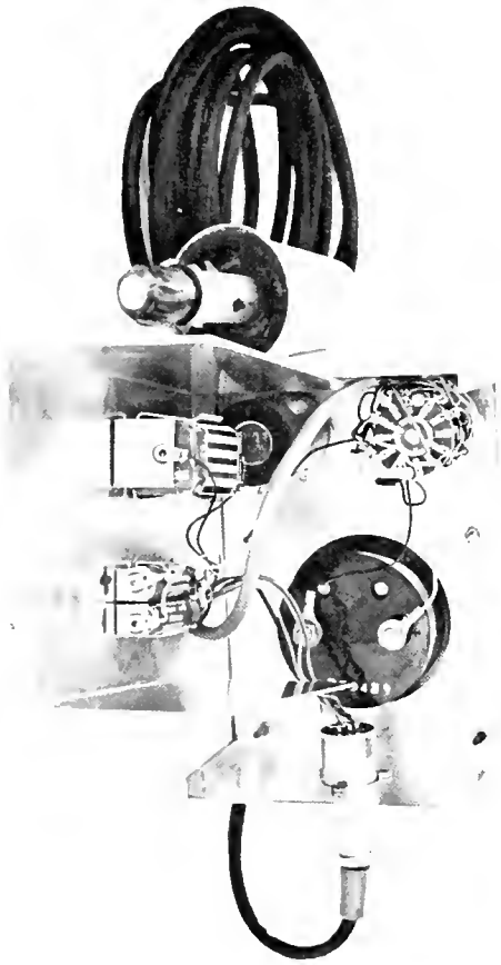
Photograph 2:--Inside view of oxygen-temperature meter.
