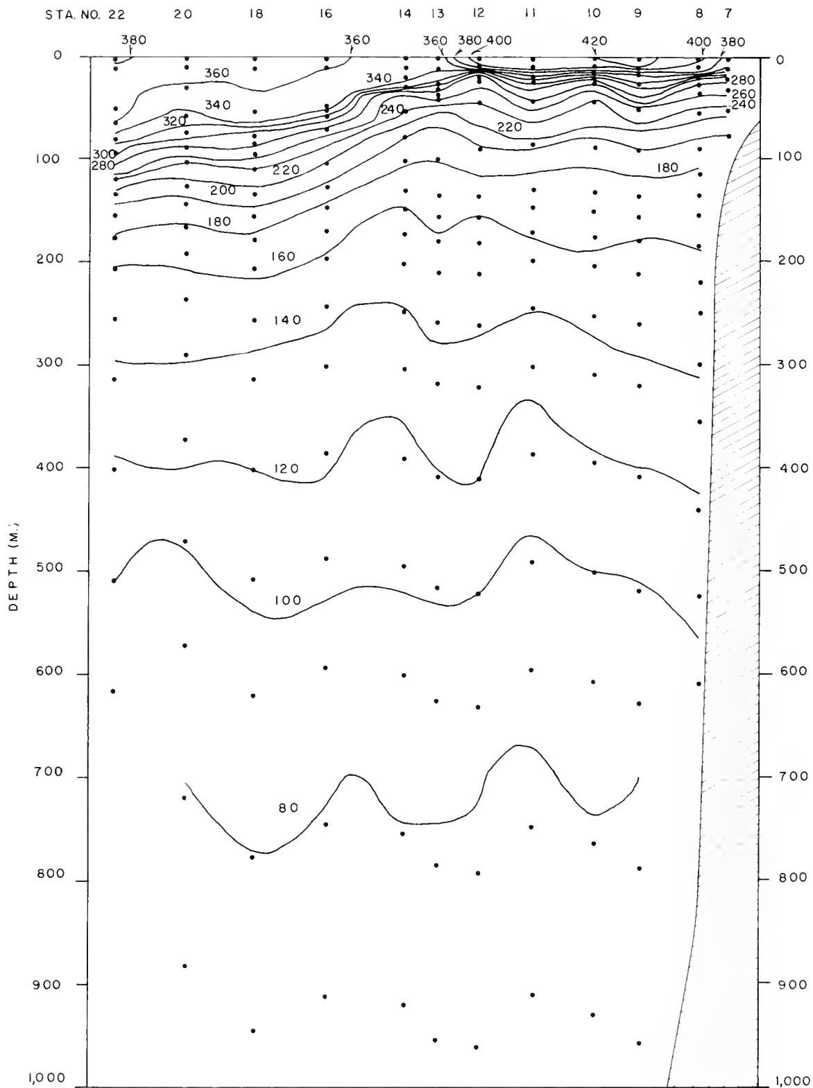
Figure 25.--Vertical profile of thermocline anomaly along the line of stations, 7 to 22, on cruise TO-60-1. The contour interval is 20 ci./metric ton.
