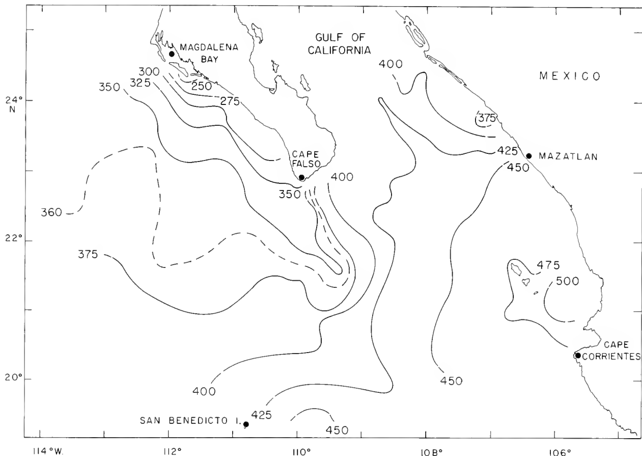
Figure 33.--Horizontal distribution of thermosteric anomaly at the sea surface for part of CalCOFI cruise 6004-B and for cruise TO-60-1. The contour interval is 25 cl./metric ton.
