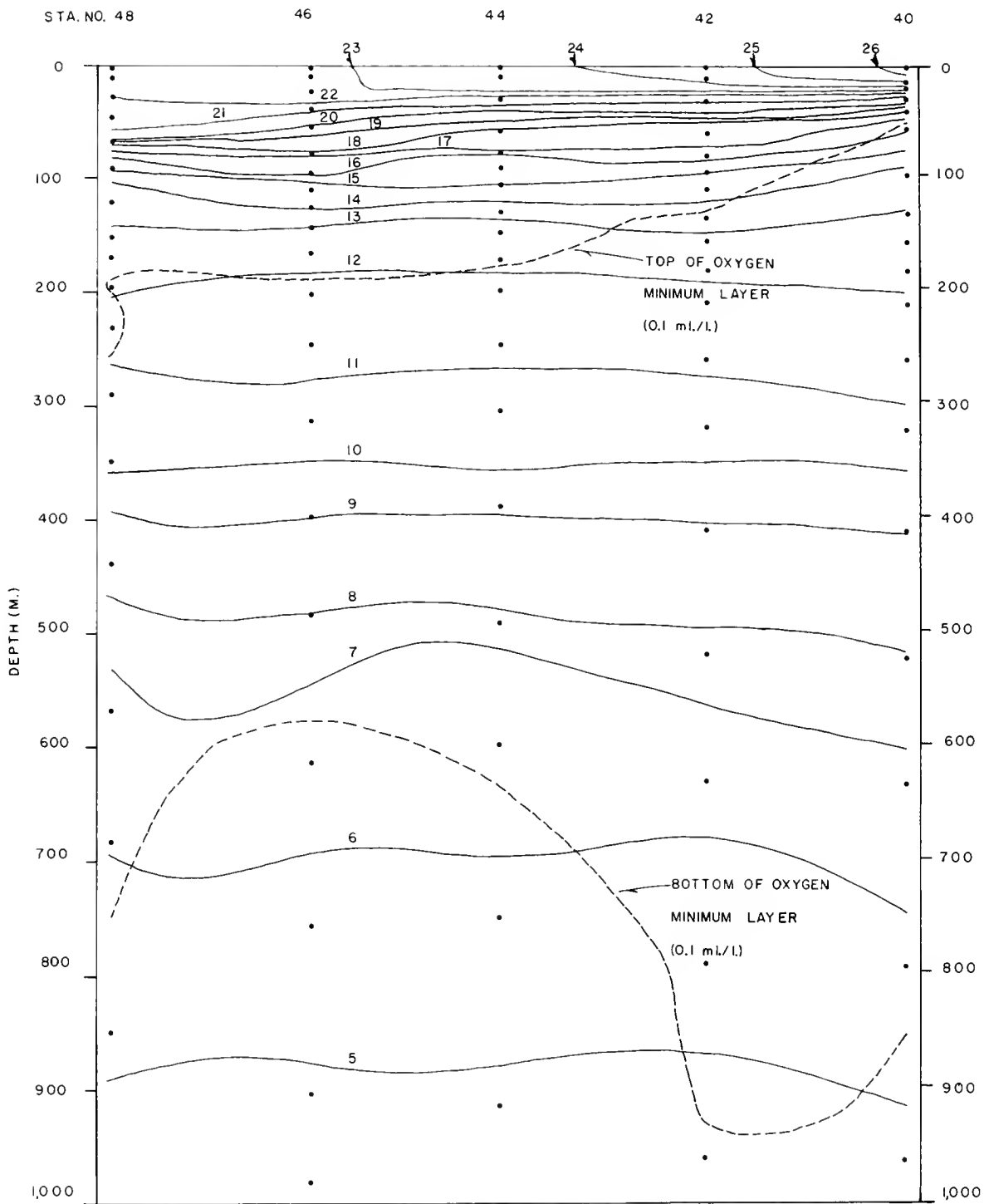
Figure 13.--Vertical temperature profile of the line of stations, 40 to 48, on cruise TO-60-1.
