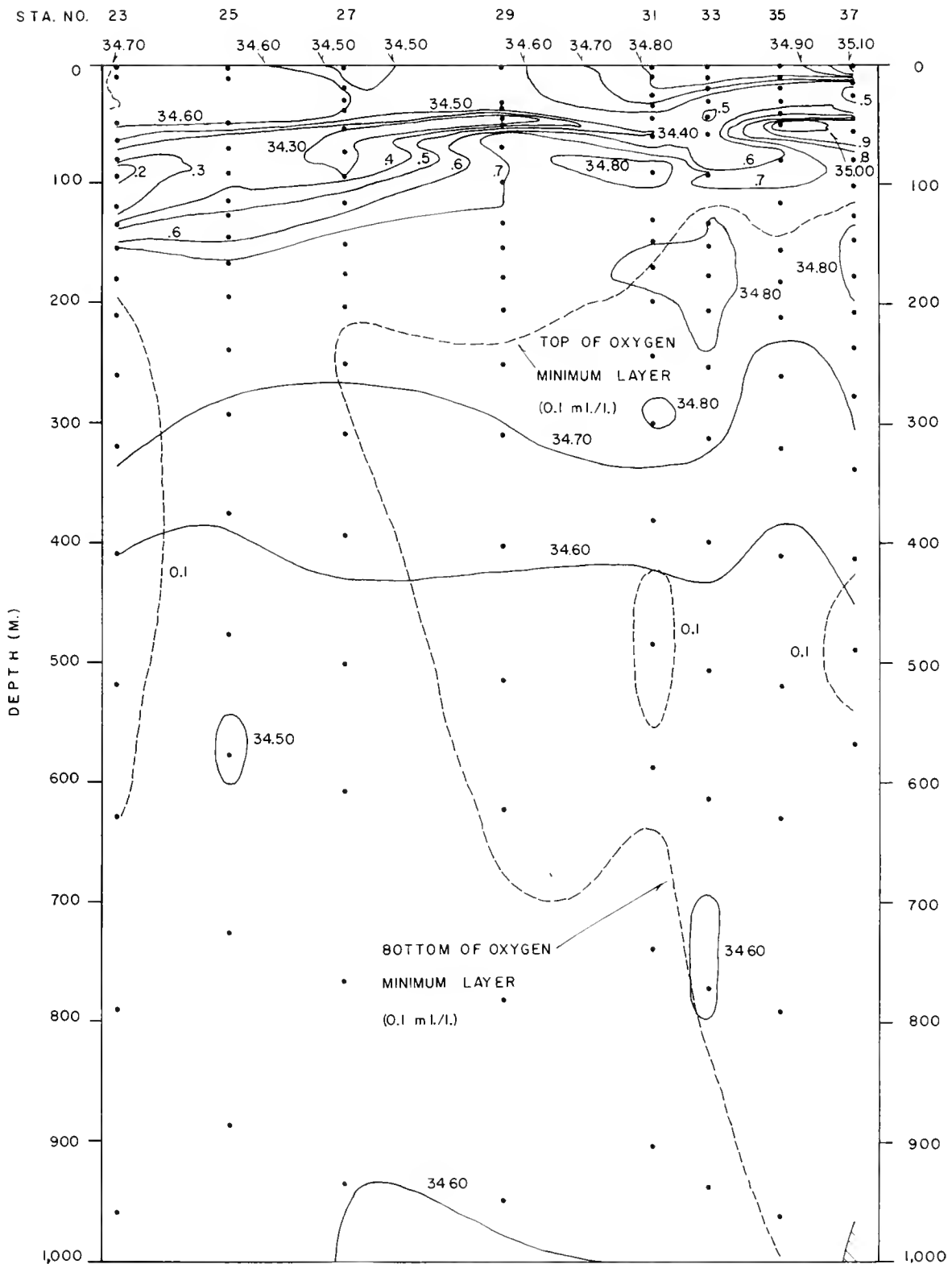
Figure 22.--Vertical salinity profile along the line of stations, 23 to 37, on cruise TO-60-i.
