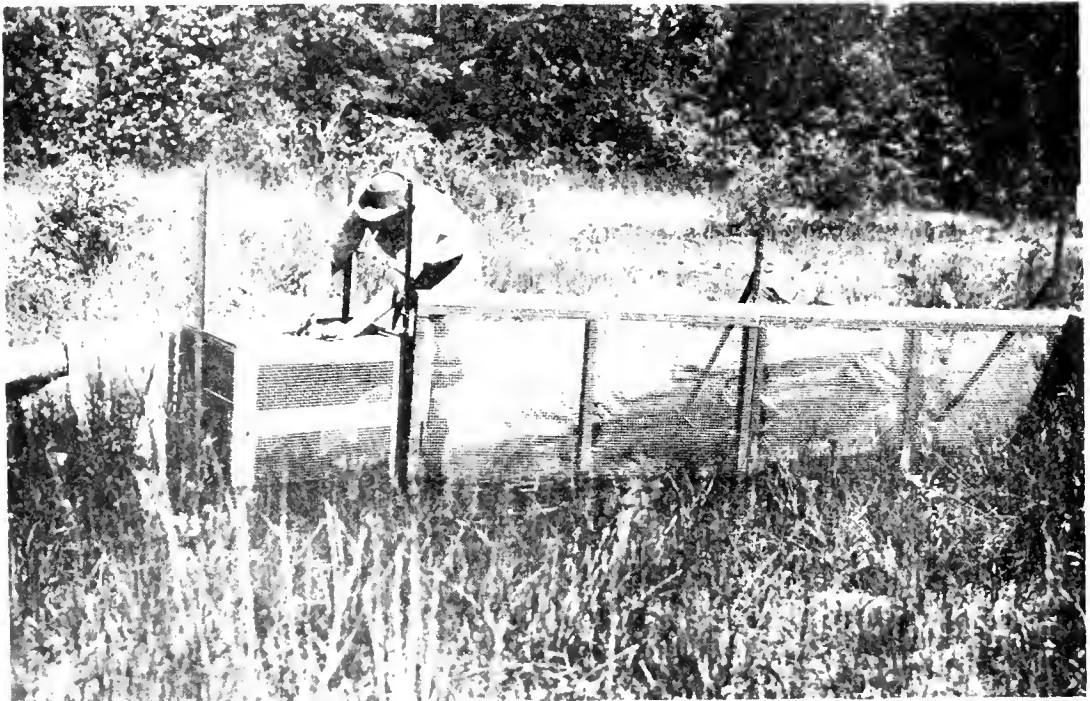
Figure 4.—Small portable-type weir and trap in Cedar Creek, Presque Isle County, Michigan
