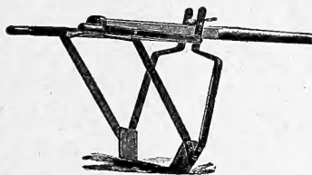
THE BOHLEN CELERY DIGGER.
