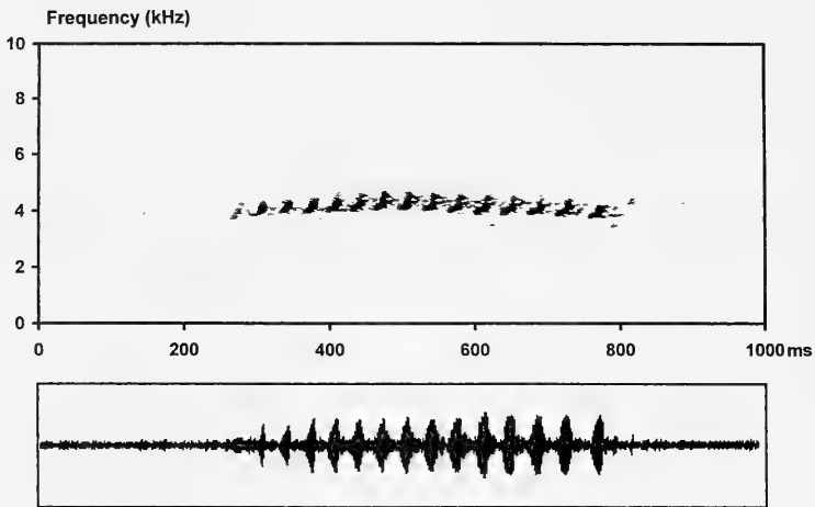
Fig. 7. Sonagram and oscillogram of a call (one note) of Boophis andohahela from Andohahela.
