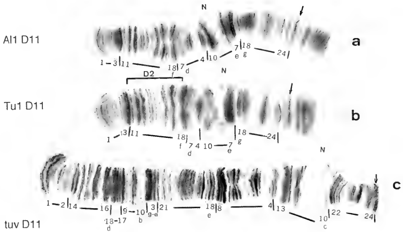
Fig. 3. Banding patterns of arms D. a. C. spec. All. b. C. spec. Tu1. c. C. tuvanicus . Designations as in Figs 1 and 2.
