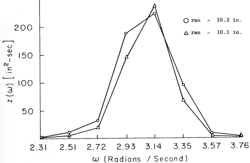
Figure 7 - Comparison of Wave Spectra Measured in Irregular Long-crested Waves in the TMB Deep Water Basin
