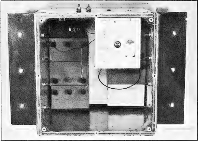
Figure 3 - Top View of SPLASHNIK Instrument Box
