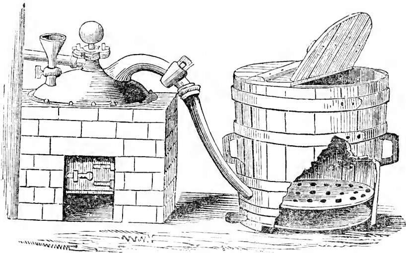
FIG. 17.—STEAMING APPARATUS.
