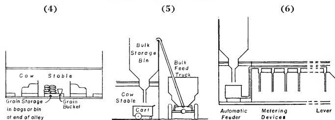
Left: grain stored in stable feed alley. In another variation, grain is stored in bags in a feed room and bags emptied into a bin near feed alley. Bucket is used in feeding. Center: grain stored in a bulk bin located above the stable. Downspout to feed cart. Right: grain stored in a bulk bin located above the stable. This is the Pennsylvania State mechanical dairy feeder. A downspout fills automatic poultry feeder unit. Endless chain fills individual meters above each stanchion. These are set individually. A hand lever is pulled to open meter-bottom slides. A rather costly installation.
