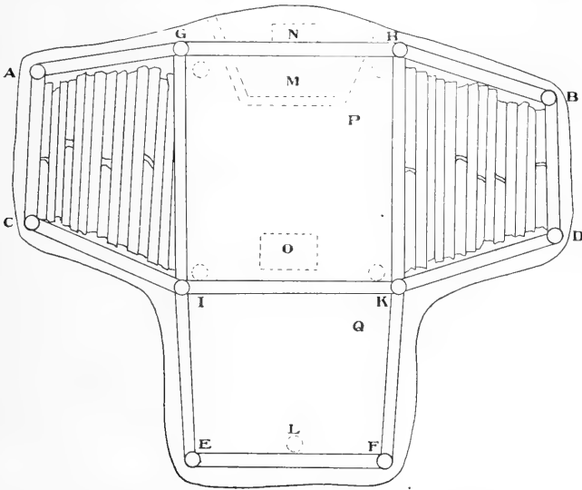
Fig. 88. Plan of a House at Shingle Point. Measurements: A to B, 23'6"; C to D, 24'; G to E, 18'10"; I to E, 8' (H to K and H to F about the same); G to H and I to K, 10'; A to C, 7"; B to D, 6'2"; E to F, 8'10" equals height of G and H, 4'; I and K, 5'10", E, 3'; F, 2'4". (A to F measurement from floor of respective platforms, others from main floor.)
