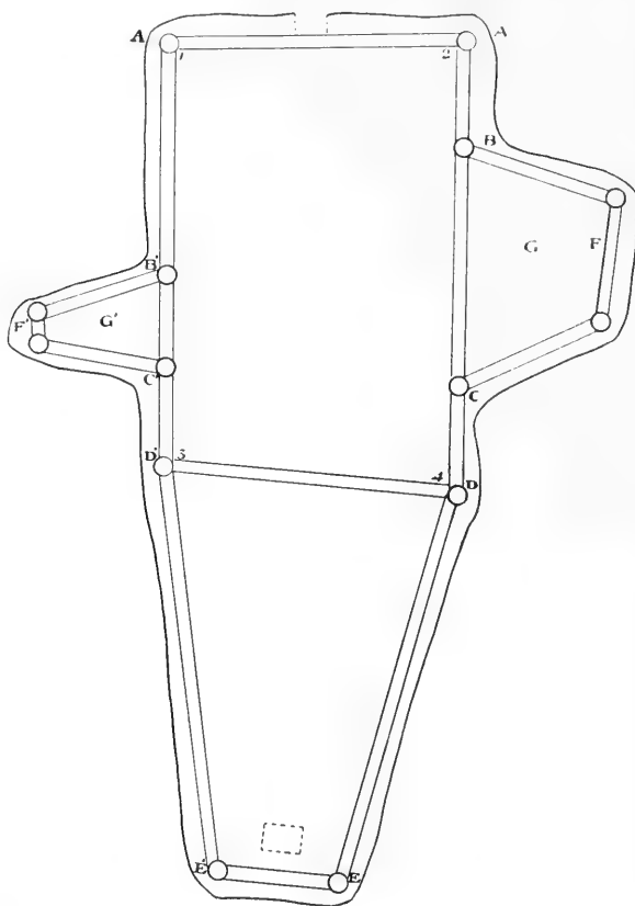
Fig. 87. Plan of a House. Measurements: A to B, 3'2"; A' to B', 6'10"; B to C, 7'; B' to C', 2'; C to D, 2'9"; C' to D', 3'; A' to A, 9'; D' to D, 8'10"; F to AD, 41" F' to A' D', 4'; posts 1, 2, to roof, 5'3"; posts 3, 4, 3'4" (roof one length, sloping logs); D E, to D' E', 10'; E to E', 3'5". The outside of the house is banked with earth. G' is a small storage alcove usually for housing a bitch with pups; it has a flat roof about 2 feet from the floor. G has a roof of the same level as the rest of the passage and sloping towards E. The door is toward the west.
