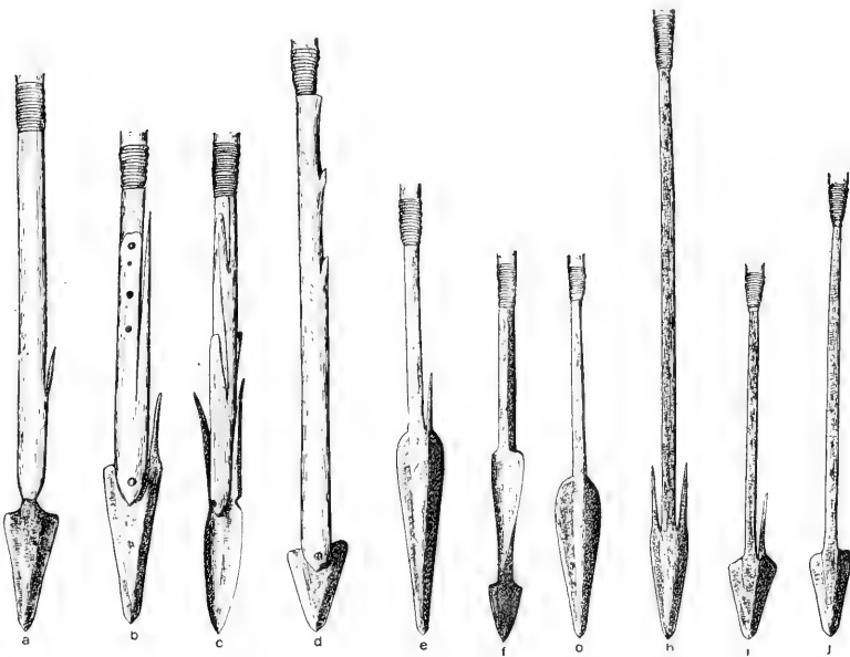
Fig. 35 (60-6938p, e, g, i, h, o, s, f, q, n). Copper Arrow-Heads selected from a single Quiver, Prince Albert Sound, Victoria Island. Length of a, 20 cm.
