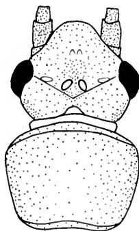
FIG. 20. Neoperla atripennis , female head and prothorax.
