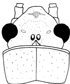
FIG. 21. Neoperla obliqua , male head and prothorax.
