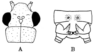
FIG. 24. Phanoperla clarissa : A, male head and prothorax; B, male genitalia, dorsal view.
