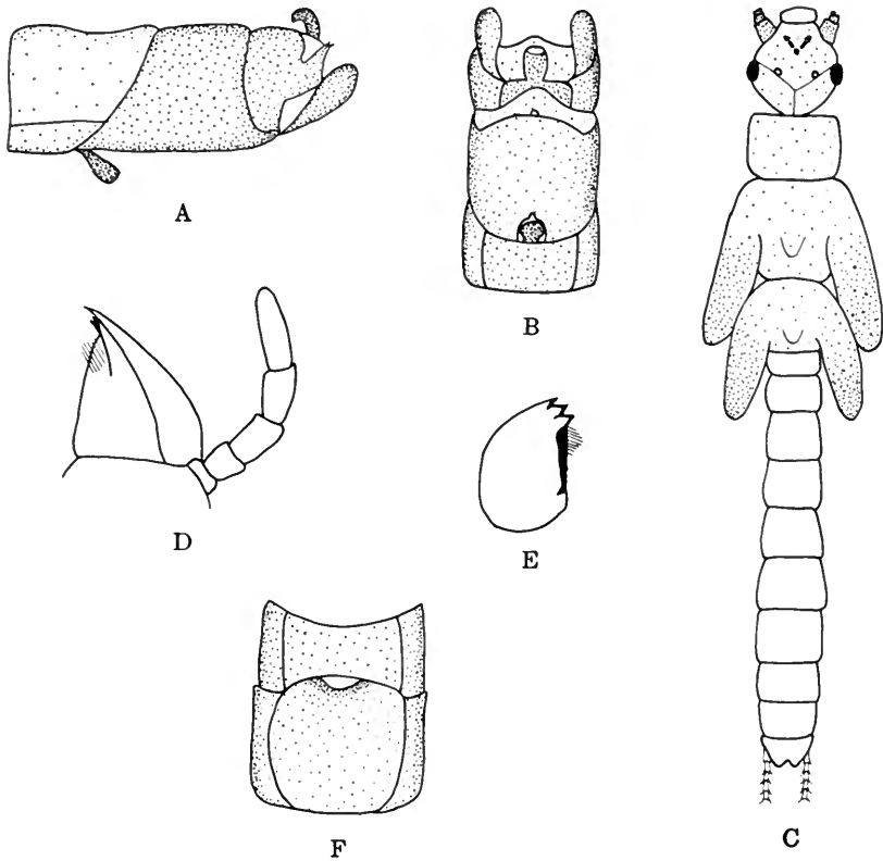
FIG. 18. Leuctra (Rhopalopsola) malayana : A, male genitalia, lateral view; B, male genitalia, ventral view; C, outline of nymph; D, left maxilla of nymph; E, left mandible of nymph; F, female genitalia, ventral view.
