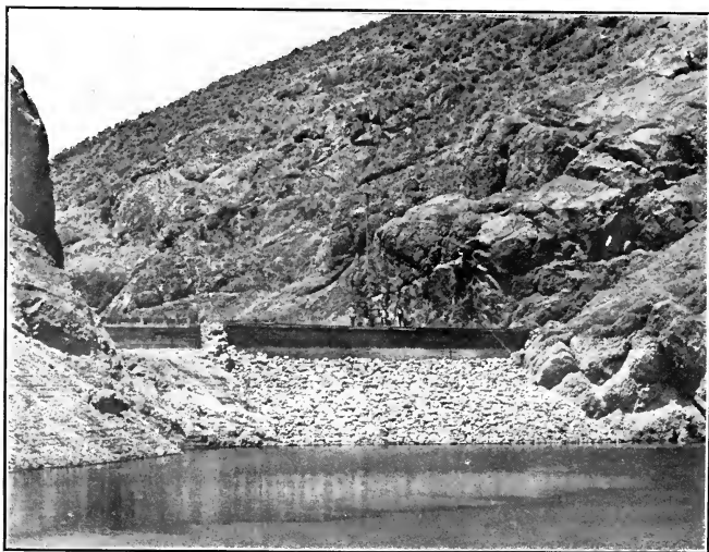
FIG. 2.—SAME, SHOWING STEEL CORE PROJECTING, AND SPILLWAY ON LEFT, AUGUST, 1900.
