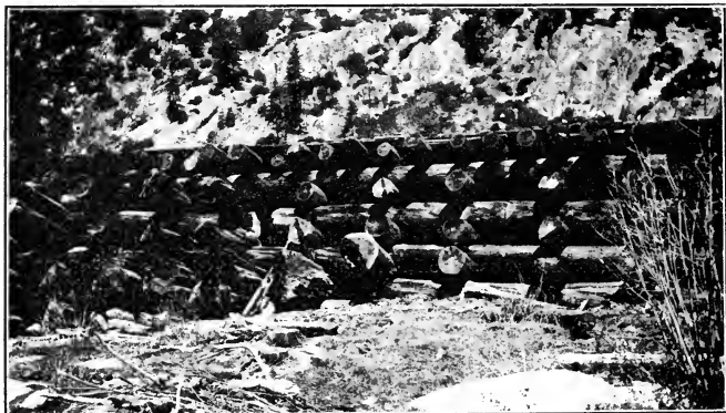
FIG. 5.—Middle Dam, South Fork Stanislaus River, Cal., showing manner of laying logs from the reservoir site. The site was not thoroughly cleared, however, only the best timber suitable for the construction of the dam being used. This standing timber is rotting at the water's edge and
