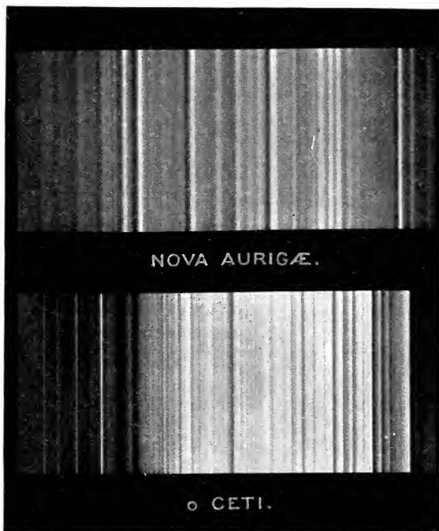
STAR SPECTRA
