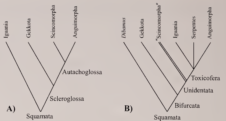
FIG. 1. Phylogenetic relationships of major groups of squamates. (A) The morphological tree. Snakes are alternatively considered to be nested within Anguimorpha (Estes et al. 1988) or Scincomorpha (Conrad, 2008). (B) The molecular tree.
