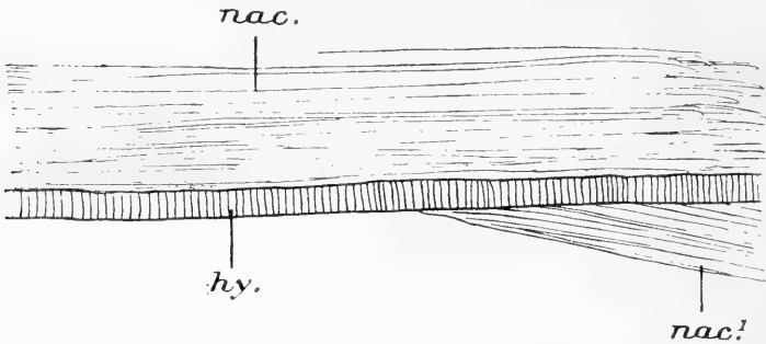
The inner limit of the adductor scar, in the same shell as that shown in text-fig. 36. hy. , hypostracum; nac. , nacre external to same; nac.? , nacre internal to same. \times 40 .
