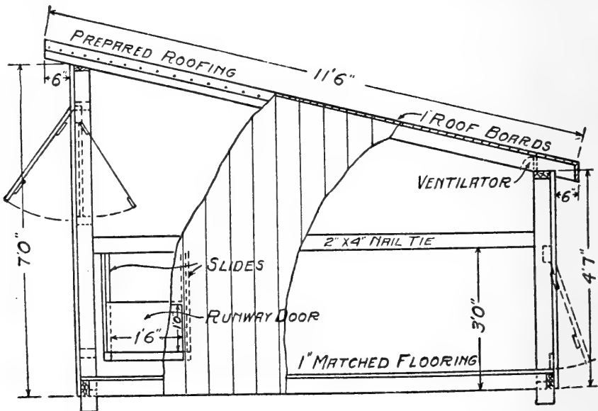
Figure 253.—End view Purdue Brooder Colony House. Reproduced from Extension Bulletin 52, Purdue University.
