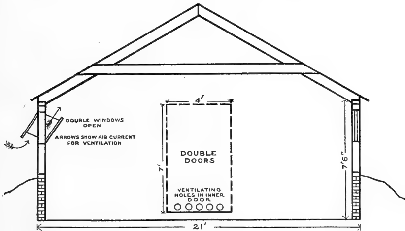
FIG. 2—SECTIONAL VIEW SHOWING VENTILATING SYSTEM
