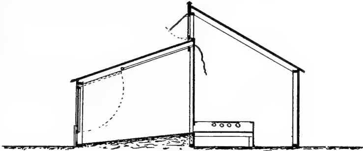
FIG. 2.—SECTION OF BROODER HOUSE SHOWING CANVAS SHELTER IN SOUTH FRONT AND WINDOW NEAR THE PEAK OF THE BROODING SECTION OF THE HOUSE
