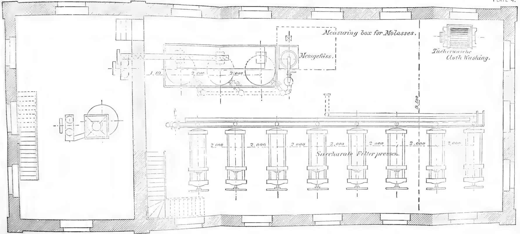
STEFFEN'S PROCESS. PLAN OF SECOND FLOOR.
