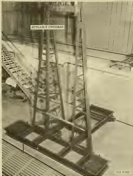
Figure 4 – Straight Tower (Located at East End of the Basin)
