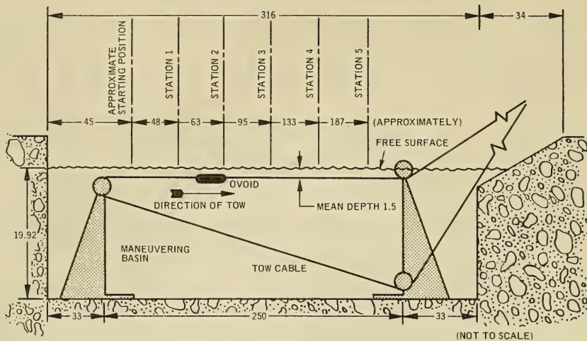
Figure 8 – Tow Cable and Model Location
