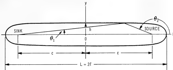
Offsets of a 7 to 1 Rankine Ovoid
