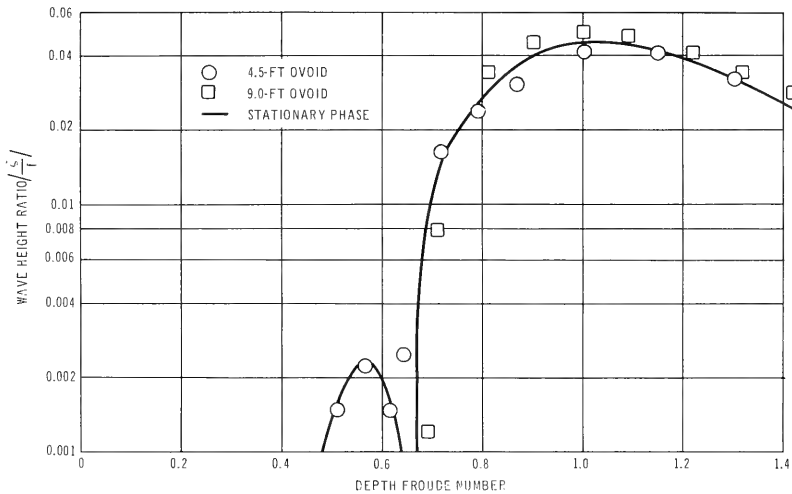
Figure 21 – Dimensionless Wave Heights of First Centerline Wave Crests as Functions of Depth Froude Number – Experimental and Stationary-Phase Data
