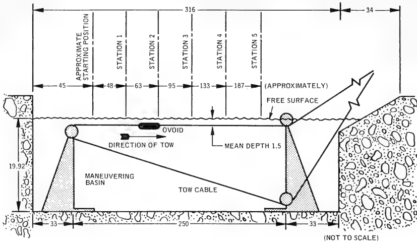
Figure 8 – Tow Cable and Model Location
