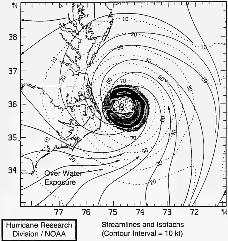
Figure 6. Surface wind analysis for Hurricane Emily 0200 hr UTC 1 September 1993
