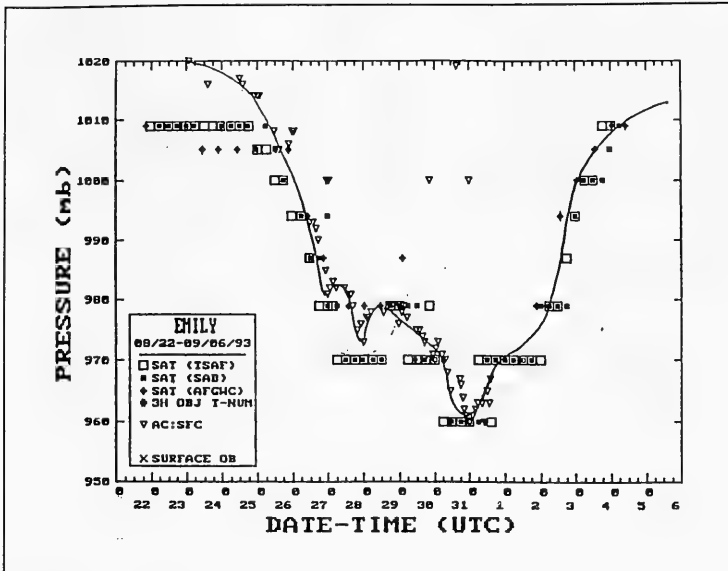
Figure 2. Best track minimum central pressure curve for Hurricane Emily
