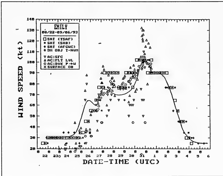
Figure 3. Best track 1-min sustained wind speed curve for Hurricane Emily
