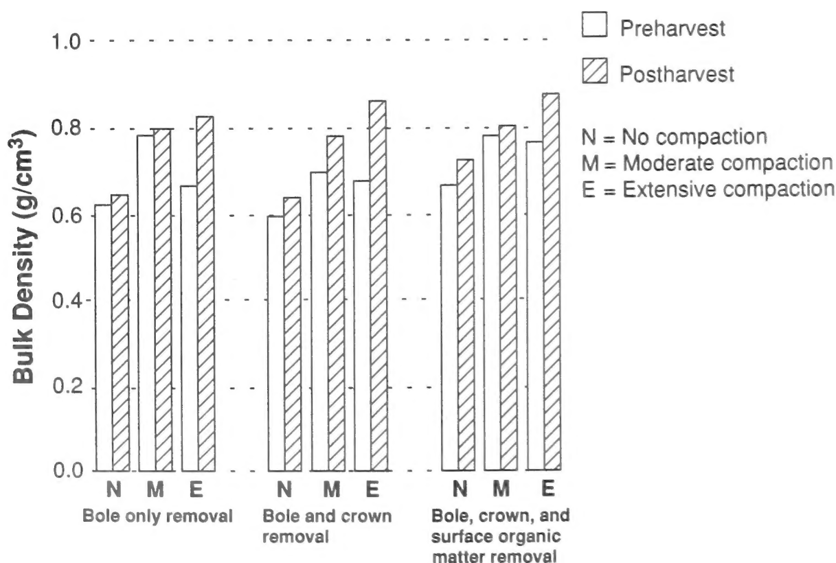
Figure 1—The effects of timber harvesting and site preparation on soil bulk density, averaged for three soil depths.
