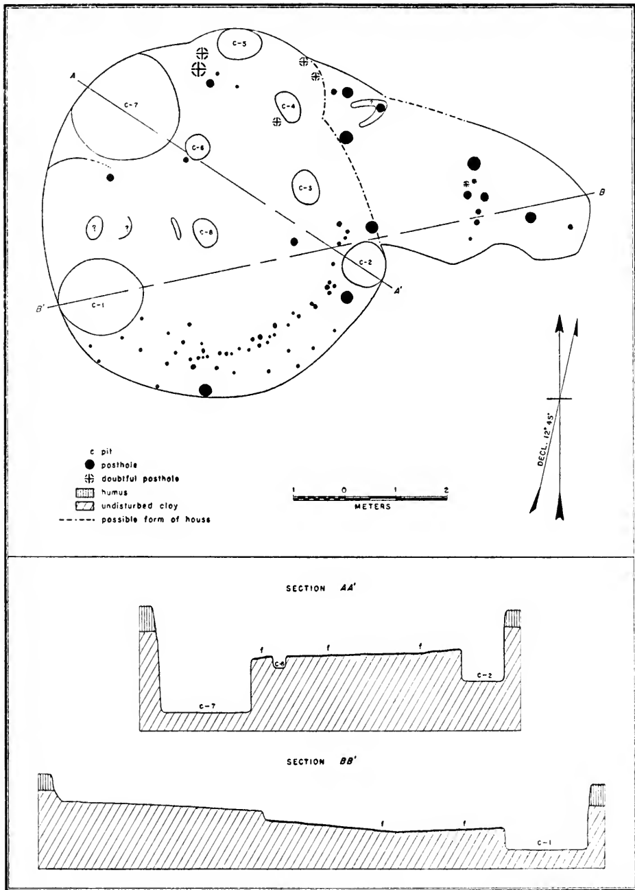
MAP 22. PLAN AND SECTIONS OF PIT HOUSE P
