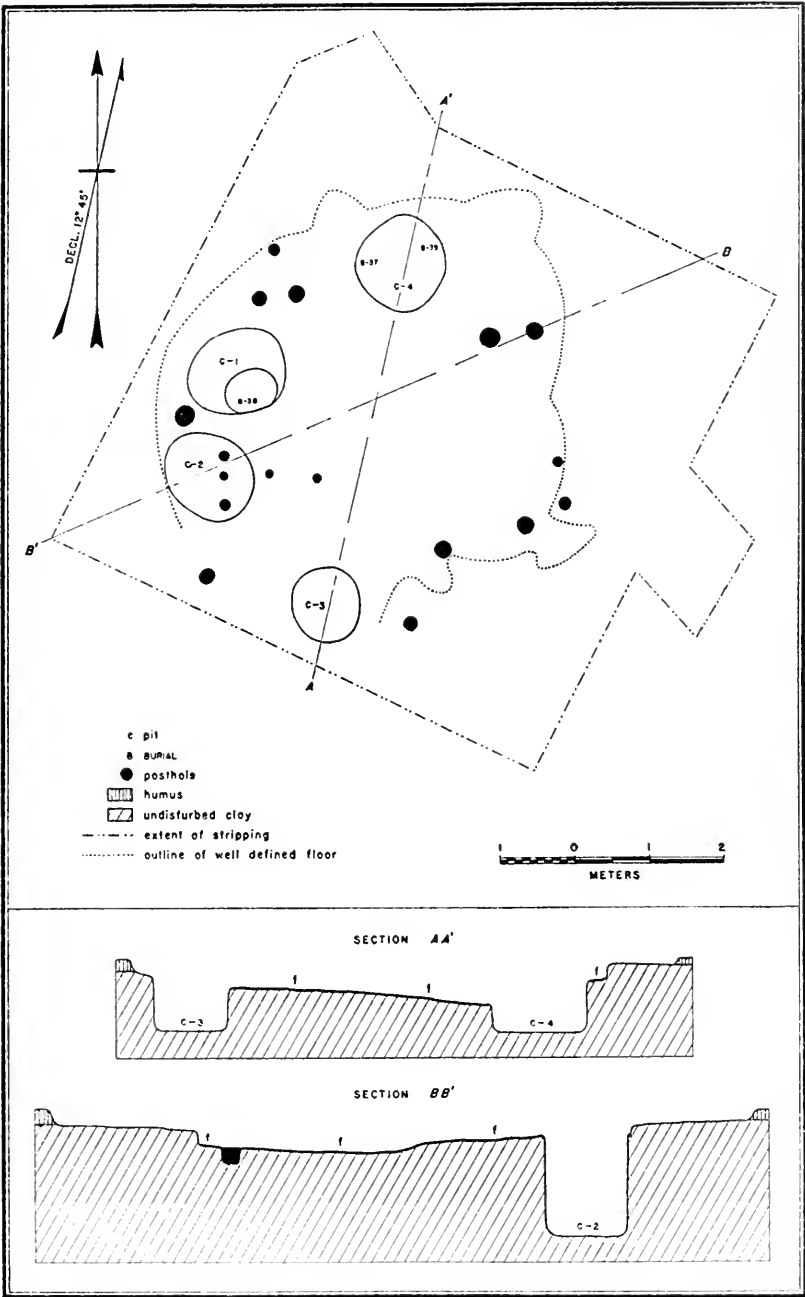
MAP 23. PLAN AND SECTIONS OF SURFACE HOUSE 2
