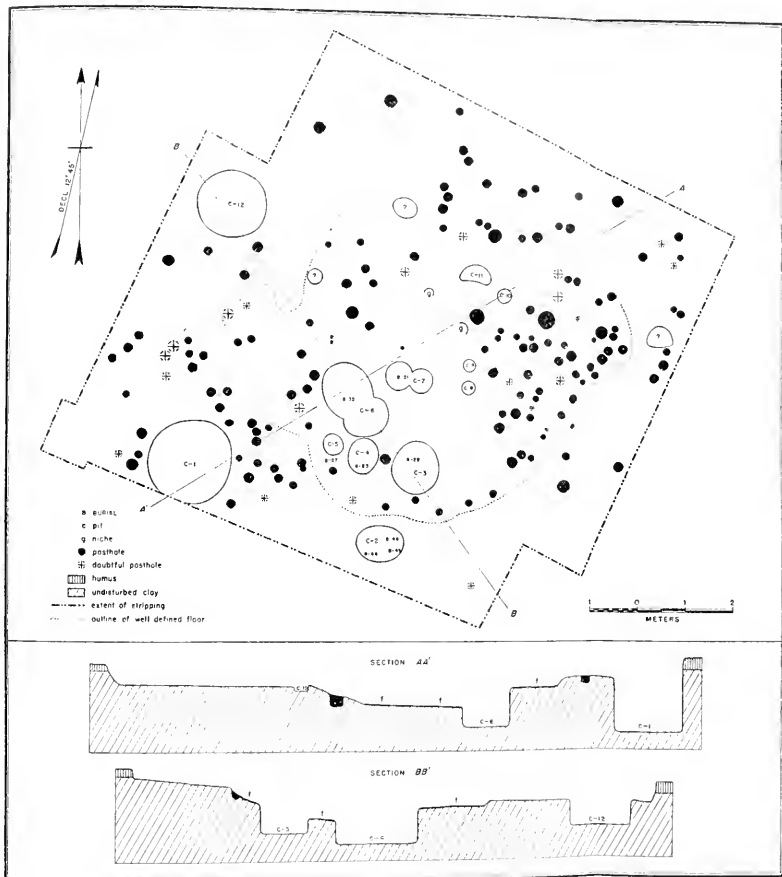
MAP 18. PLAN AND SECTIONS OF SURFACE HOUSE 3 (FORMERLY CALLED K)
