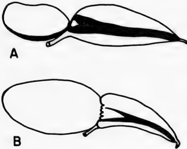
FIG. 111. Types of serrasalmid swim bladders. A, The general type, with the posterior chamber most prominent. B, The special type, with the anterior chamber most prominent; this type is to be seen in the genera Serrasalmus and Piaractus .
