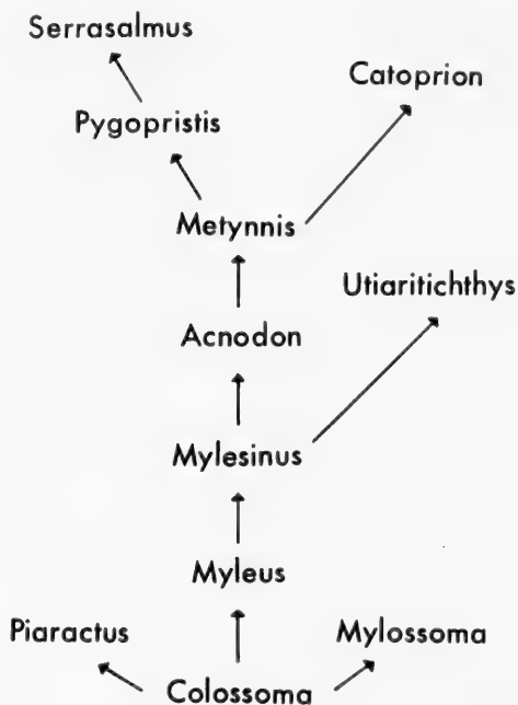
FIG. 119. Schema showing inter-relationships of the genera of the Serrasalminae, based upon internal morphology.
