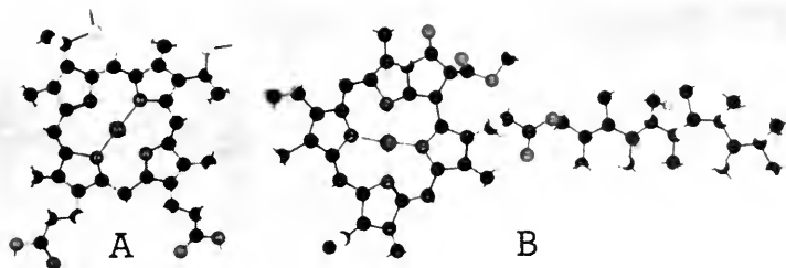
FIG. 11. A. Portion of the prosthetic group of Cytochrome c. B. Chlorophyll A. The large central ball in the porphyrin ring represents iron in Cytochrome and magnesium in Chlorophyll.
