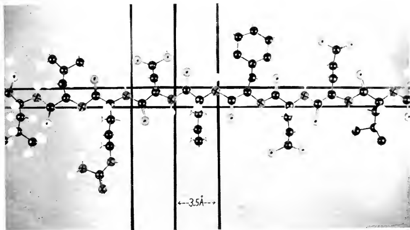
FIG. 4. Model photograph of a portion of a protein chain, made to scale using known atomic radii and bond angles. Black balls indicate carbon atoms; dark grey balls marked X indicate nitrogen atoms; light grey balls marked with a dot indicate oxygens; small white balls, hydrogen atoms.
