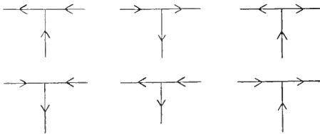
FIG. 4. Six possible combinations in direction of flow in two connecting strands.
