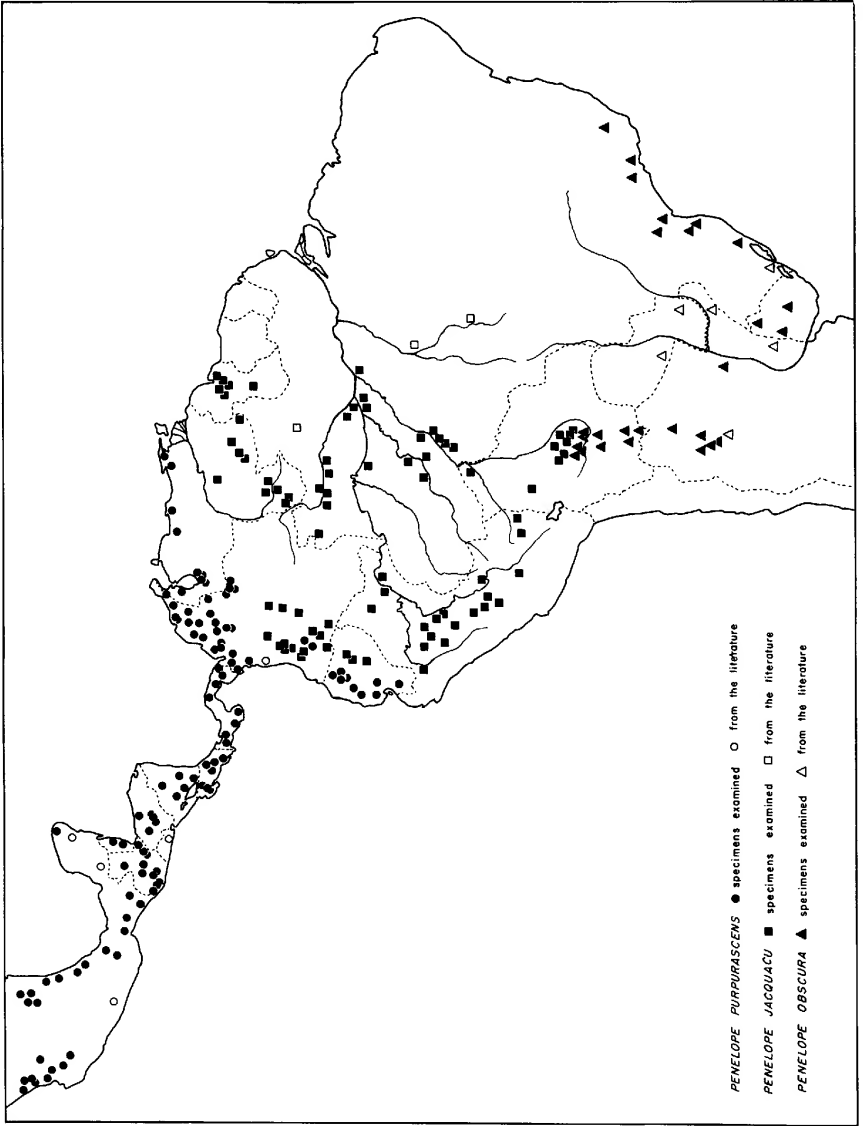
FIG. 1. Distribution of Penelope purpurascens , Penelope jacquacu , and Penelope obscura .
