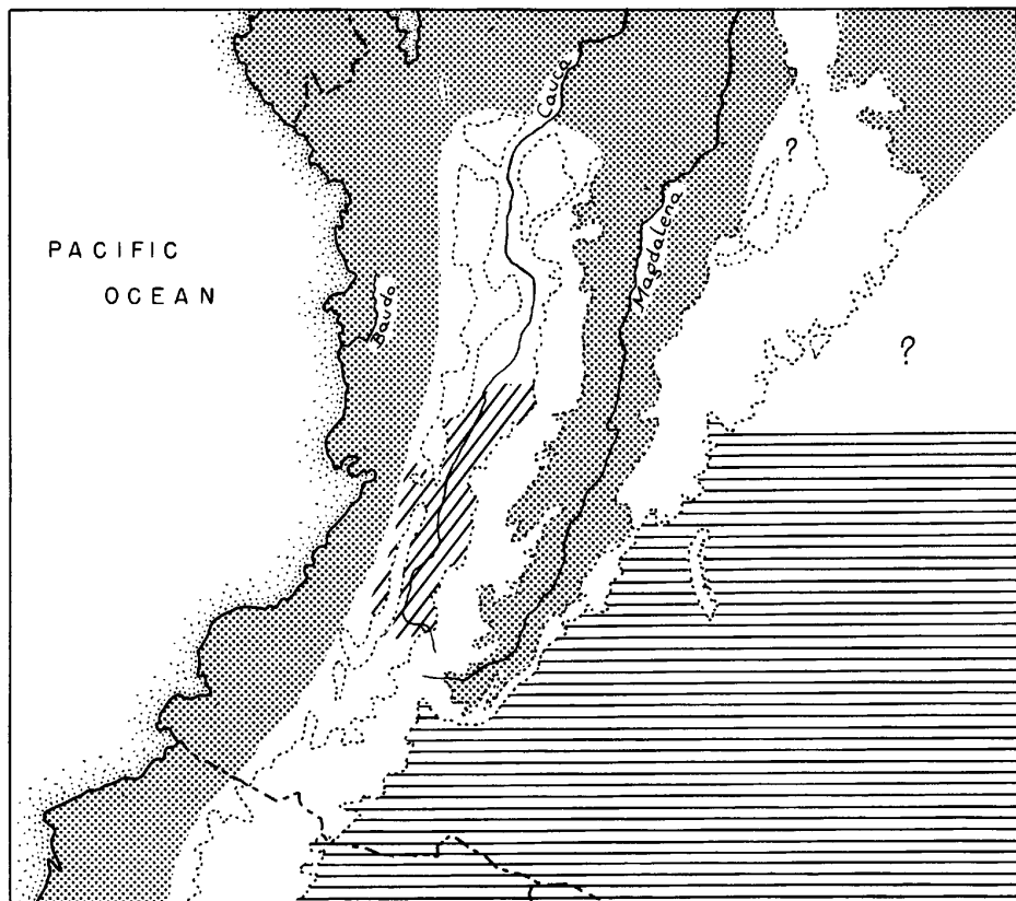
FIG. 2. Distribution of Penelope purpurascens and Penelope jacquaçu in central and western Colombia and neighboring Panama and Ecuador. The stippled area indicates the range of P. purpurascens ; the diagonal lines show the range of P. jacquaçu perspicax ; and the horizontal lines, that of nominate jacquaçu . The approximate contour of 2000 meters is shown by dotted lines.
