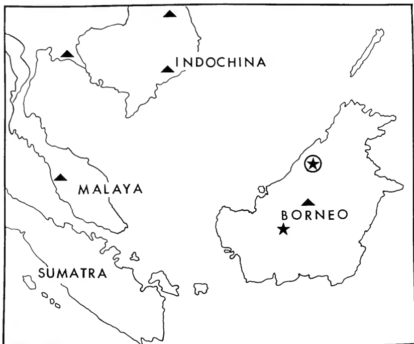
FIG. 4. Triangles show localities of Sphenomorphus stellatus ; stars show localities of Sphenomorphus hallieri ; circle shows type locality of Sphenomorphus maculicollus .
