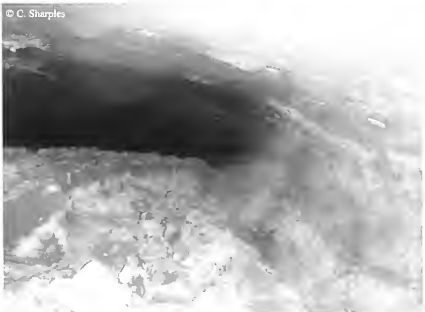
Plate 3. Dry passage in Conference Concourse in the vicinity of Plates 1-2, July 2011. The passage is low (<1 m) due to infilling by sediment deposited by an ancient stream. The whitish coloration is precipitated salts (potentially calcite, aragonite and/or gypsum).
