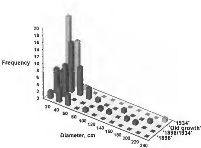
Figure 6. Diameter distribution of stags in the four plots at the Warra 'Bird Track'. Although plots '1934' and 'Old growth' had almost the same number of stags (34 vs. 33), those for '1934' were mostly concentrated in the two lowest diameter classes ( D \leq 40 cm), whereas 'Old growth' had more stags in the higher diameter classes. Like plot '1934', '1898/1934' also had the majority of its stags in the D \leq 40 cm classes, but it also had four stags with diameters 1.0 m or greater. Plot '1898' had few stags.
