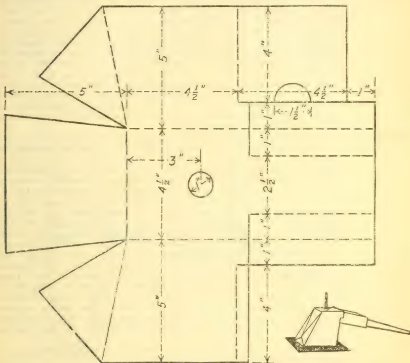
FIG. 11.—Asbestos shield.
