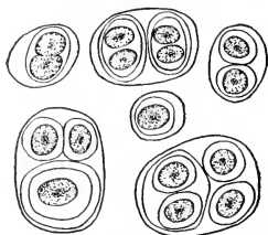
FIG. 4.— Gloeothecce : a single plant in the center, showing the protoplast surrounded by the swollen wall and a layer of mucilage; the other figures show various stages of cell-multiplication, the cells being embedded in the gelatinous matrix produced by their walls.
