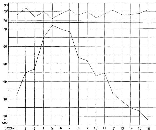
FIG. 603. — Grand curve of growth (solid line): the first day of the observation was evidently after fairly rapid growth had begun; it attained a maximum on the fifth day, with an increment of 72 mm.; thence the rate falls off rapidly, and on the sixteenth day is only 18 mm.; growth rate magnified 10 times. The temperature curve (broken line) for the same days runs between 71 and 77° F. — From data by SPOEHR.
