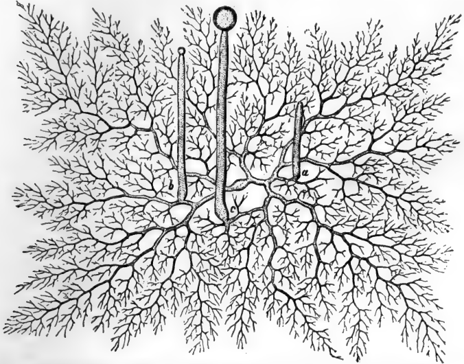
FIG. 125.—Diagram of Mucor , showing the profusely branching mycelium and three sporophores, sporangia forming on b and c .—After ZOPF.
