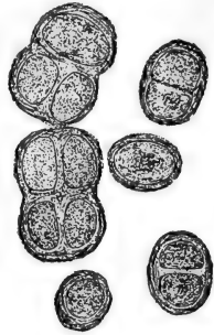
FIG. 92.— Glæocapsa : showing single cells, and small groups that have been formed by division and are held together by the enveloping mucilage.
