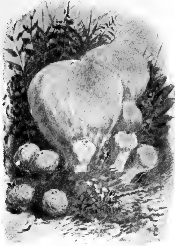
FIG. 152.—Puffballs.—After GIBSON.
