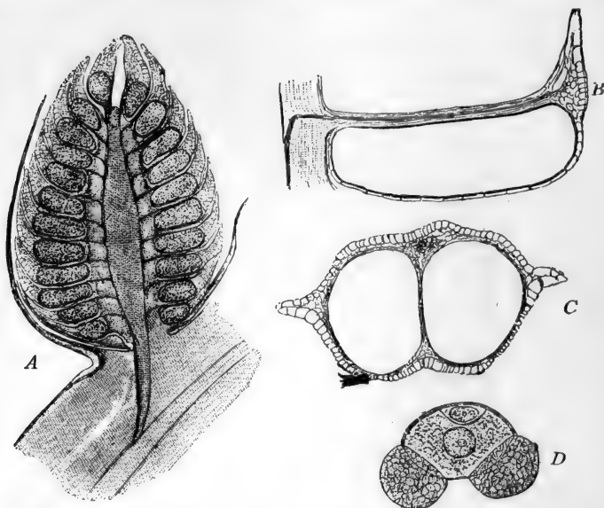
FIG. 203.—Staminate cone of pine: A , section of cone, showing sporophylls (stamens) bearing sporangia (pollen sacs); B , longitudinal section of stamen, through one pollen sac; C , cross-section of stamen, showing both pollen sacs; D , the winged pollen grain.—After STRASBURGER.
