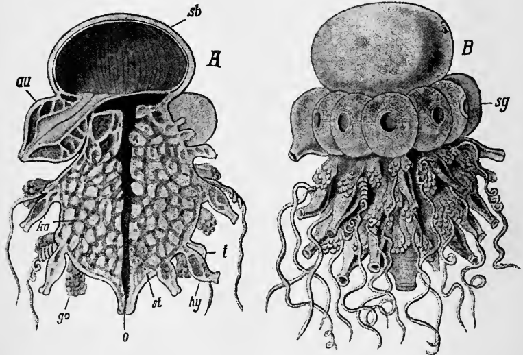
FIG. 84.— Stephalia corona , after Haeckel. A , Halved longitudinally. B , From life. sb , Swim-bladder; au , aurophore; sg , swimming-bells; ka , canal system of the stem (chief stomach, st ); go , gonophore clusters; o , aperture (mouth) of the peduncle (chief gastric tube, st ); hy , gastric tubes (siphons); t , tentacles.
