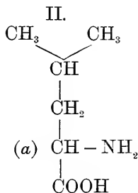
\alpha -Amido-isobutylacetic acid.
