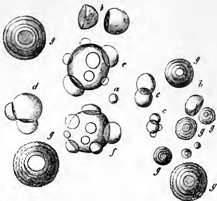
FIG. 15. LEUCINE IN THE FORM WHICH IT USUALLY ASSUMES WHEN SEPARATED FROM THE PRODUCTS OF DIGESTION BY TRYPSIN.
