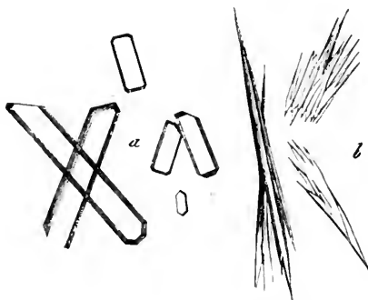
FIG. 22. CRYSTALS OF TAURINE. (a) pure, (b) impure.
