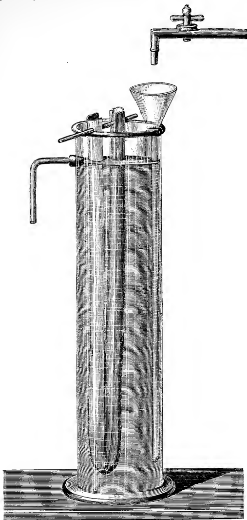
FIG. 7. KÜHNE'S ARRANGEMENT FOR DIALYSING IN A CONTINUOUS STREAM OF WATER.
