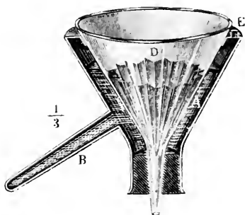
FIG. 23. A HOT-WATER FUNNEL.
