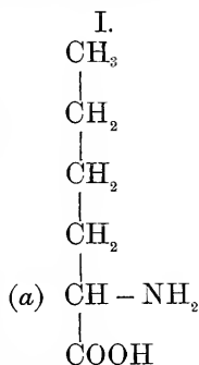
\alpha -Amido-normal caproic acid.
