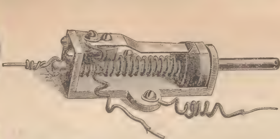
CIRCUIT CLOSER FOR MECHANICAL DOOR PULL
