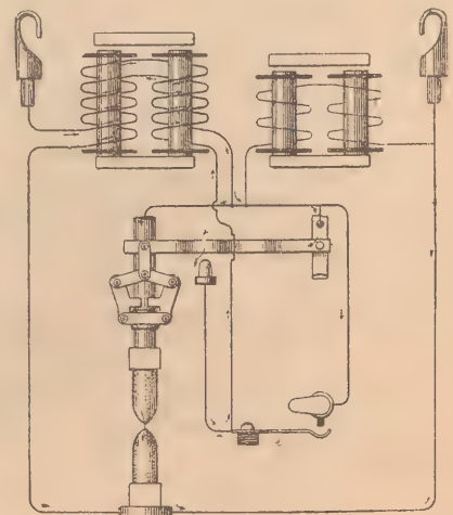
NO. 423,638. CUT-OUT FOR ELECTRIC LAMPS.
