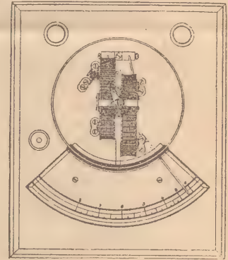
NO. 423,600. AMPERE METER.
