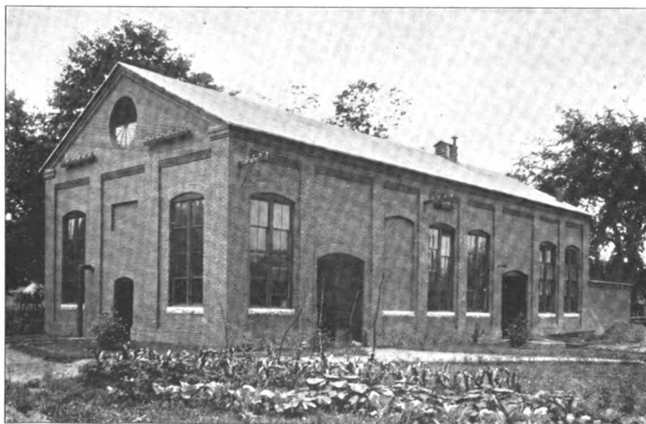
EXTERIOR OF THE GAS-POWER PLANT OF THE CITIZENS' ELECTRIC COMPANY. THE ABSENCE OF ANY SMOKESTACK IS A CONSPICUOUS FEATURE
