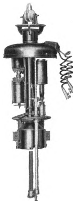
FIG. 2.—MECHANISM OF A SERIES LUMINOUS ARC LAMP
