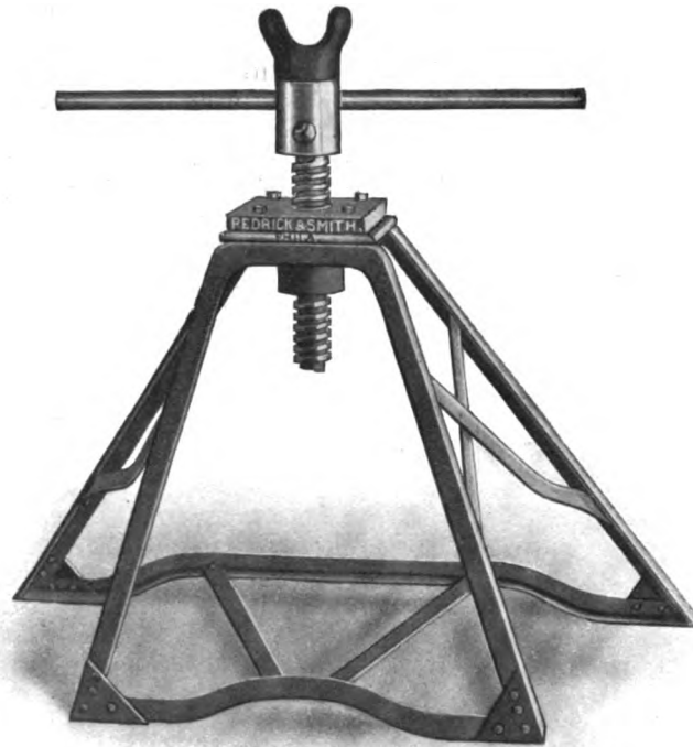
A SCREW CAPSTAN CABLE JACK BUILT BY PEDRICK & SMITH, GERMANTOWN, PHILADELPHIA
