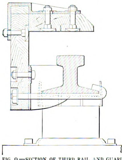
FIG. 9.—SECTION OF THIRD RAIL AND GUARD
