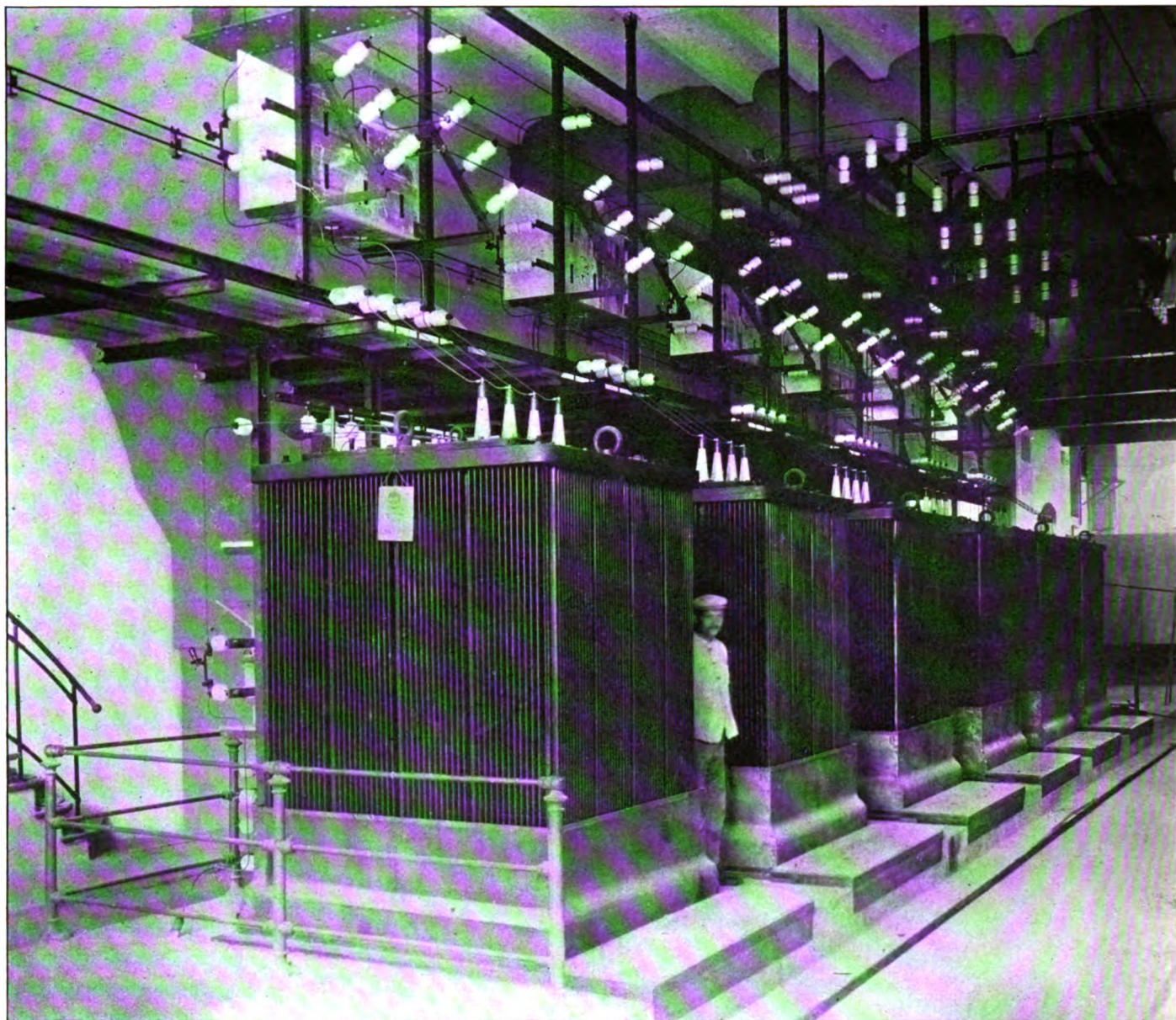
FIG. 21.—TRANSFORMERS IN THE GLOMMEN RIVER POWER PLANT. CURRENT IS GENERATED AT 5000 VOLTS AND RAISED TO 20,000 VOLTS
