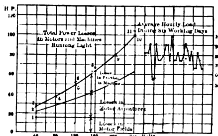
FIG. 6.—POWER LOSSES AND AVERAGE CONSUMPTION OF FORTY-SIX MACHINES WITH MOTORS OF AN AGGREGATE RATED HORSE-POWER OF 500
