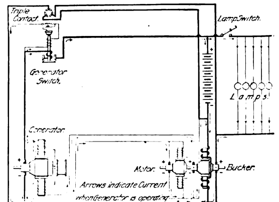
FIG. 11.—DIAGRAM SHOWING CONNECTIONS OF THE BLISS SYSTEM
