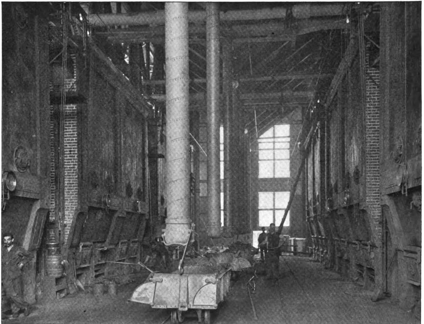
FIG. 6.—THE BOILER ROOM IN THE WESTVILLE POWER STATION. TWELVE WATER-TUBE BOILERS BUILT BY THE STIRLING CONSOLIDATED BOILER COMPANY, NEW YORK, AND PROVIDED WITH SUPERHEATERS, GENERATE STEAM AT 175 POUNDS
