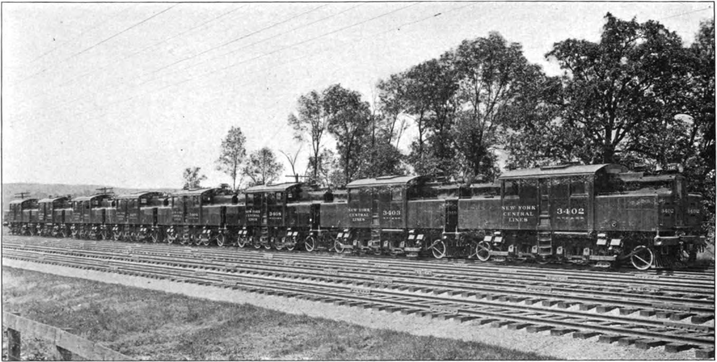
EIGHT ELECTRIC LOCOMOTIVES BUILT JOINTLY BY THE GENERAL ELECTRIC COMPANY AND THE AMERICAN LOCOMOTIVE COMPANY, OF SCHENECTADY, N. Y., FOR THE NEW YORK CENTRAL & HUDSON RIVER RAILROAD
