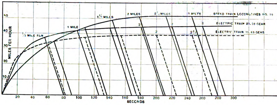
FIG. 8.—TIME SPEED CURVE OF A STEAM TRAIN WEIGHING 171.9 TONS, DISREGARDING A SMALL LIVE LOAD; AND TIME SPEED CURVES OF PROPOSED ELECTRIC TRAINS, WEIGHING 121 TONS WITH STARTING LOAD. ALL TRAINS HAD THREE CARS
