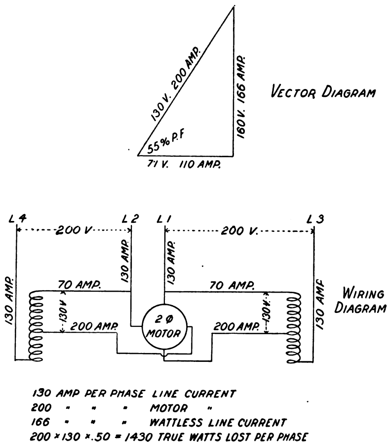
FIG. 1.—WIRING DIAGRAM OF TWO-PHASE MOTOR AND POWER CIRCUIT
