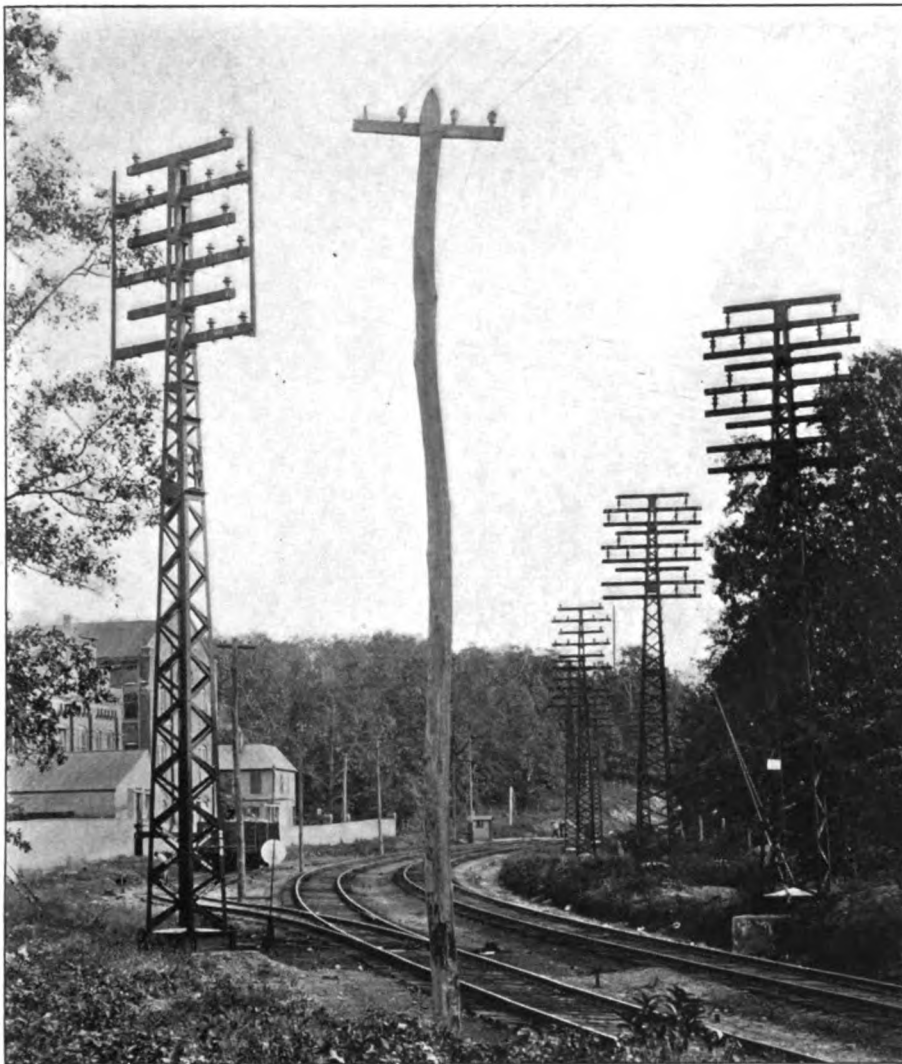
FIG. 1.—THE TRANSMISSION LINE OF THE LONG ISLAND RAILROAD CROSSING A TRACK. THE CABLE RETAINERS ARE SHOWN ON THE POLE AT THE LEFT
