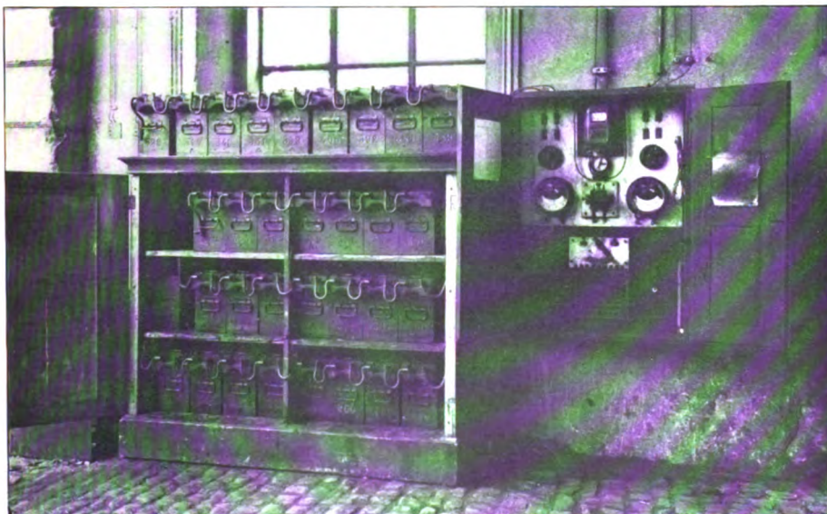
FIG. 2.—INTERIOR OF CAR LIGHTING STORAGE BATTERY CHARGING STATION AT PRAGUE
