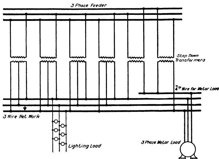
FIG. 3.—THREE-WIRE SECONDARY NETWORK, WITH FOURTH WIRE FOR POWER
