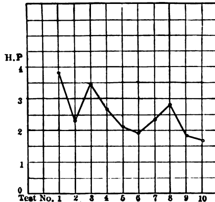
FIG. 5.—HORSE-POWER REQUIRED PER POUND OF METAL REMOVED
