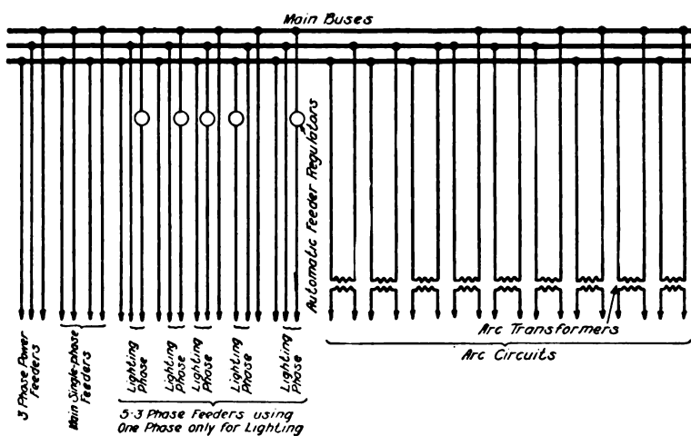
FIG. 2.—THE SYSTEM OF FEEDER CONNECTIONS USED IN SCHENECTADY, N. Y.
