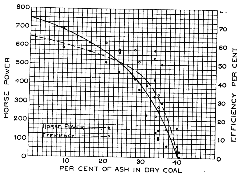
FIG. 2.—INFLUENCE OF ASH IN COAL ON CAPACITY AND EFFICIENCY
