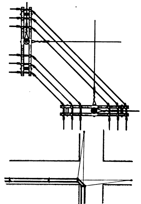
FIG. 8.—TWO-POLE METHOD OF TURNING A CORNER
