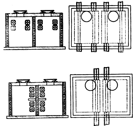
FIG. 6.—SHOWING GENERAL CONSTRUCTION OF MANHOLES AND THE GROUPING OF DUCTS
