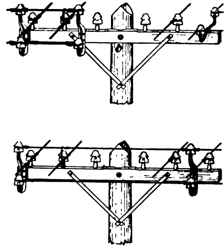
FIG. 17.—BRANCH LINE TAPS
