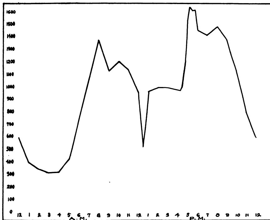
FIG. 4.—CURRENT GENERATED DECEMBER 15, 1905
