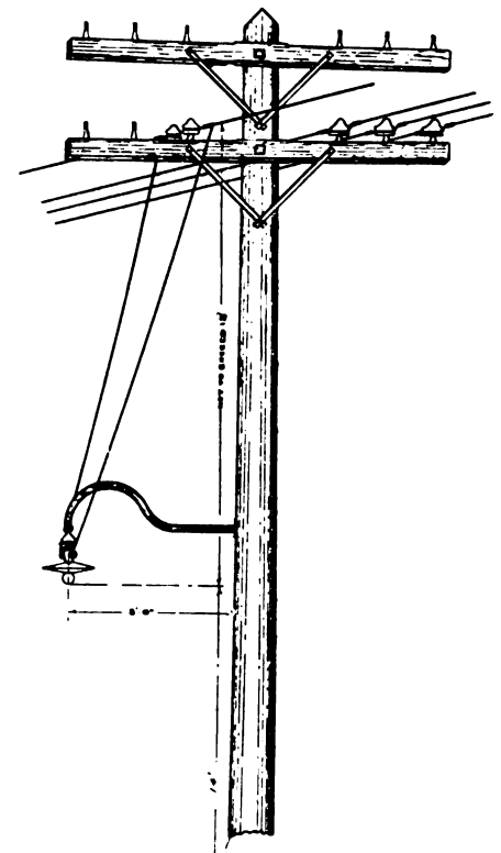
FIG. 20.—INCANDESCENT LAMP SUSPENSION WITH SEPARATE CONDUCTOR LOOP
