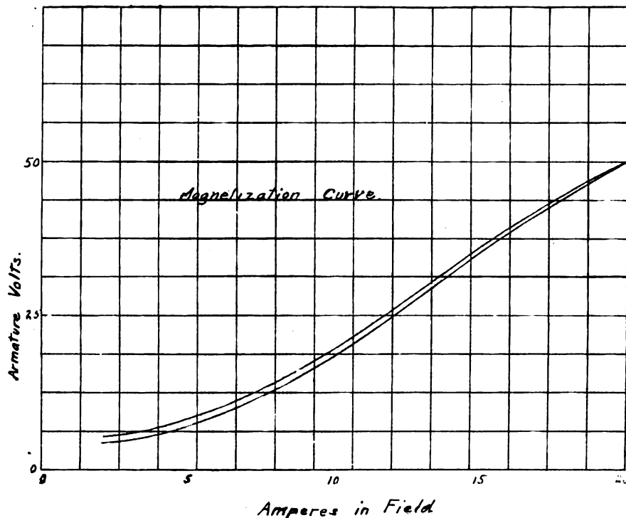
FIG. 5.—MAGNETIZATION CURVE OF A SINGLE-PHASE MOTOR
