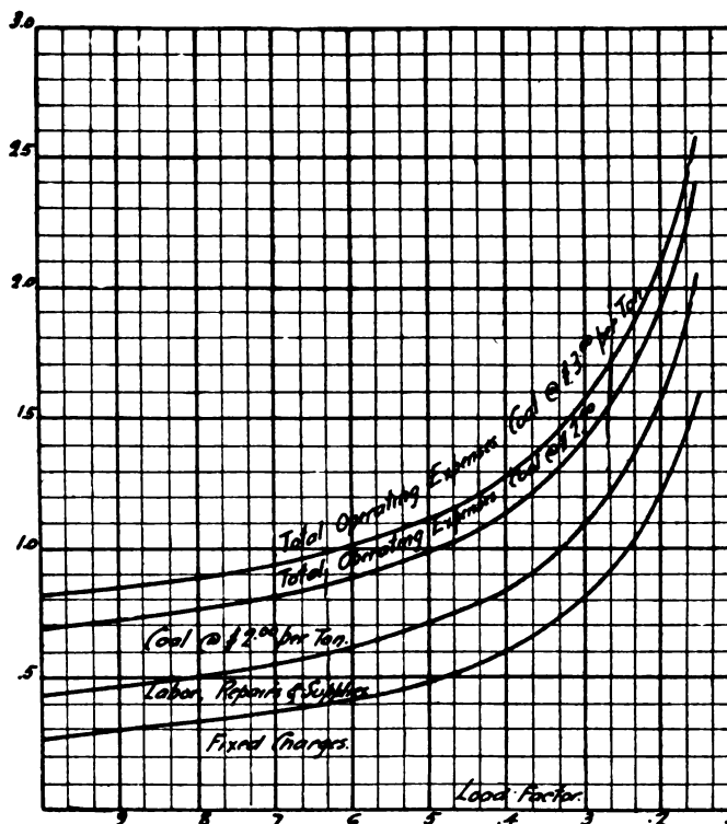
FIG. 5.—OPERATING EXPENSES OF AN 1800-KW. CONDENSING STEAM PLANT WITH A 1500-KW. PEAK
