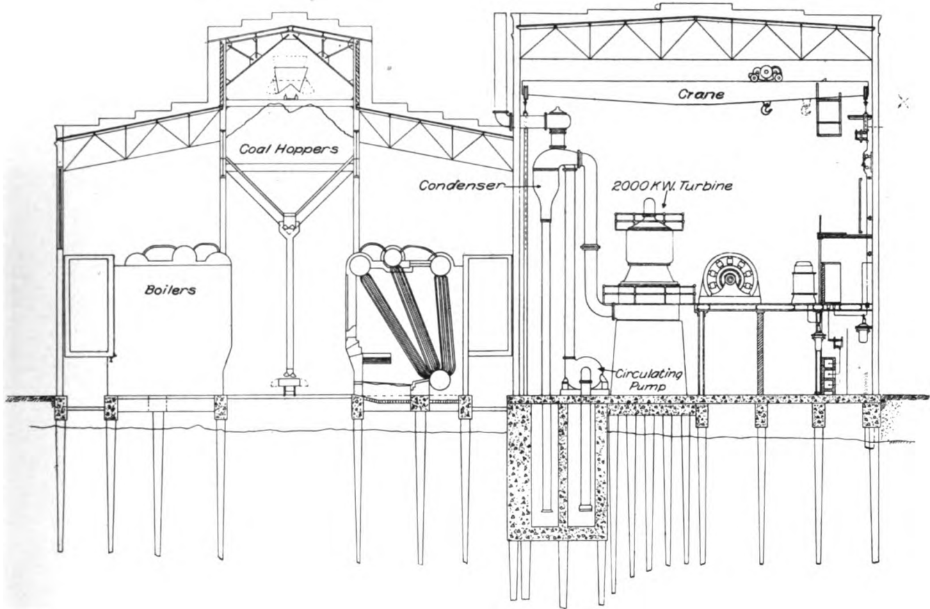
FIG. 7.—TRANSVERSE SECTION OF THE POWER HOUSE AT WESTVILLE, N. J.
