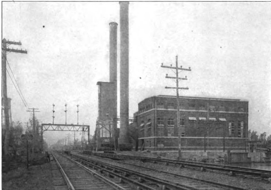
FIG. 1.—THE POWER HOUSE OF THE WEST JERSEY & SEASHORE RAILROAD AT WESTVILLE, N. J.
