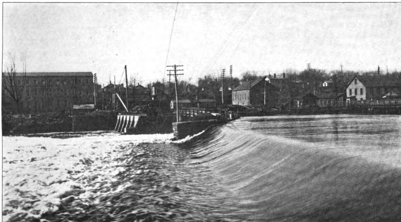
FIG. 1.—VIEW OF THE UPPER DAM WHILE THE CENTRAL PLANT OF THE JANESVILLE ELECTRIC COMPANY WAS BEING CONSTRUCTED. THIS IS ONE OF THREE PLANTS OWNED BY THE COMPANY, TWO BEING USED FOR NORMAL SERVICE AND ONE FOR PEAK LOADS
