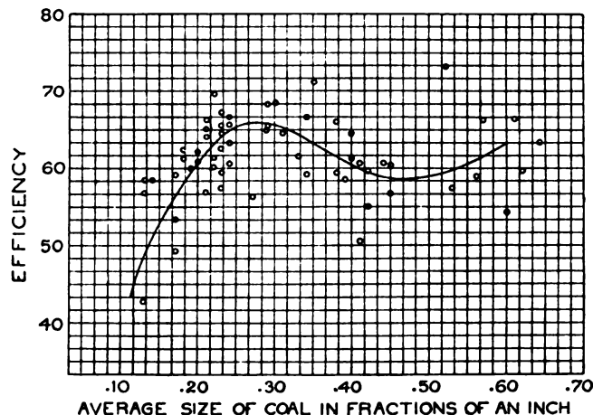
FIG. 4.—EFFECT ON EFFICIENCY OF COAL OF DIFFERENT SIZES
