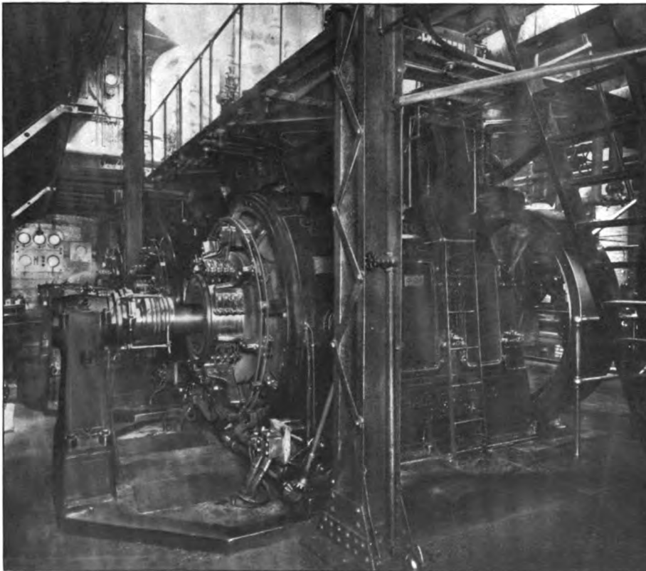
WESTINGHOUSE THREE-WIRE, DIRECT-CURRENT GENERATORS FURNISH CURRENT FOR THE OLIVER ESTATE
