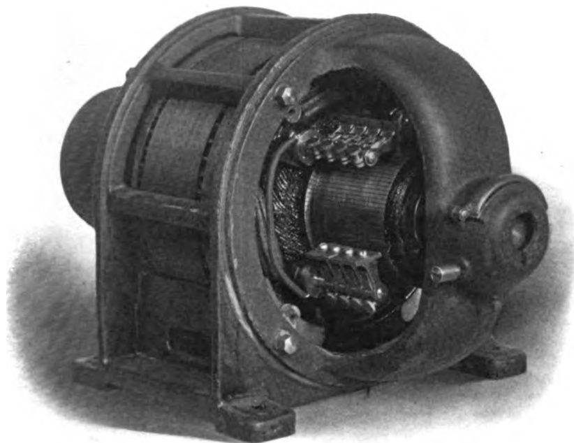
A SINGLE-PHASE REPULSION INDUCTION MOTOR BUILT BY THE STANLEY-G. L. ELECTRIC MANUFACTURING COMPANY, PITTSFIELD, MASS.
