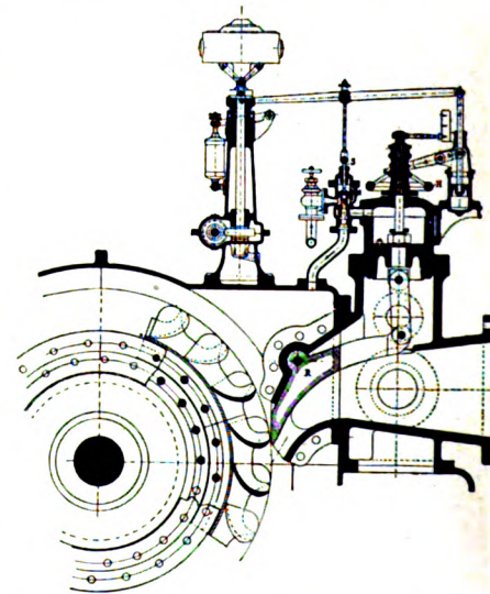
FIG. 18.—SECTION OF A WHEEL AND GOVERNOR IN THE INNSBRUCK PLANT
