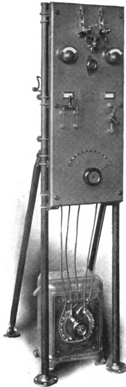
FIG. 1.—NEW MERCURY-ARC RECTIFIER OUTFIT MADE BY THE GENERAL ELECTRIC COMPANY, SCHENECTADY, N. Y.
