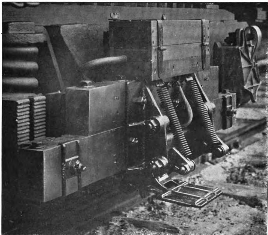
FIG. 4.—INNER POSITION OF THE ADJUSTABLE THIRD-RAIL SHOE
