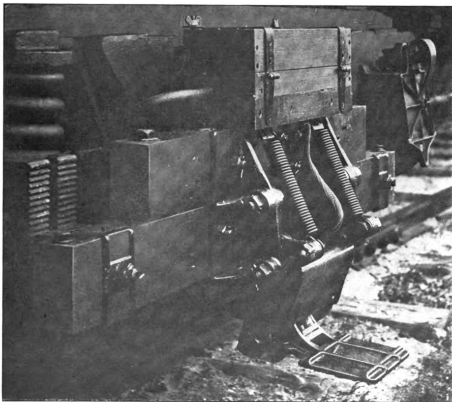
FIG. 5.—OUTER POSITION OF THE ADJUSTABLE THIRD-RAIL SHOE
