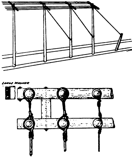
FIG. 6.—METHOD OF DEAD-ENDING A LINE
