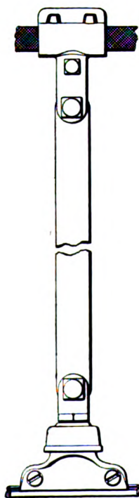
FIG. 5.—SPREADER MADE OF FLAT STEEL STRIP
