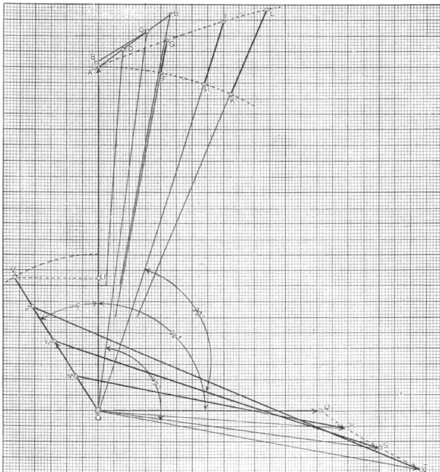
FIG. 4.—VECTOR DIAGRAM FOR 85 PER CENT. POWER FACTOR
