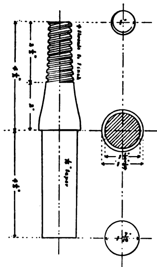
FIG. 15.—STANDARD LOCUST PIN
