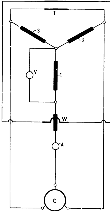
FIG. 6.—CONNECTIONS FOR A CORE LOSS TEST
