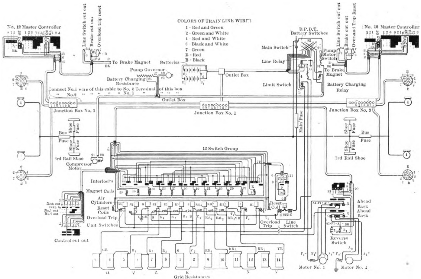
FIG. 10.—WIRING DIAGRAM OF A MOTOR CAR
