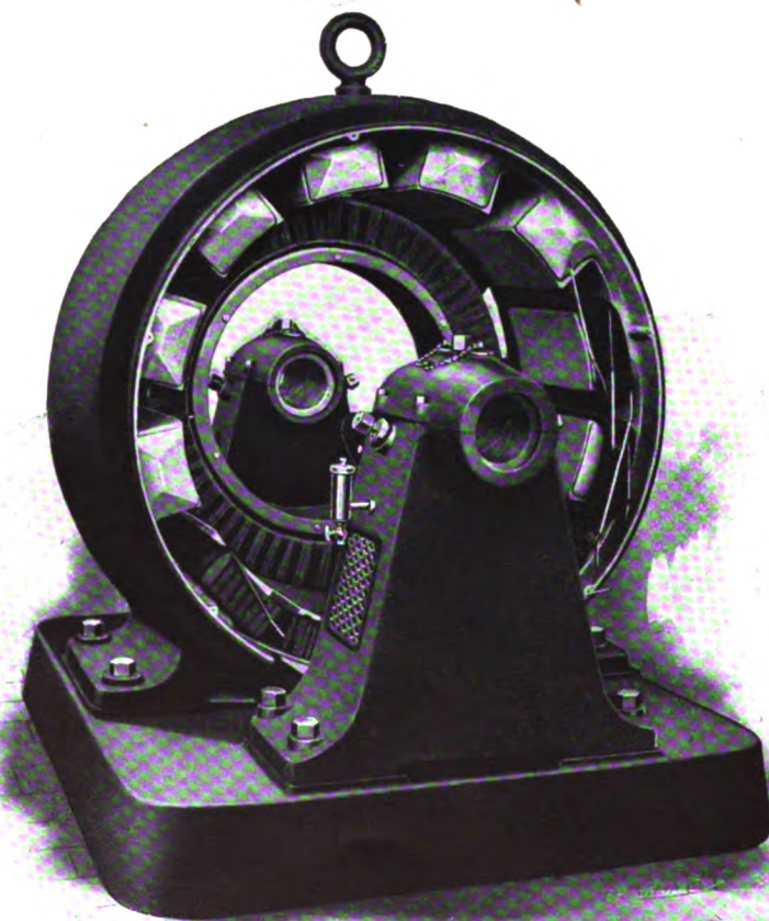
FIGS. 1 AND 2.—INDUCTOR AND ARMATURE OF AN INDUCTOR ALTERNATOR BUILT BY THE WARREN ELECTRIC MANUFACTURING COMPANY, SANDUSKY, OHIO.
