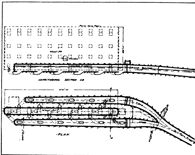
WHEEL PIT AND BRANCH TAILRACE TUNNELS
