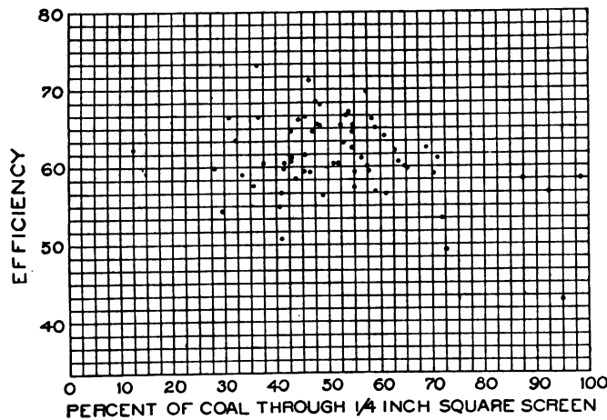
FIG. 8.—EFFECT OF SCREENED COAL ON EFFICIENCY
