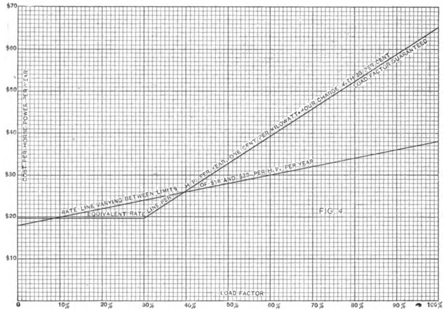
FIG. 4.—SUGGESTED PLAN OF CHARGING FOR ELECTRIC POWER
