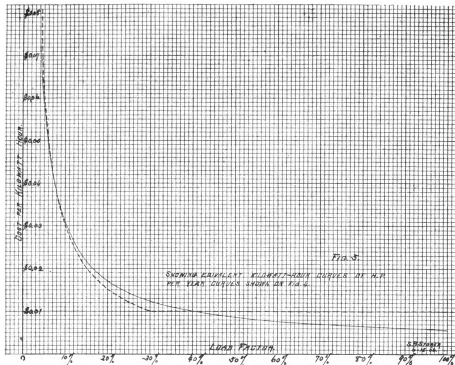
FIG. 5.—EQUIVALENT KILOWATT-HOUR CURVES OF HORSE-POWER PER YEAR CURVES SHOWN IN FIG. 4
