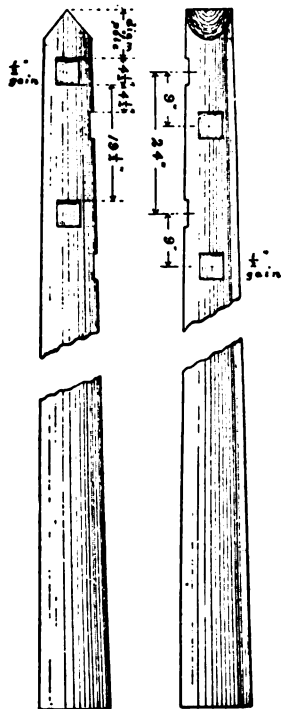
FIG. 1.—POLE FRAMING
