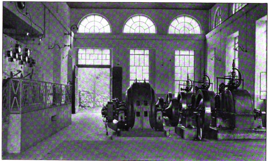
FIG. 2.—INTERIOR OF THE HYDRO-ELECTRIC PLANT ON THE MAROBBIA RIVER IN SWITZERLAND. CURRENT IS GENERATED BY THREE 490-KW. MACHINES AT 5350 VOLTS
