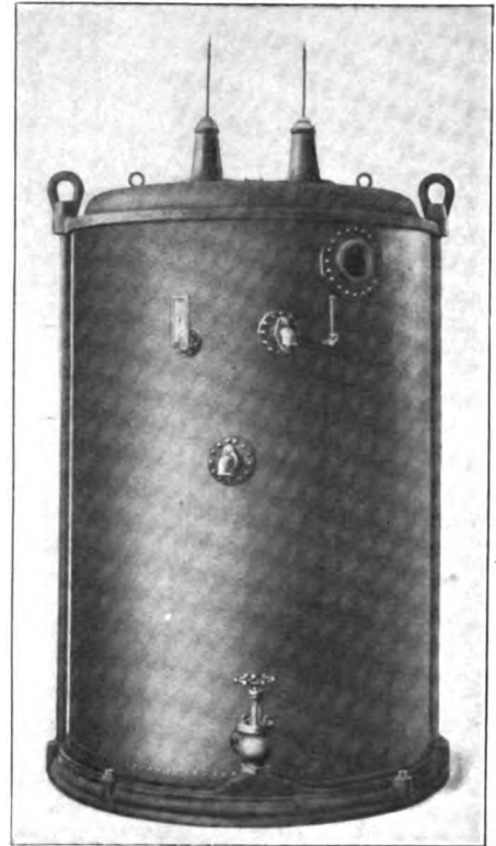
A 500-KW., 405-2000-VOLT, OIL-FILLED, WATER-COOLED TRANSFORMER, BUILT BY THE ALLIS-CHALMERS COMPANY, MILWAUKEE, WIS.
