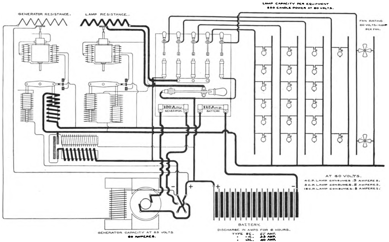
FIG. 12.—WIRING DIAGRAM OF THE MCELROY AUTOMATIC CAR LIGHTING SYSTEM OF THE CONSOLIDATED CAR HEATING COMPANY, NEW YORK
