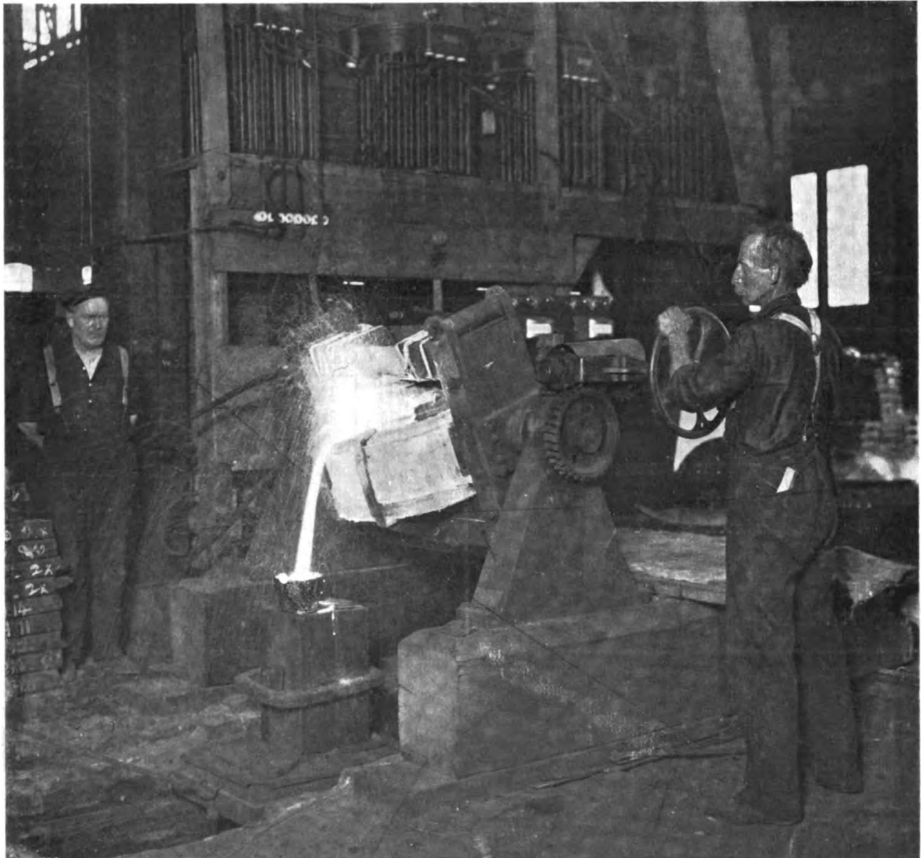
AN ELECTRIC STEEL FURNACE OPERATING ON A CENTRAL STATION CIRCUIT. SEE PAGE 353
