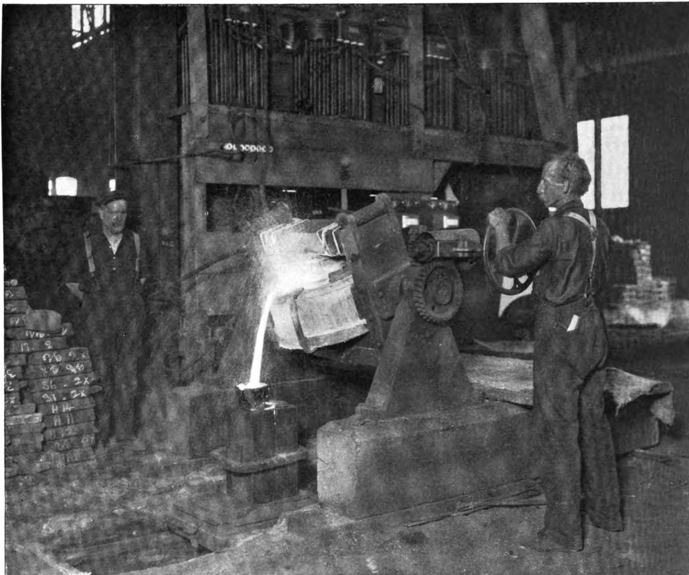
FIG. 3.—POURING MOLTEN STEEL FROM THE ELECTRIC FURNACE SHOWN IN FIG. 1.
