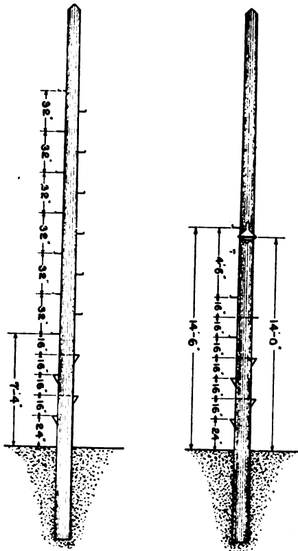
FIG. 3.—LOCATION OF POLE STEPS
