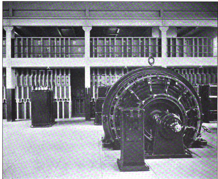
FIG. 12.—AN INTERIOR VIEW OF PART OF THE SUB-STATION AT WOODHAVEN JUNCTION LOOKING TOWARD THE HIGH-TENSION GALLERY
