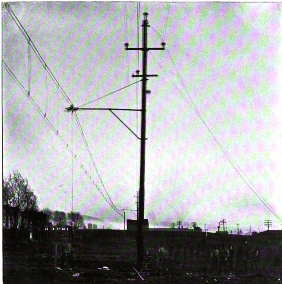
FIG. 4.—APPEARANCE OF THE EXPERIMENTAL LINE UNDER A DOWNWARD STRAIN OF 2000 POUNDS ON THE END OF THE BRACKET
