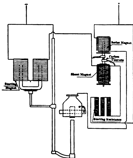
FIG. 3.—CONNECTIONS OF THE LAMP MECHANISM
