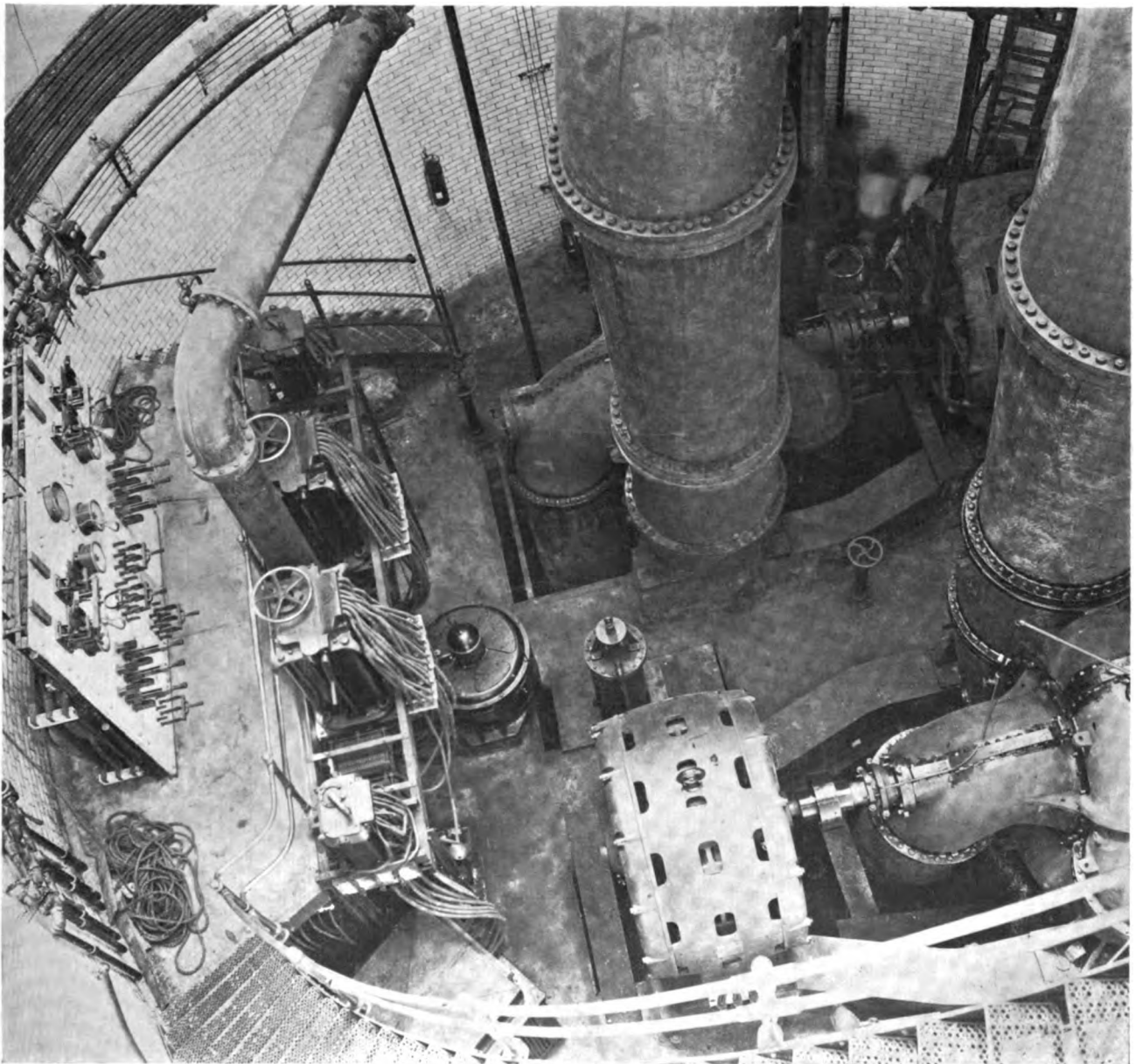
THE MOTOR-DRIVEN DRY DOCK PUMPING PLANT AT THE BOSTON NAVY YARD. SEE PAGE 37
