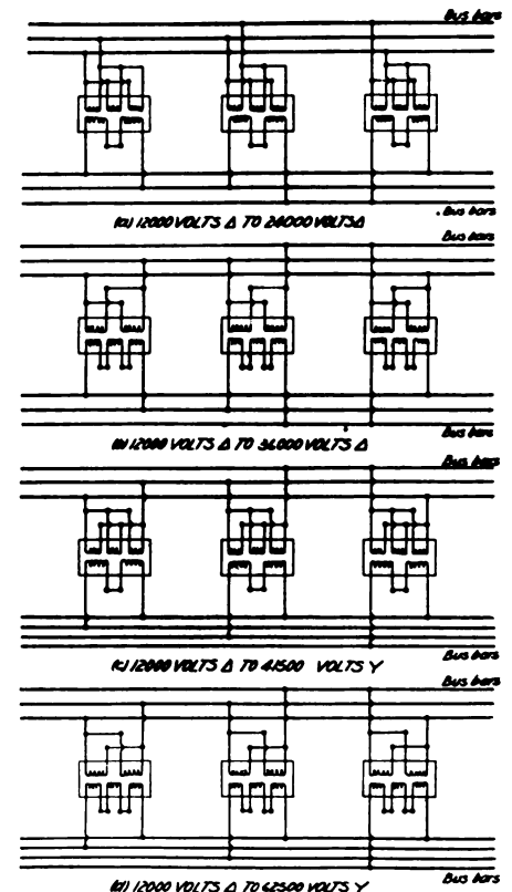
FIG. 10.—DIAGRAM OF WINDINGS OF THE 1250-KW. TRANSFORMERS
