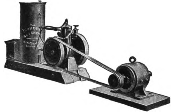
A SMALL GAS-ENGINE LIGHTING UNIT BUILT BY THE R. M. CORNWELL COMPANY, OF SYRACUSE, N. Y.
