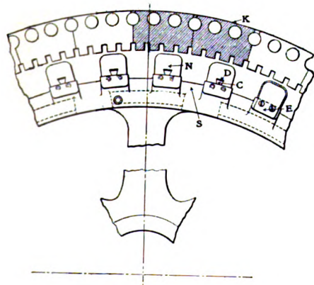
FIG. 5.—SECTION OF A STANLEY-G. I. INDUCTOR ALTERNATOR
