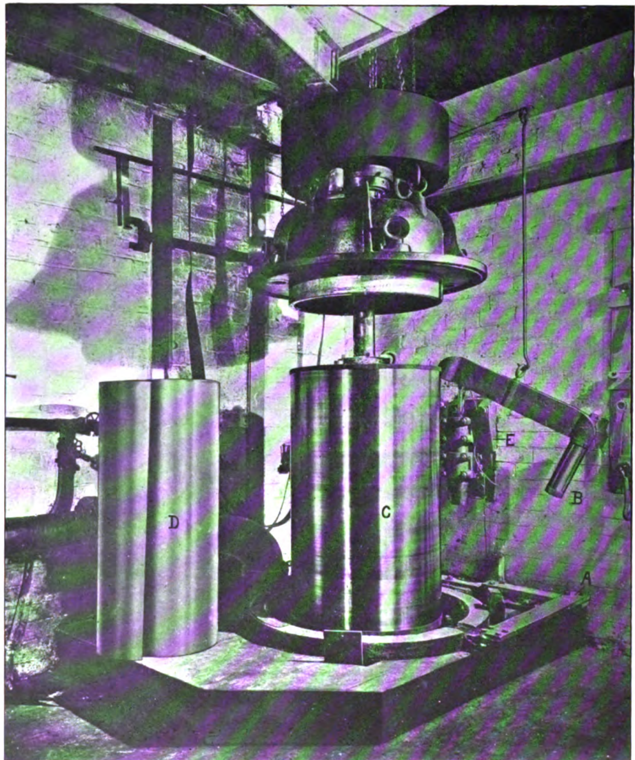
FIG. 8.—PLANT FOR DEPOSITING LARGE COPPER CYLINDERS
