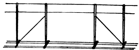
FIG. 5.—HEAD GUYING
