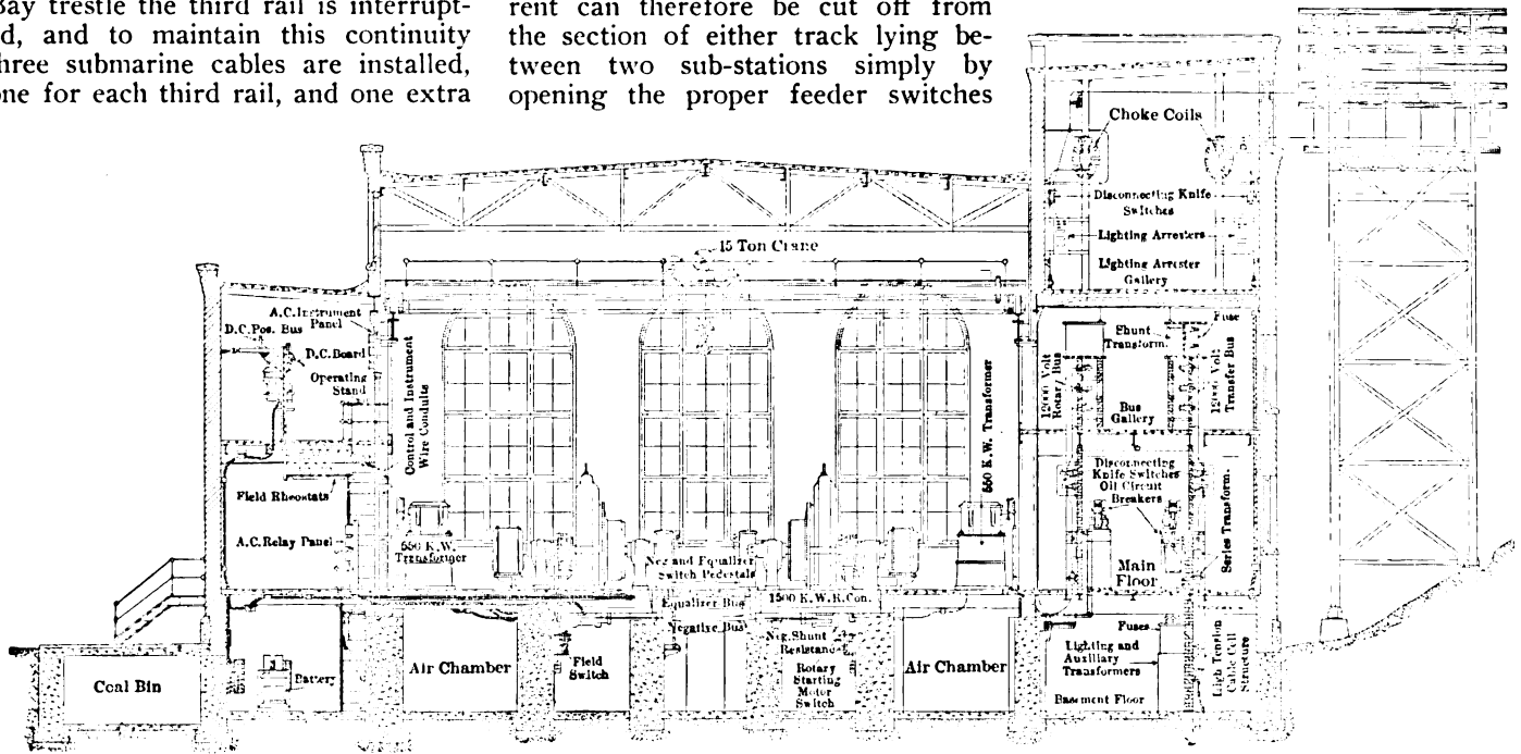
FIG. 10.—SECTIONAL ELEVATION OF THE SUB-STATION AT WOODHAVEN JUNCTION
