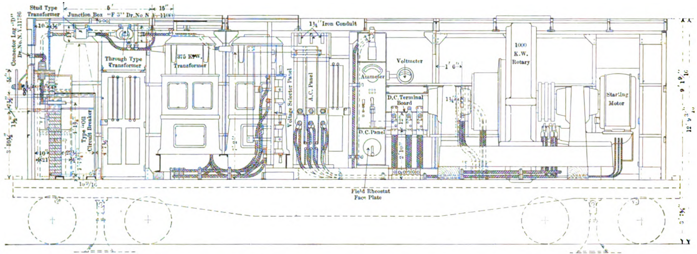
FIG. 13.—SECTIONAL ELEVATION OF A SUB-STATION CAR, SHOWING ARRANGEMENT OF THE EQUIPMENT
