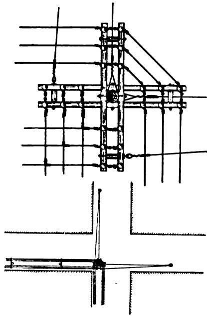
FIG. 7.—ONE-POLE METHOD OF TURNING A CORNER
