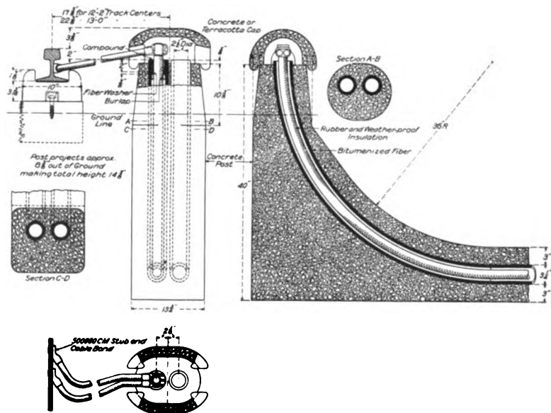
FIG. 8.—THIRD-RAIL JUMPER, USED AT ALL GRADE CROSSINGS
