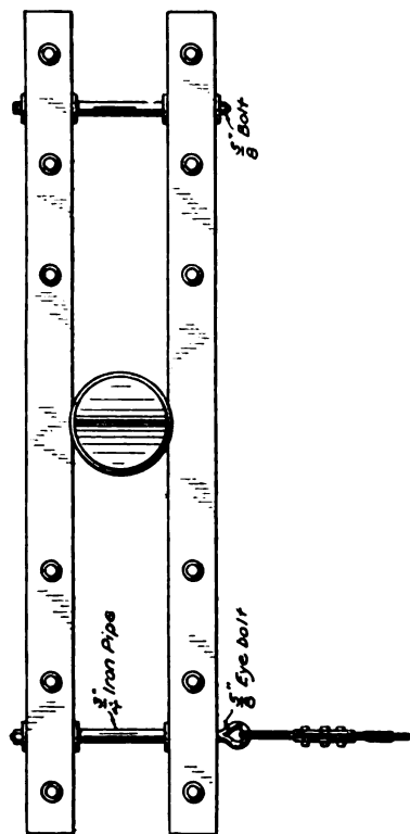
FIG. 13.—A DOUBLE CROSS-ARM
