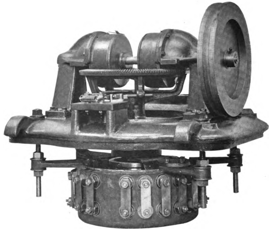
FIG. 7.—COVER OF THE SWITCH-TYPE REGULATOR WITH CONTROLLING MECHANISM
