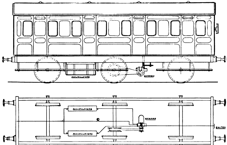
FIG. 13.—A BRITISH PASSENGER COACH EQUIPPED WITH THE ELECTRIC LIGHTING SYSTEM OF J. STONE & COMPANY, LTD., LEFFORD, LONDON
