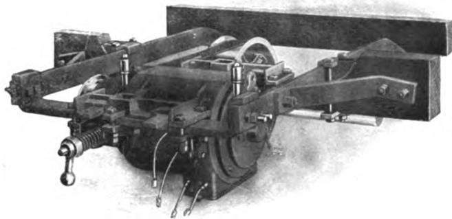
FIG. 8.—VIEW OF GENERATOR AND METHOD OF SUSPENSION IN THE SYSTEM OF THE BLISS ELECTRIC CAR LIGHTING COMPANY, OF MILWAUKEE, WIS.
