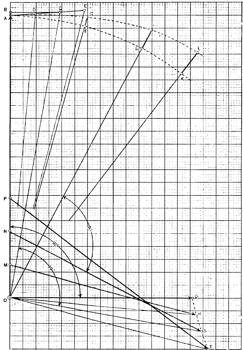
FIG. 3.—VECTOR DIAGRAM FOR 100 PER CENT. POWER FACTOR
