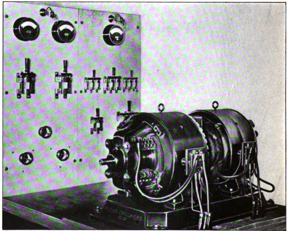
A 3-WIRE BALANCER BUILT BY THE ALLIS-CHALMERS COMPANY, OF MILWAUKEE, FOR A MULTI-VOLTAGE SYSTEM OF MOTOR CONTROL
