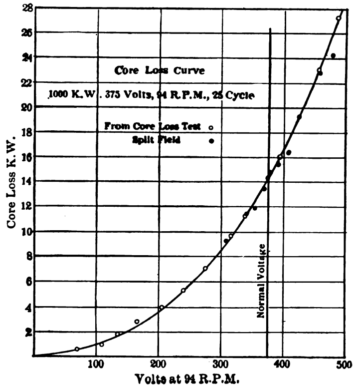
FIG. 8.—COMPARISON OF CORE LOSSES OBTAINED ON OPEN CIRCUIT AND IN THE BEHREND SPLIT-FIELD TEST. SEE PAGE 393
