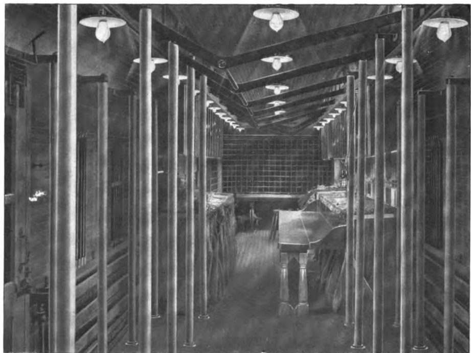
FIG. 19.—A POSTAL CAR LIGHTED ON THE MOSKOWITZ SYSTEM OF THE UNITED STATES LIGHT & HEATING COMPANY
