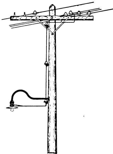
FIG. 21.—INCANDESCENT LAMP SUSPENSION WITH DUPLEX CONDUCTOR LOOP
