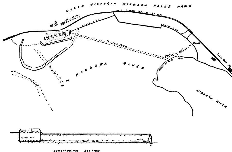
GENERAL PLAN OF THE ELECTRICAL DEVELOPMENT COMPANY'S UTILIZATION OF NIAGARA POWER
