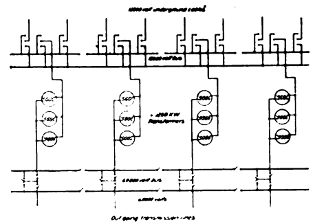
FIG. 9.—DIAGRAM OF CONNECTIONS OF TRANSFORMER HOUSE CIRCUITS
