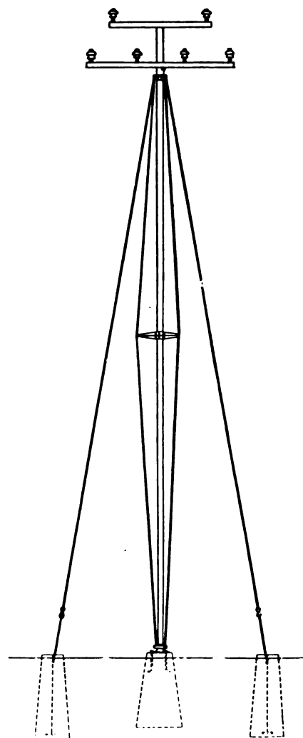
FIG. 13.—POLE FOR THE BUFFALO TRANSMISSION LINE
