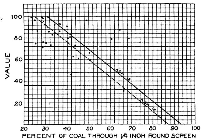
FIG. 11.—EFFECT OF SCREENED COAL ON VALUE
