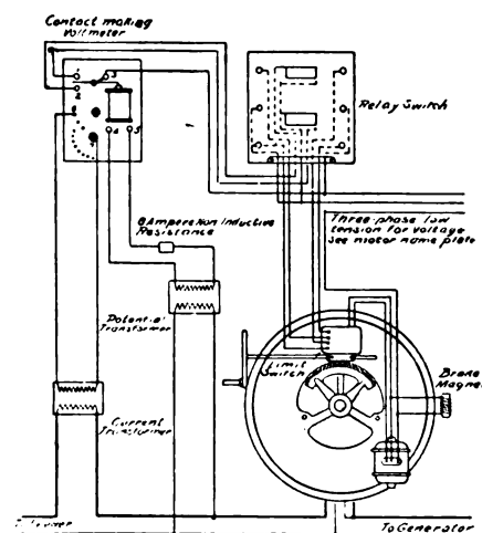
FIG. 11.—DIAGRAM OF CONNECTIONS OF POTENTIAL RELAY
