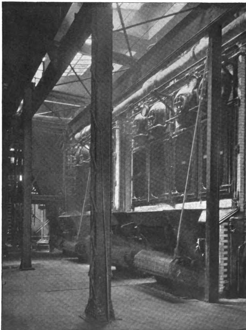
THE BABCOCK & WILCOX BOILERS IN THE CENTRAL POWER PLANT OF THE ESTATE OF HENRY W. OLIVER, PITTSBURG, PA., ARE PROVIDED WITH CHAIN GRATES MADE BY THE GREEN ENGINEERING COMPANY, CHICAGO
