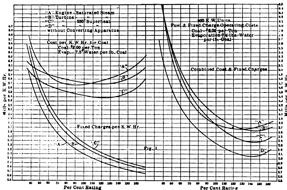
FIG. 1.—FUEL AND FIXED CHARGE OPERATING COSTS OF A 500-KW. RECIPROCATING ENGINE UNIT AND A STEAM TURBINE UNIT OF THE SAME CAPACITY
