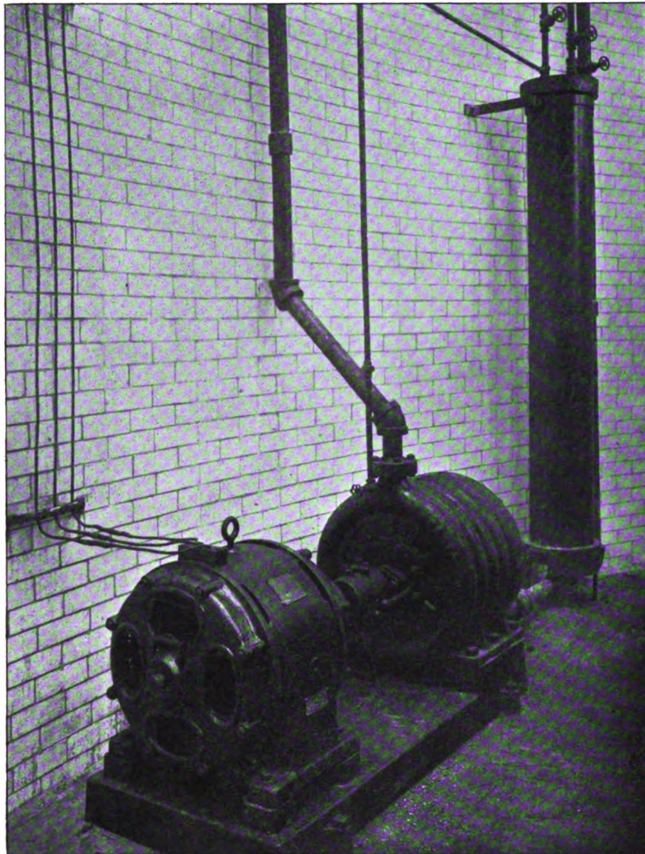
FIG. 3.—A 5-STAGE MOTOR-DRIVEN WORTHINGTON PUMP SUPPLYING WATER AT 200 POUNDS PRESSURE FOR OPERATING THE HYDRAULIC VALVES
