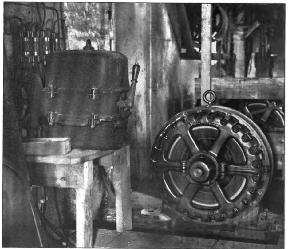
ONE OF TWO 50-H. P. INDUCTION MOTORS INSTALLED BY THE WESTINGHOUSE ELECTRIC & MANUFACTURING COMPANY, OF PITTSBURG, IN THE PLANT OF THE SPRINGFIELD, OHIO, METALLIC CASKET COMPANY
