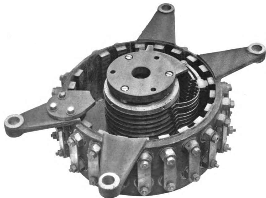
FIG. 8.—THE SWITCH OF THE AUTOMATIC FEEDER REGULATOR
