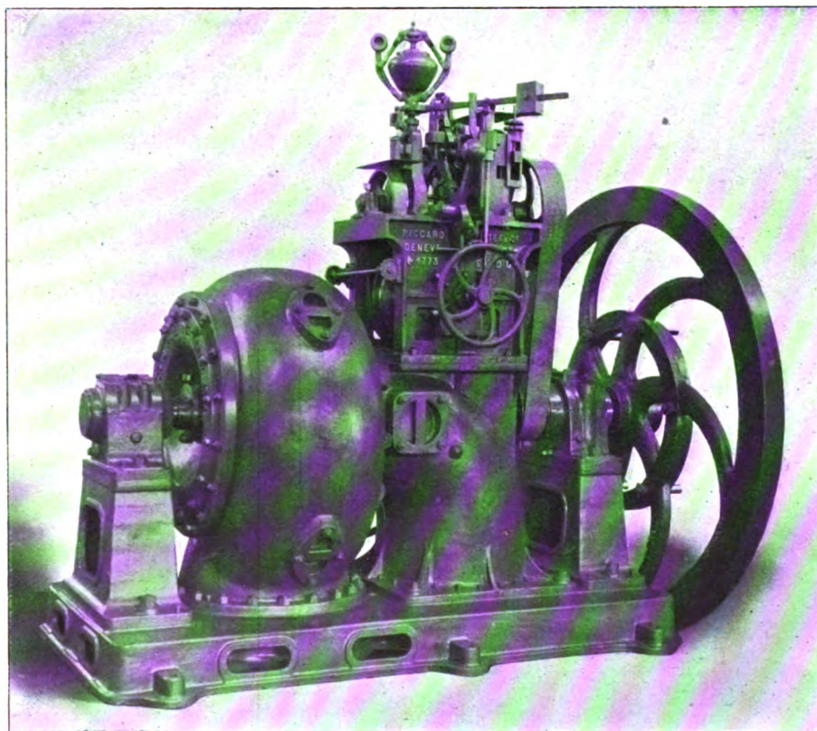
FIG. 15.—ONE OF THE TURBINES USED IN AN ITALIAN HYDRO-ELECTRIC PLANT
