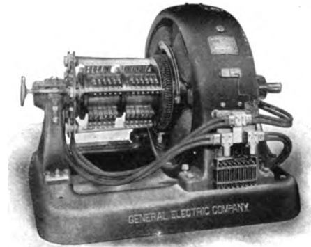
A MOTOR BUILT BY THE GENERAL ELECTRIC COMPANY, OF SCHENECTADY, N. Y., FOR TESTING PURPOSES AT THE WORTHINGTON HYDRAULIC WORKS, HARRISON, N. J.
