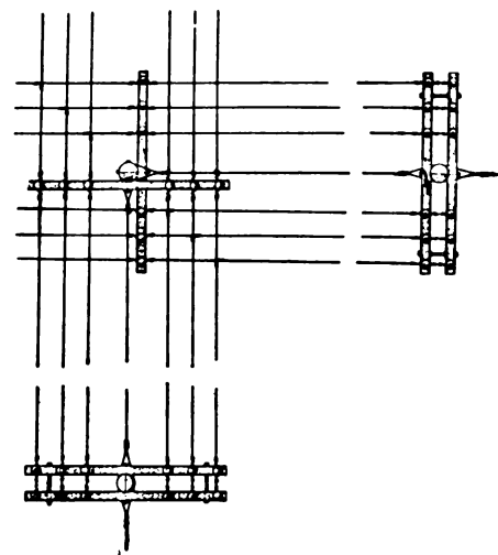
FIG. 18.—CORNER POLE WITHOUT DOUBLE CURVES
