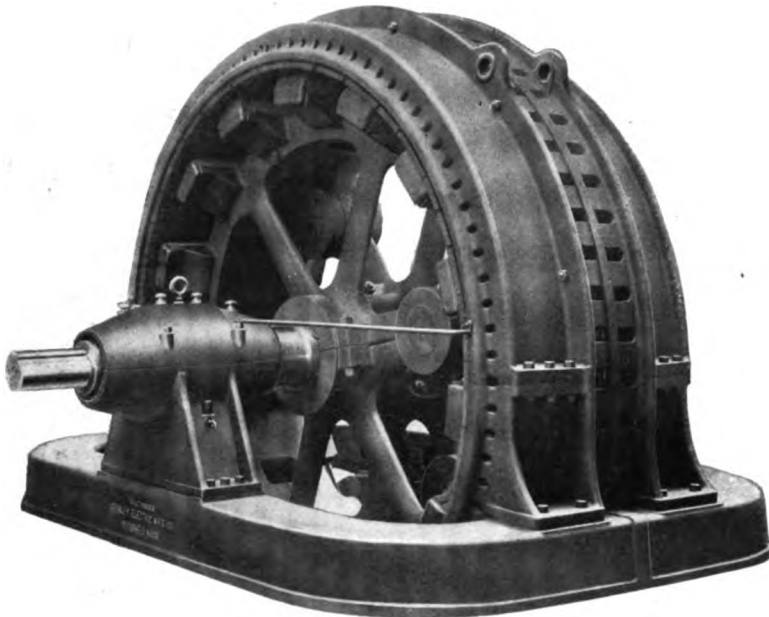
FIG. 8.—A 2000-KW. WATER-WHEEL TYPE OF INDUCTOR ALTERNATOR BUILT BY THE STANLEY-G. I. ELECTRIC MANUFACTURING COMPANY, OF PITTSFIELD, MASS.
