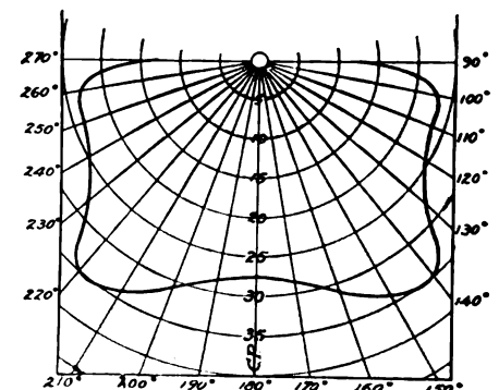
CURVE SHOWING LIGHT DISTRIBUTION OF A TANTALUM LAMP WITH A DISTRIBUTING FORM OF REFLECTOR
