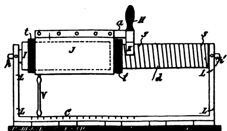
FIG. 8.—ANOTHER WAVE-METER DEvised BY FLEMING
