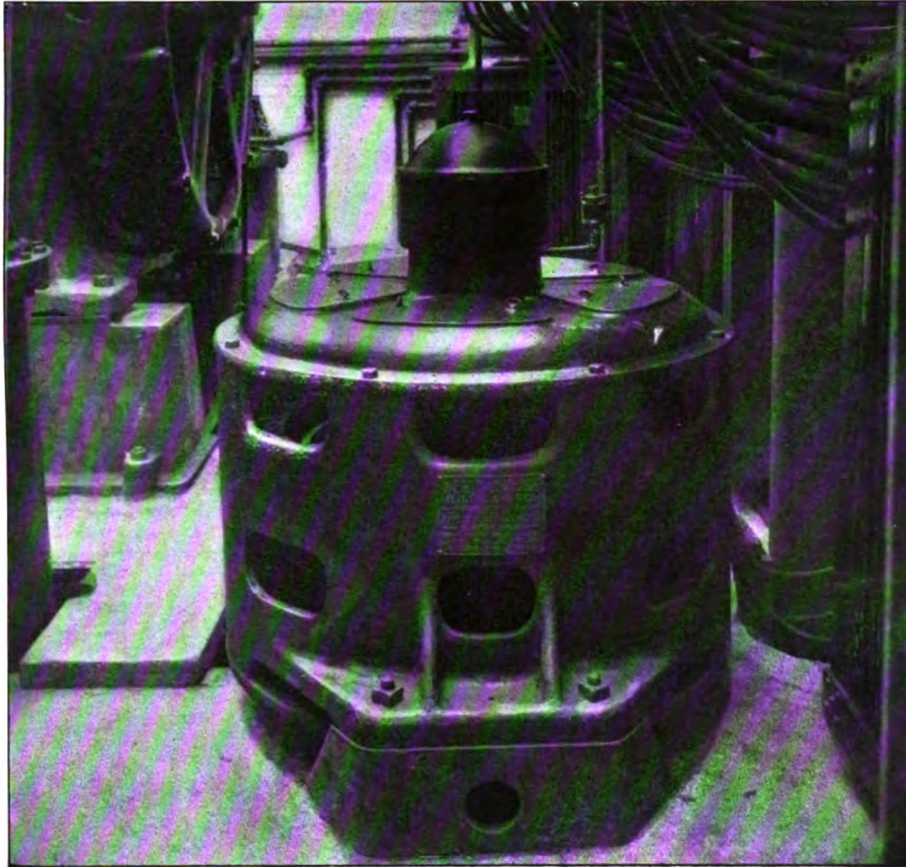
FIG. 4.—A 75-H. P. VERTICAL MOTOR DRIVING A DRAINAGE PUMP
