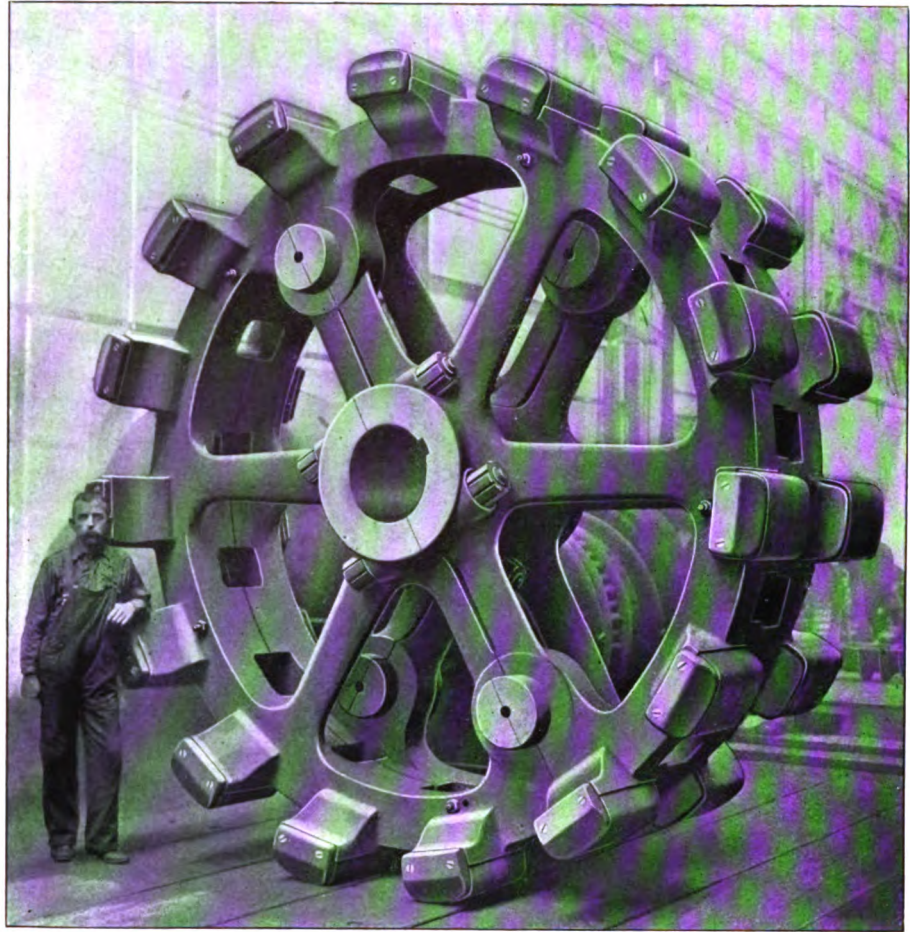
FIG. 6.—INDUCTOR OF A 2000-KW. INDUCTOR ALTERNATOR BUILT BY THE STANLEY-G. I. ELECTRIC MANUFACTURING COMPANY, OF PITTSFIELD, MASS.
