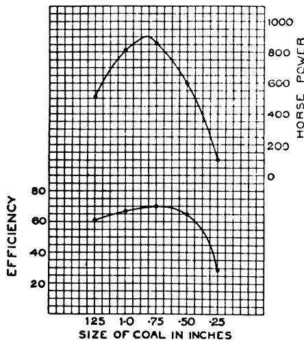
FIG. 1.—EFFECT ON CAPACITY AND EFFICIENCY DUE TO COAL OF DIFFERENT SIZES
