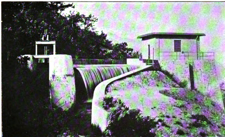
FIG. 4.—THE END OF THE CONDUIT FROM THE MAROBBLIA RIVER AND THE GATE HOUSE FROM WHICH THE PENSTOCK CONVEYS THE WATER TO THE POWER PLANT
