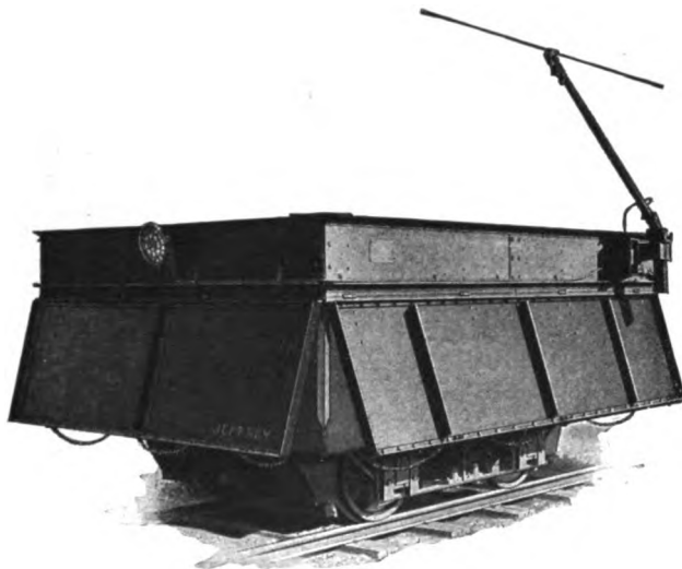
FIG. 2.—ANOTHER VIEW OF THE JEFFREY ELECTRIC DUMP CAR, SHOWING SIDES OPEN
