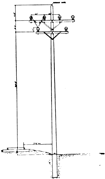
FIG. 4.—A POLE USED ON THE HIGH-TENSION TRANSMISSION LINE
