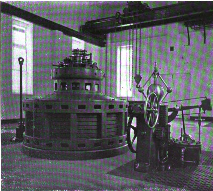
FIG. 3.—A NEARER VIEW OF ONE OF THE GENERATORS AND A WATER-WHEEL GOVERNOR
