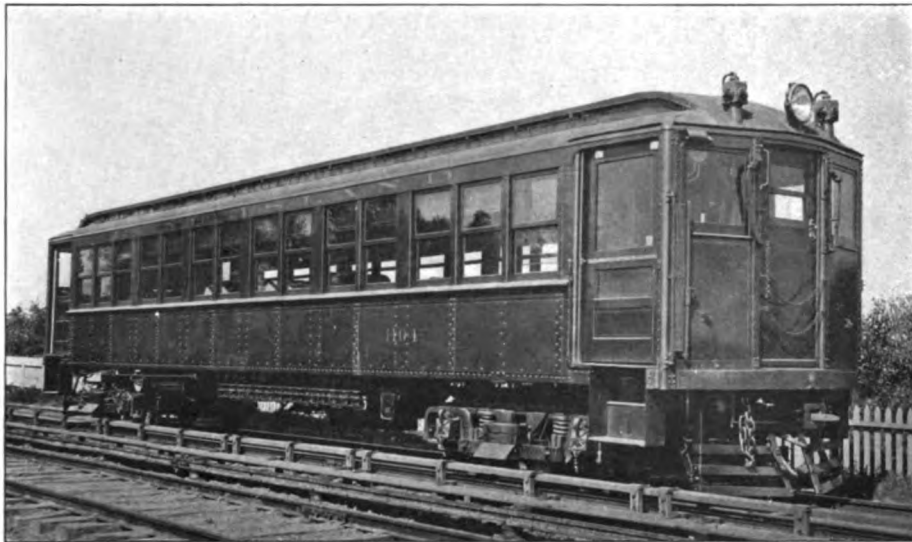
FIG. 1.—A STEEL MOTOR CAR FOR THE LONG ISLAND RAILROAD, BUILT AT THE BERWICK (PA.) SHOPS OF THE AMERICAN CAR & FOUNDRY COMPANY
