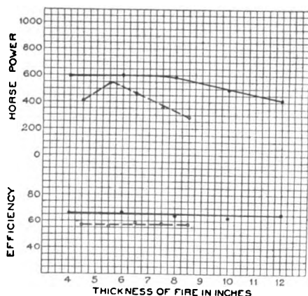
FIG. 5.—RESULT OF DIFFERENT THICKNESSES OF FIRE
