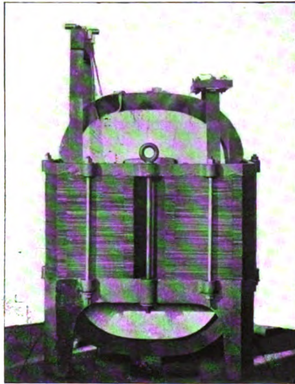
CORE AND COILS OF AN ALLIS-CHALMERS OIL-FILLED TRANSFORMER
