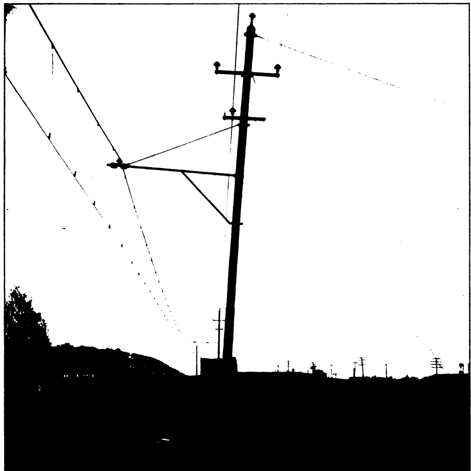
FIG. 3.—THE POLE WAS DEFLECTED AS HERE SHOWN UNDER A STRAIN OF 2050 POUNDS AT THE TOP, EXERTED AT A DISTANCE OF 125 FEET
