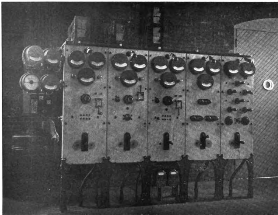
THE SWITCHBOARD IN THE CITIZENS' ELECTRIC COMPANY'S PLANT
