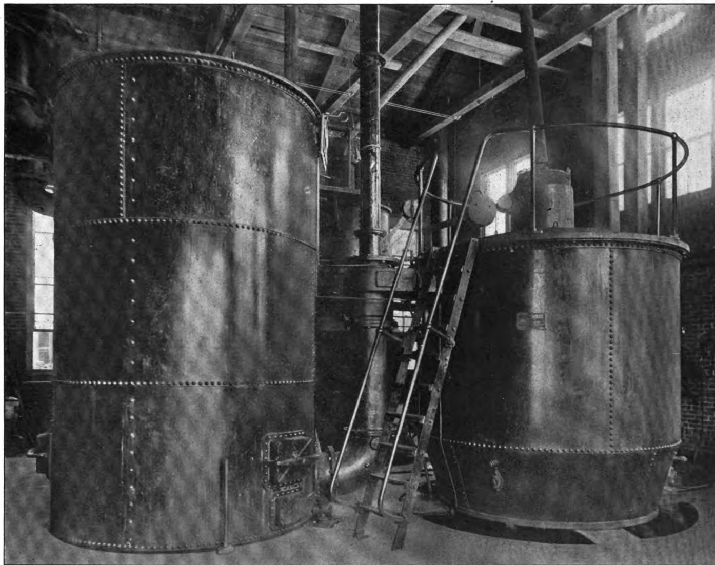
A PART OF THE GAS-PRODUCER PLANT OF THE CITIZENS' ELECTRIC COMPANY. TWO 250-H. P. SETS ARE INSTALLED, ONE BEING SHOWN HERE. ON THE RIGHT IS THE PRODUCER SHELL, WITH THE COAL-CHARGING HOPPER ON TOP. ON THE LEFT IS THE SCRUBBER
