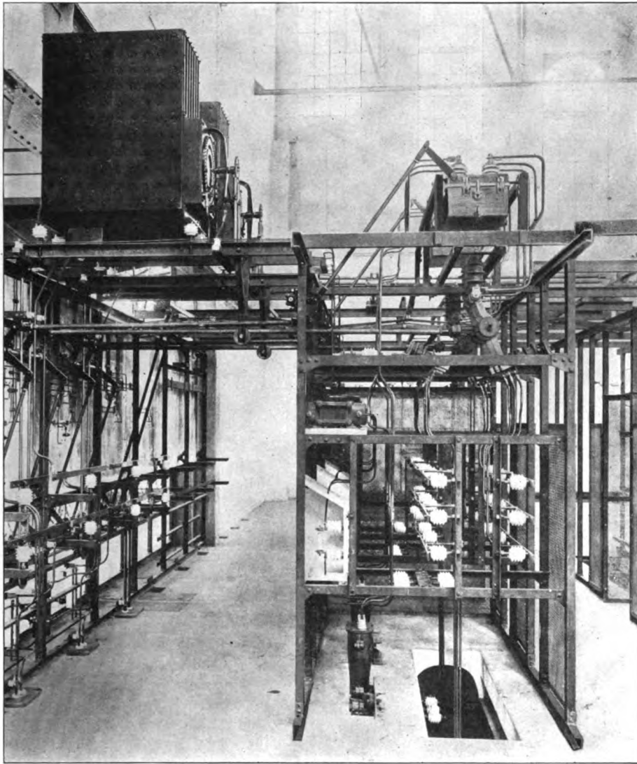
FIG. 22.—OIL SWITCHES IN THE GLOMMEN RIVER PLANT
