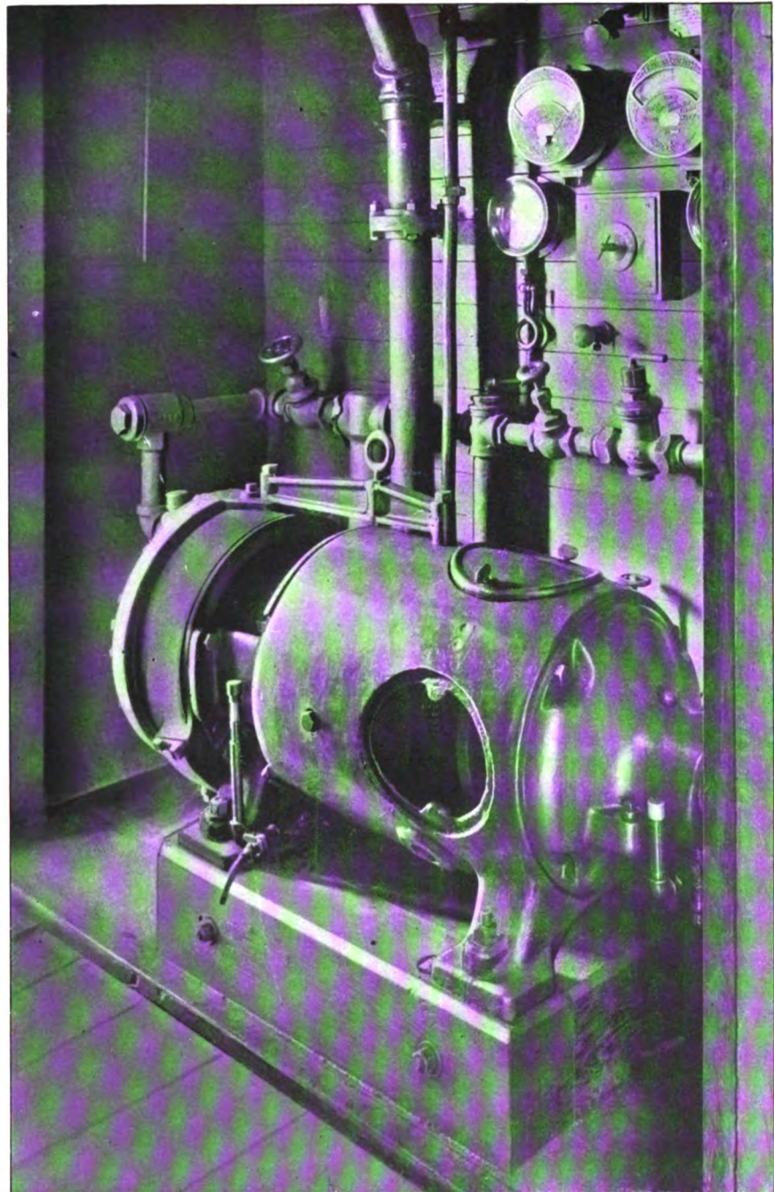
FIG. 7.—BAGGAGE CAR EQUIPPED WITH A CURTIS STEAM-TURBINE-DRIVEN GENERATOR FOR ELECTRIC TRAIN LIGHTING
