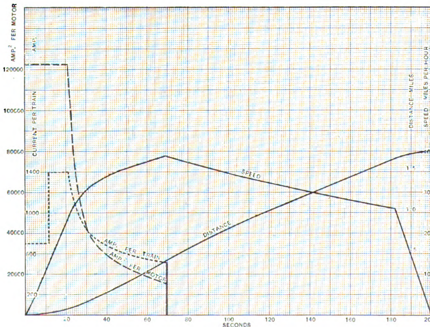
FIG. 9.—TYPICAL SPEED TIME CURVE OF A 117-TON TRAIN
