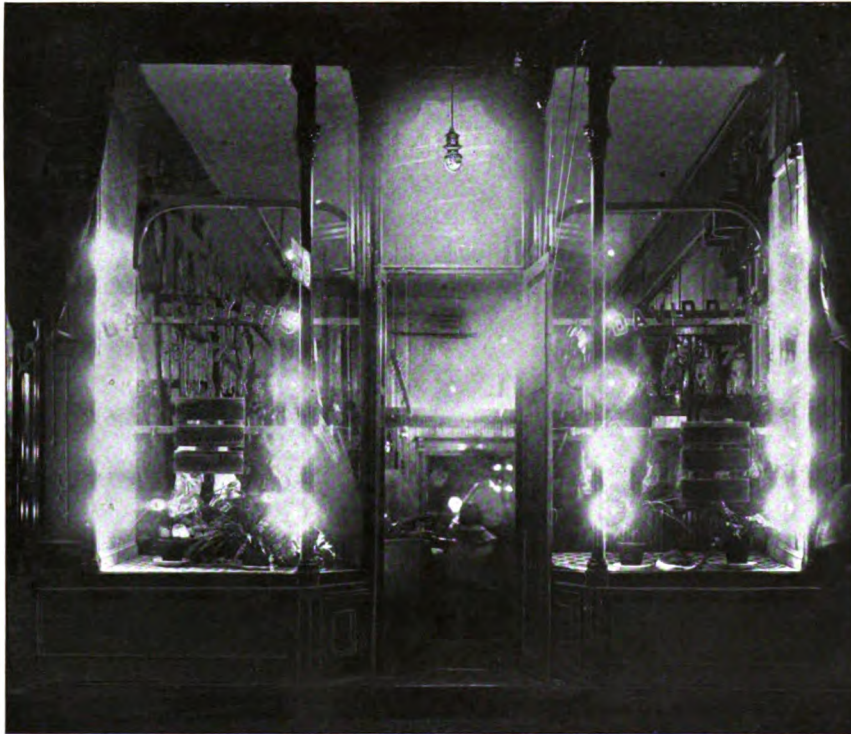
PERMISSIBLE WINDOW ILLUMINATION FOR A BUTCHER SHOP
