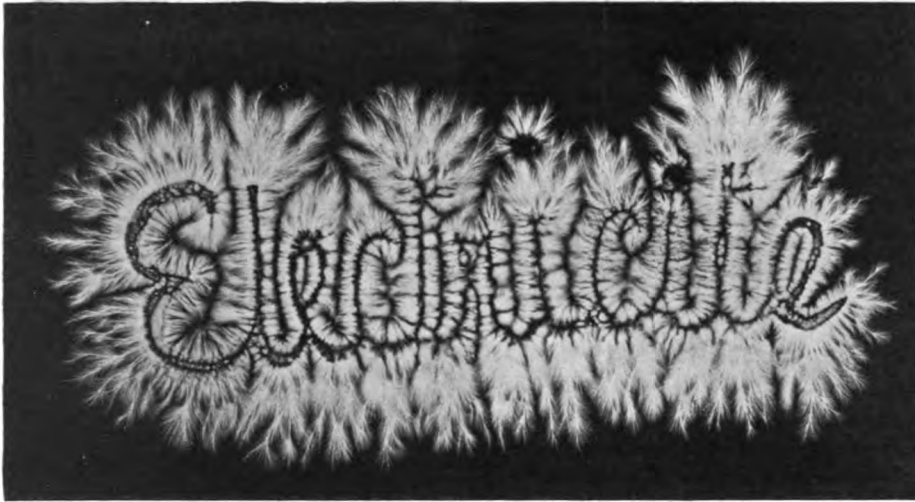
FIG. 1.—A PHOTOGRAPH OF A SPARK DISCHARGE TRACING THE WORD "ELECTRICITE"
