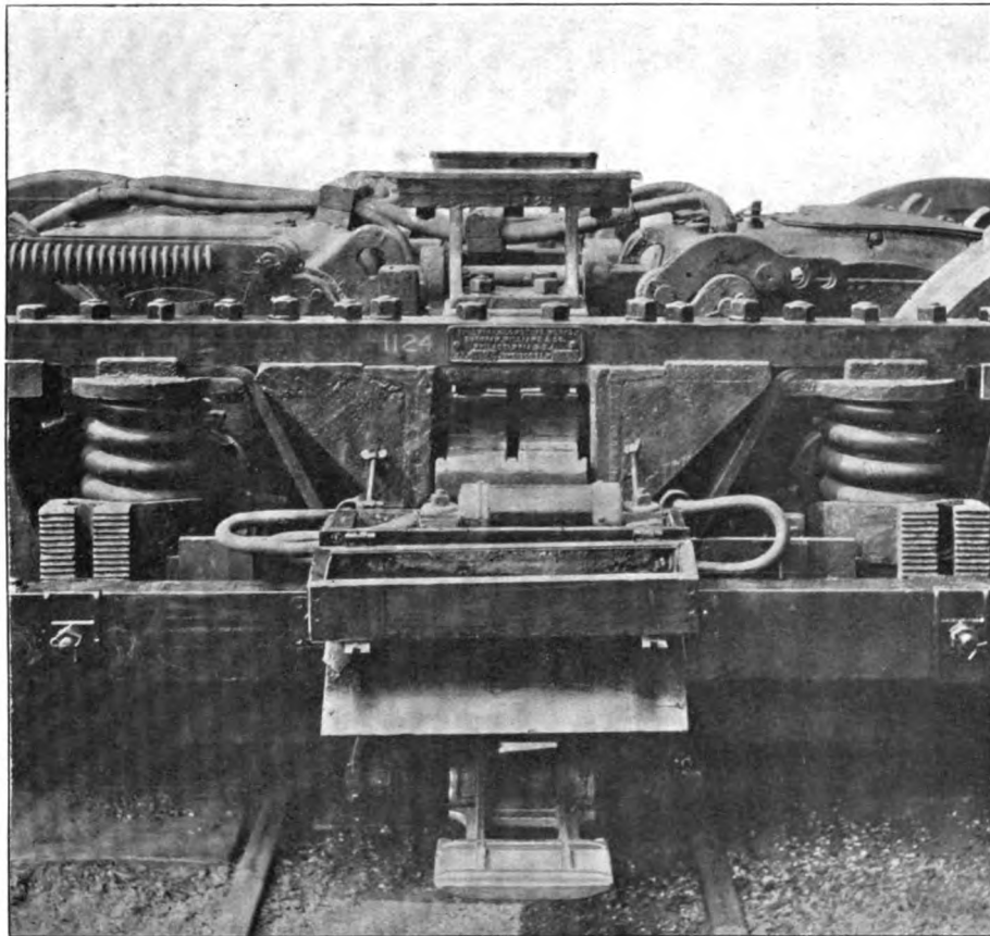
FIG. 3.—THE THIRD-RAIL SHOE, FUSE, AND CONNECTIONS
