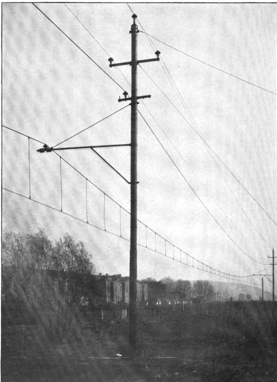
FIG. 1.—GENERAL VIEW OF THE EXPERIMENTAL LINE FOR TESTING OVERHEAD CATENARY CONSTRUCTION, ERECTED BY ELMER P. MORRIS, NEW YORK, REPRESENTING THE ELECTRIC RAILWAY EQUIPMENT COMPANY, CINCINNATI, OHIO
