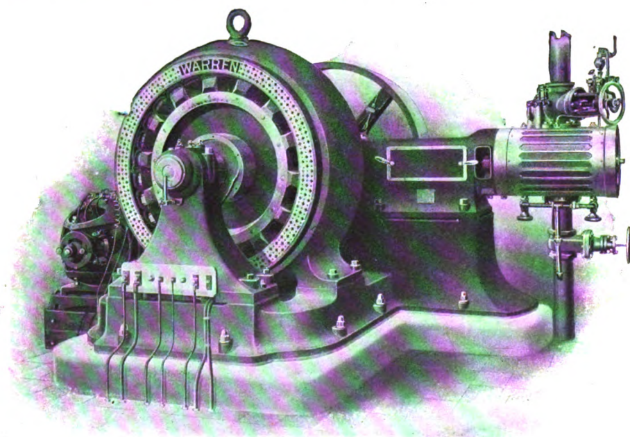
FIG. 4.—A WARREN INDUCTOR ALTERNATOR DIRECT CONNECTED TO A STEAM ENGINE
