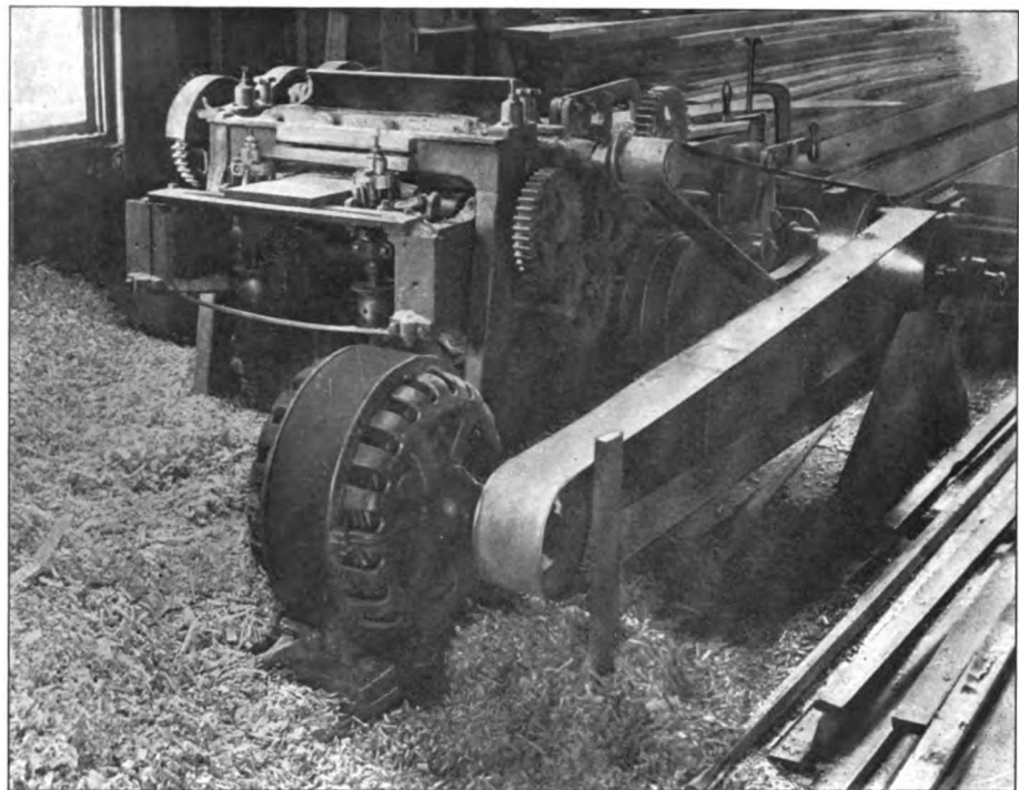
A 15-H. P. WESTINGHOUSE INDUCTION MOTOR DRIVING A PLANER IN THE LUMBER MILL OF THE EGGERS & GRAHAM LUMBER COMPANY, UNIONTOWN, PA.
