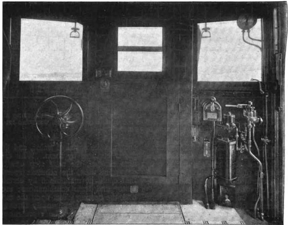
FIG. 7.—VESTIBULE OF STEEL MOTOR CAR
