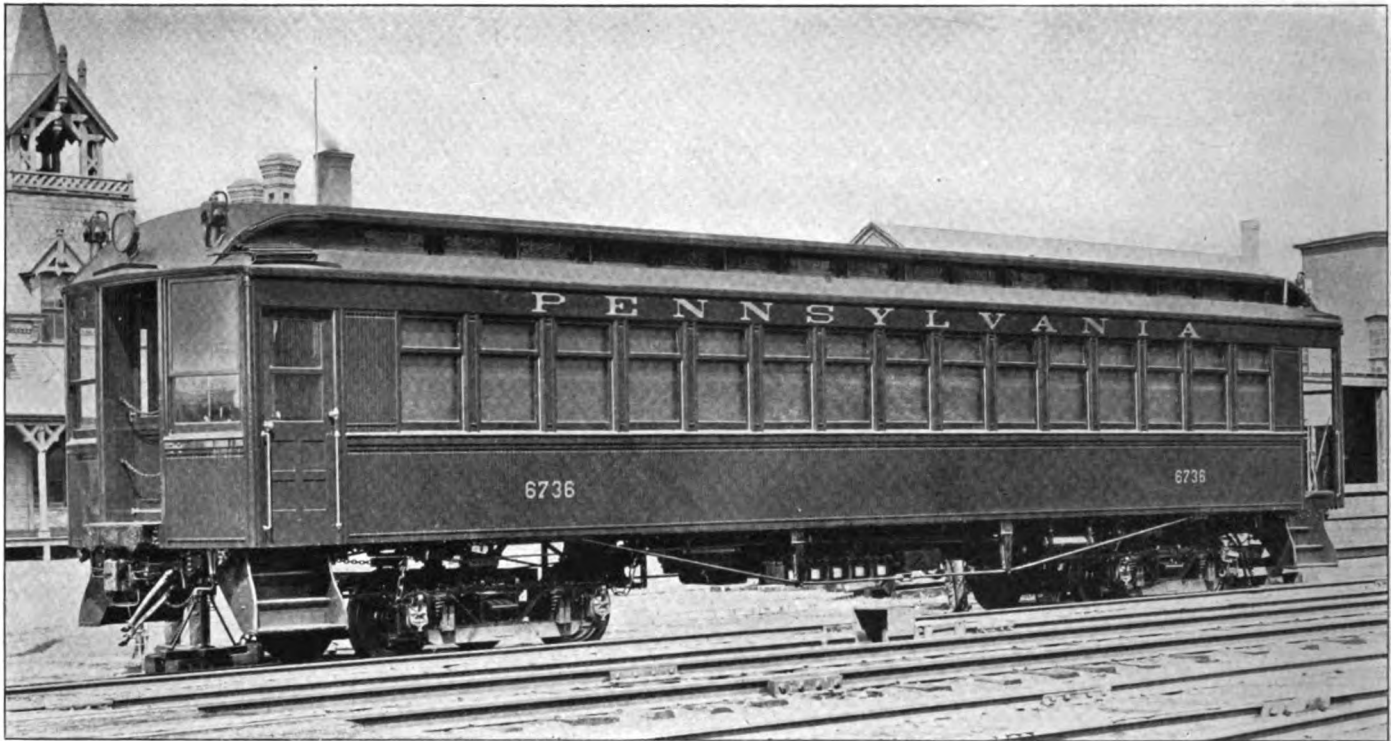
FIG. 9.—A STEEL MOTOR CAR ON THE WEST JERSEY & SEASHORE BRANCH OF THE PENNSYLVANIA RAILROAD
