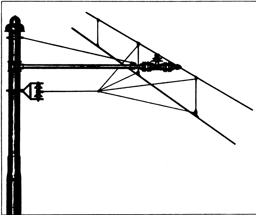
FIG. 2.—CATENARY CONSTRUCTION IN WHICH A BRIDLE GUY IS USED
