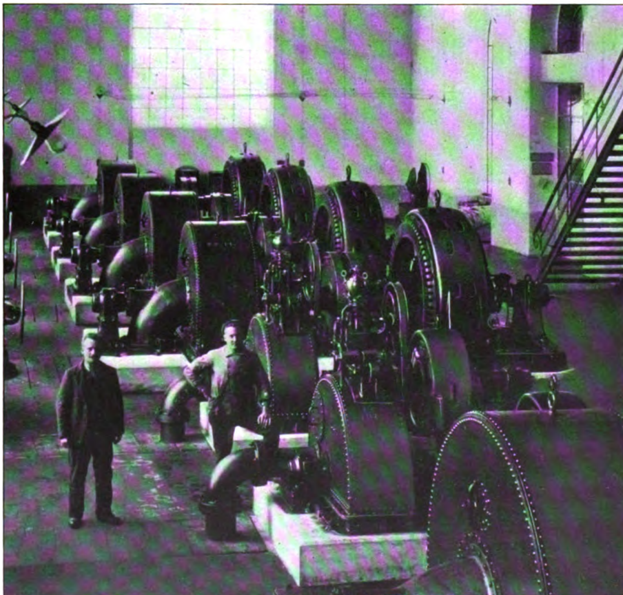
FIG. 11.—INTERIOR OF THE TUSCIANO RIVER PLANT IN ITALY, SHOWING FIVE 1400-H. P. UNITS AND TWO 150- H. P. EXCITER UNITS
