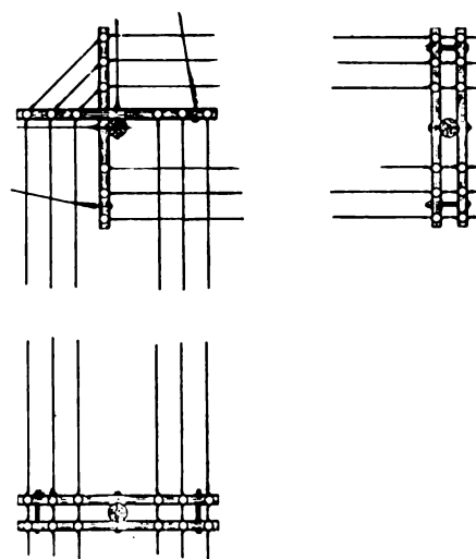
FIG. 14.—A CORNER POLE WITHOUT DOUBLE ARMS
