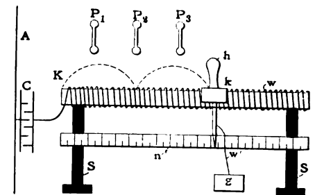
FIG. 4.—FLEMING'S WAVE-METER
