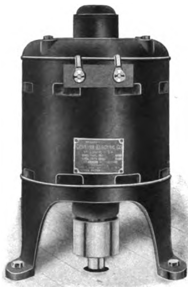
A VERTICAL SINGLE-PHASE SELF-STARTING MOTOR BUILT BY THE CENTURY ELECTRIC COMPANY, ST. LOUIS, MO.
