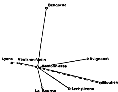
FIG. 1.—DIAGRAM SHOWING RELATIVE LENGTH AND LOCATION OF HIGH-TENSION LINES SUPPLYING HYDRO-ELECTRIC POWER TO LYONS, IN FRANCE
