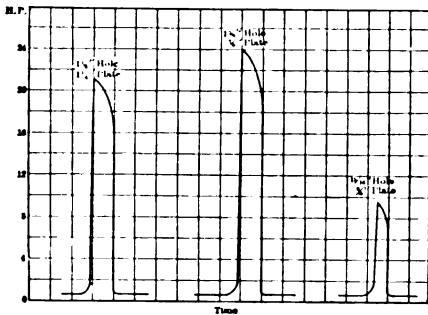
FIG. 3.—POWER CONSUMPTION OF A HILLES & JONES PUNCH
