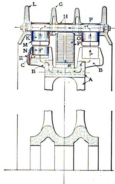
FIG. 7.—SECTION OF A STANLEY-G. I. ALTERNATOR, SHOWING THE MAGNETIC PATH
