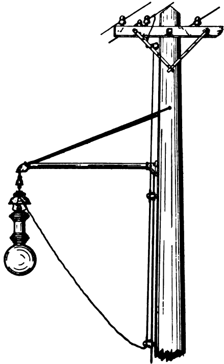
FIG. 19.—INNER ROPE ARC LIGHT SUSPENSION
