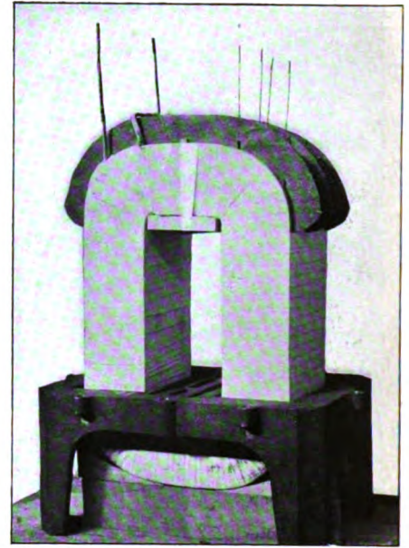
ASSEMBLED COILS OF AN ALLIS-CHALMERS OIL-FILLED TRANSFORMER
