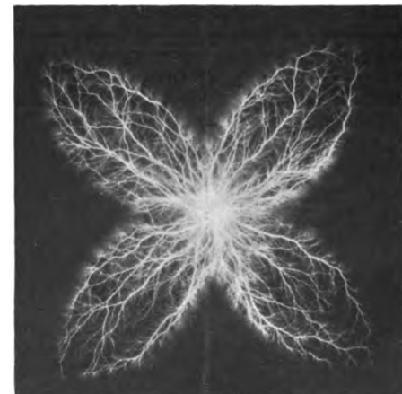
FIGS. 3 AND 4.—DECORATIVE SPARK DESIGNS
