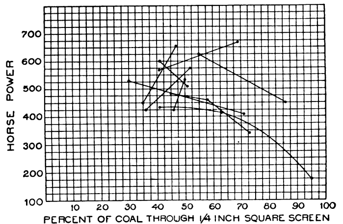
FIG. 9.—EFFECT OF SCREENED COAL ON HORSE-POWER
