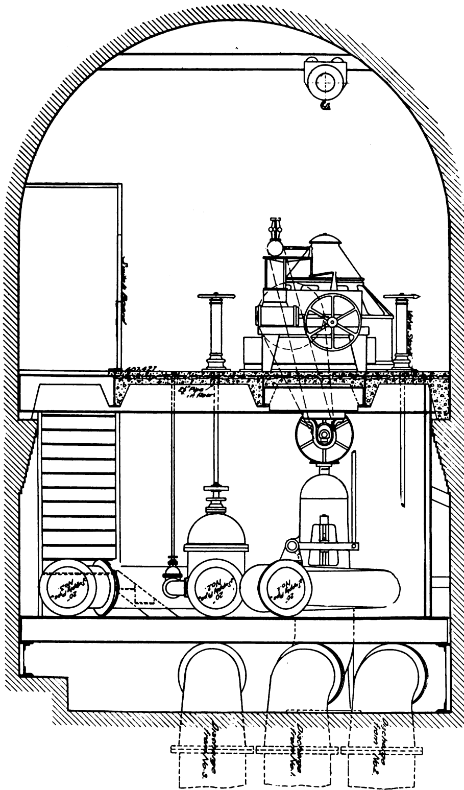
FIG. 8.—GENERAL ARRANGEMENT OF THE EXCITER PLANT
