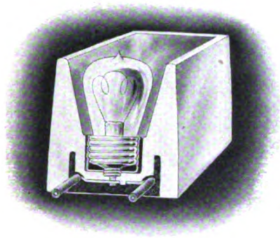
SECTIONAL VIEW OF A SIGN LETTER MADE BY THE COLONIAL SIGN & INSULATOR COMPANY, AKRON, OHIO
