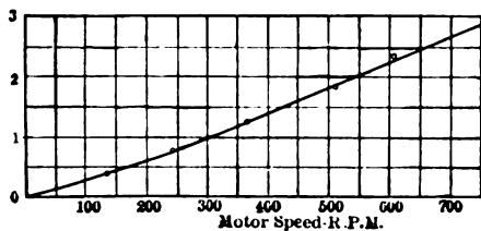
FIG. 4.—POWER LOST IN A 25-H. P. MOTOR
