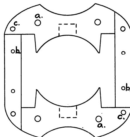
FIG. 4.—FORM OF LAMINATED FIELD OF AN EXPERIMENTAL SINGLE-PHASE MOTOR BUILT BY THE AUTHOR
