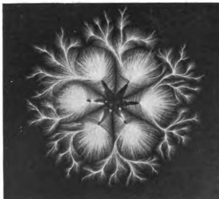
FIG. 2.—A DECORATIVE SPARK
