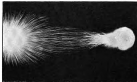
FIG. 6.—A DISCHARGE FROM TWO POLES OF OPPOSITE SIGN
