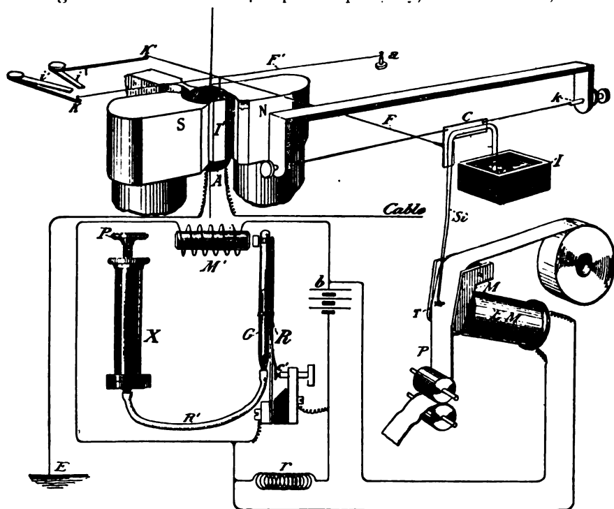
FIG. 7.—THE CUTTRISS SIPHON RECORDER
