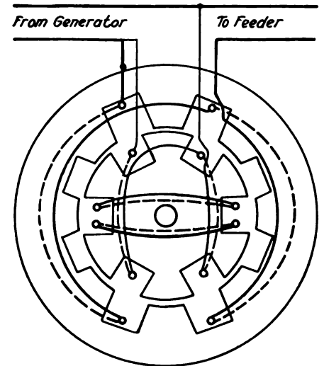
FIG. 13.—DIAGRAM SHOWING CONNECTIONS OF SINGLE-PHASE INDUCTION REGULATOR
