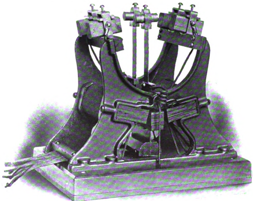
FIG. 16.—REVERSING SWITCH TO REVERSE THE DIRECTION OF THE MOTOR USED ON THE INDUCTION REGULATOR
