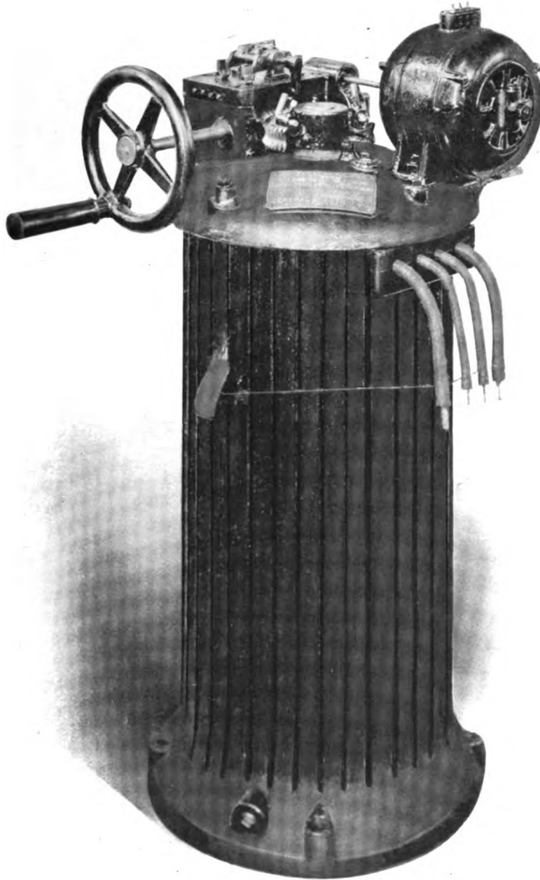
FIG. 12.—AN AUTOMATIC SINGLE-PHASE INDUCTION REGULATOR
