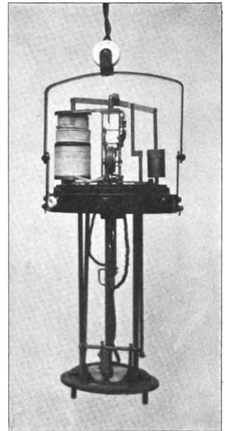
FIG. 8.—VIEW SHOWING THE MECHANISM OF THE SIEMENS FLAMING ARC LAMP
