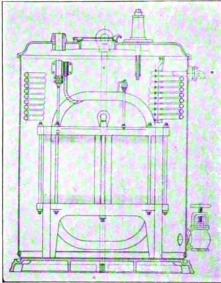
SECTIONAL VIEW OF AN OIL-FILLED, WATER-COOLED TRANSFORMER
