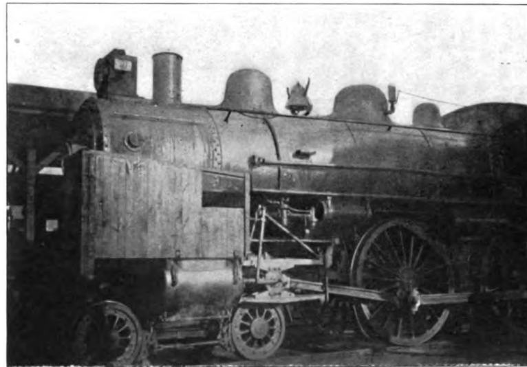
A LOCOMOTIVE FITTED WITH A WIND SHIELD FOR PROTECTION WHILE INDICATOR CARDS WERE TAKEN
