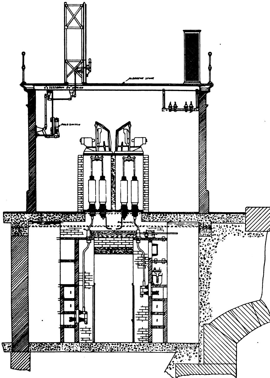
FIG. 5.—SECTION THROUGH SWITCHBOARD GALLERY
