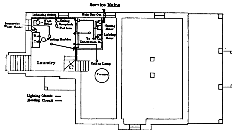
BASEMENT PLAN
