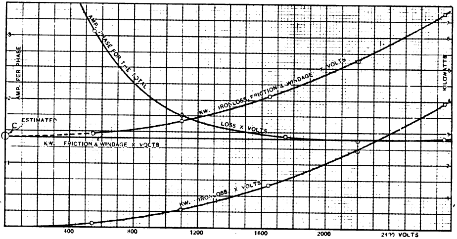
FIG. 7.—CURVES OF IRON, FRICTION AND WINDAGE LOSS
