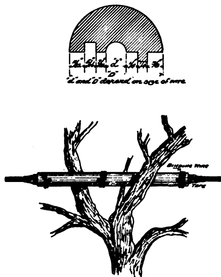
FIG. 16.—ABRASION MOULDING
