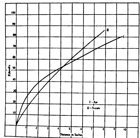
GRAPHIC REPRESENTATION OF TESTS TO DETERMINE THE RELATIVE TENDENCIES TO DIELECTRIC DISCHARGES IN ORDINARY AIR, IN STEAM, AND IN SMOKE
