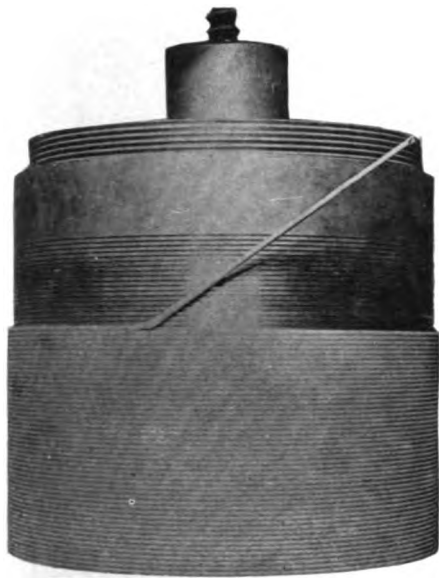
FIG. 13.—UNWINDING COPPER STRIP FOR WIRE
