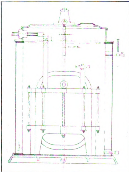
SECTIONAL VIEW OF AN OIL-FILLED, SELF-COOLING TRANSFORMER
