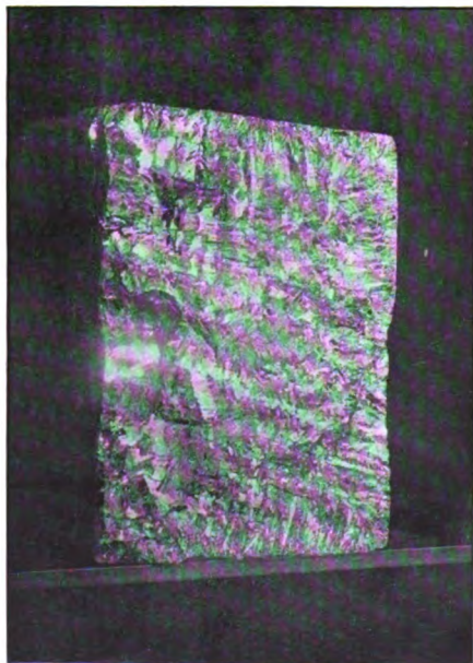
FIG. 10.—CAST ZINC, SHOWING LINES OF CLEAVAGE
