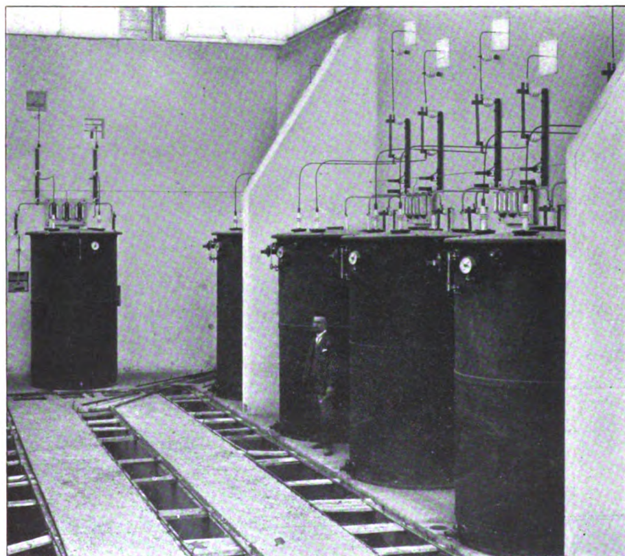
FIG. 9.—SINGLE-PHASE TRANSFORMERS AT THE CELLINA RIVER PLANT FOR RAISING THE PRESSURE FROM 4000 TO 36,000 VOLTS. FIVE GROUPS OF THREE SINGLE-PHASE TRANSFORMERS ARE INSTALLED
