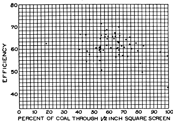
FIG. 10.—EFFECT OF SCREENED COAL ON EFFICIENCY
