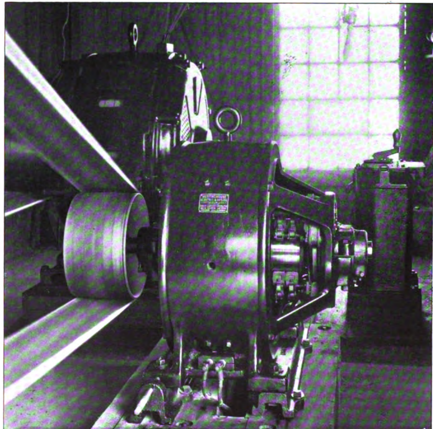
IN THE BACKGROUND IS A 100-H. P. INDUCTION MOTOR OPERATING KILNS. IN THE FOREGROUND IS A 22\frac{1}{2} -KW. EXCITER
