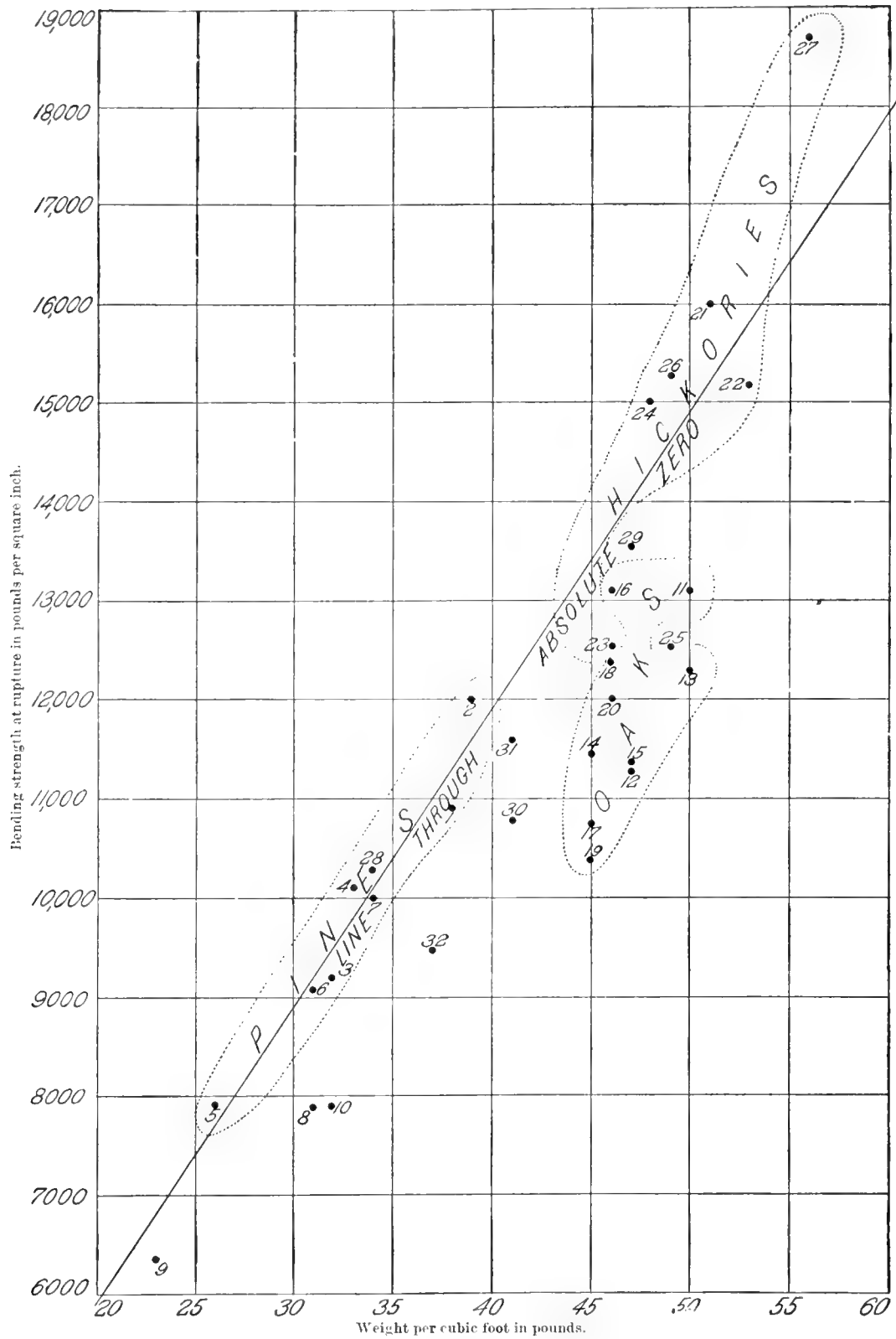
FIG. 36.—Relation of weight to bending strength at rupture. The figure at each point indicates the species thereby represented.
