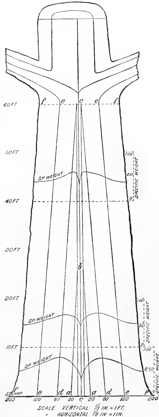
FIG. 92.—Schematic section through stem of long leaf pine, showing variation of specific weight, with height, diameter, and age, at 20 (aba), 60 (ded), 120 (eccc), 200 (ffff) years.
