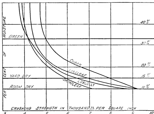
FIG. 2.—Diagram showing variation of compression strength with moisture.
