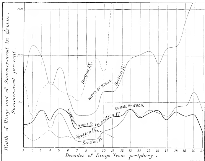
FIG. 15.—Variation of summerwood per cent with rate of growth (width of rings), in tree No. 3, Longleaf Pine.
