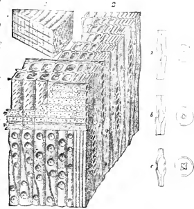
FIG. 16.—Schematic representation of coniferous wood structure: wood of spruce—1, natural size; 2, small part of one ring magnified 100 times. The vertical tubes are wood fibers, in this case all "tracheids," m , medullary or pith ray; a , transverse tracheids of pith ray; a , b , and c , bordered pits of the tracheids more enlarged.
