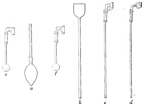
FIG. 9.—Tools used in turpentine orcharding: a , dipper; b , pusher; c , open puller; d , closed puller; e, f , hammer (front and rear view).
