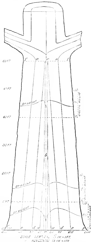
FIG. 2.—Schematic section through stem of Longleaf Pine, showing variation of specific weight with height, diameter, and age (at twenty, thirty, sixty, ninety, one hundred and twenty, one hundred and fifty, and two hundred years).
