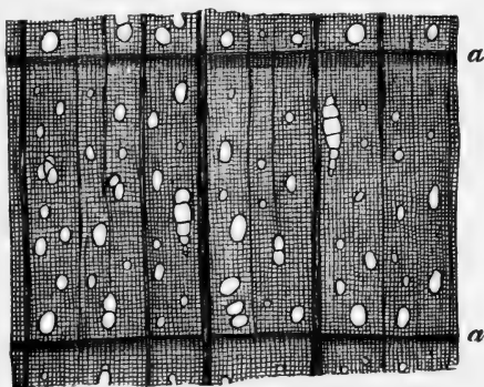
FIG. 9.—Transverse section of the wood of Acer pseudo-platanus , selected to show a type of timber common in Europe. The annual rings ( a ) are well-marked and regular. The vessels are small and numerous, and scattered somewhat equally over the whole breadth of the ring. The medullary rays are numerous, some broad, some fine. Many European timbers (beech, hornbeam, lime, &c.) agree with this type, except in detail.
