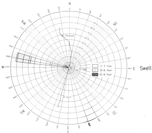
Figure 23. Sea and swell summary, gold experiments. Height in feet and direction from which the wave is approaching.
