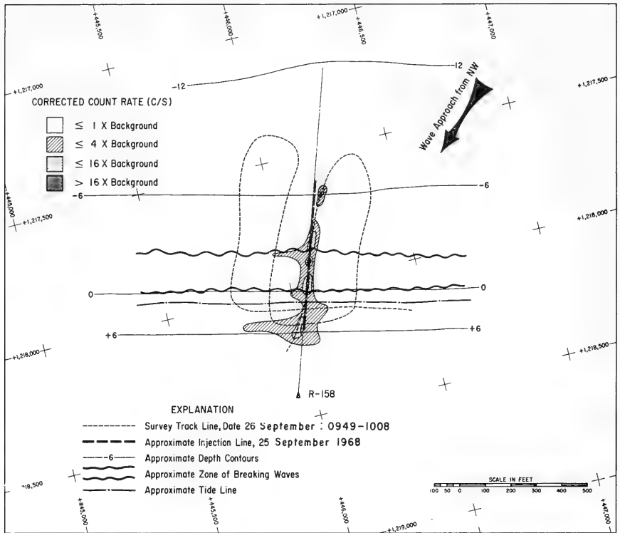
Figure 12. Pattern of xenonated sand approximately 24 hours after emplacement.
