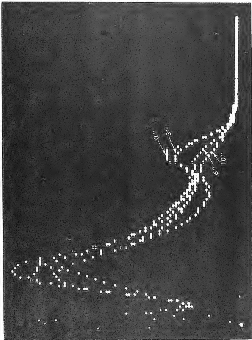
Figure 24. Changes in radioactive gold 198-199 spectrum resulting from burial by non-radioactive (dead) sand. Numbers indicate overburden thickness.
