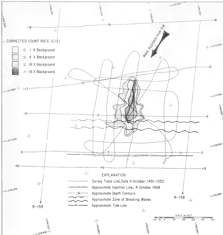
Figure 17. Dispersal pattern of gold-tagged sand approximately 4 hours after injection.
