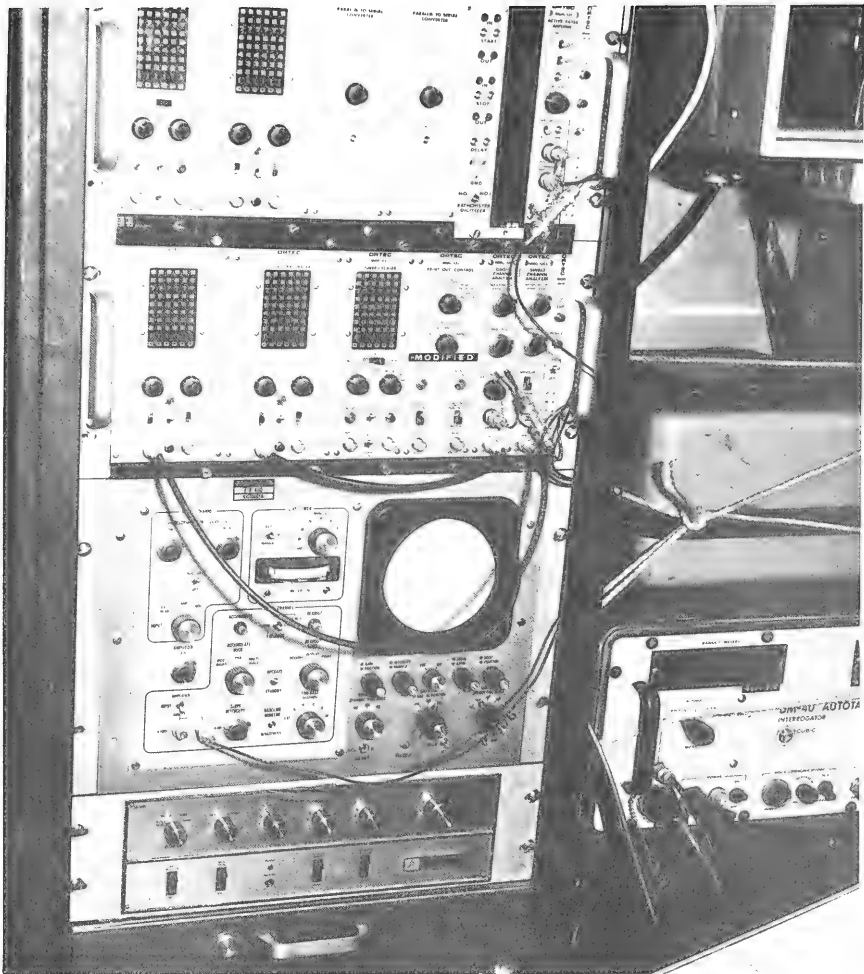
Figure 6. Onboard data acquisition system. Individual signals from the 4 scintillation detectors in the detector vehicle are fed through cables to a mixer in the instrument bank. A differential discriminator sorts the proper signals and feeds them to a multichannel analyzer (center bank). By means of a programmed interrogator (upper two banks), time and line sequence data are coordinated with the radiation data and read into the data display in real time and simultaneously onto punched paper tape. Navigation data is supplied from the Cubic Auto-tape interrogator (right).
