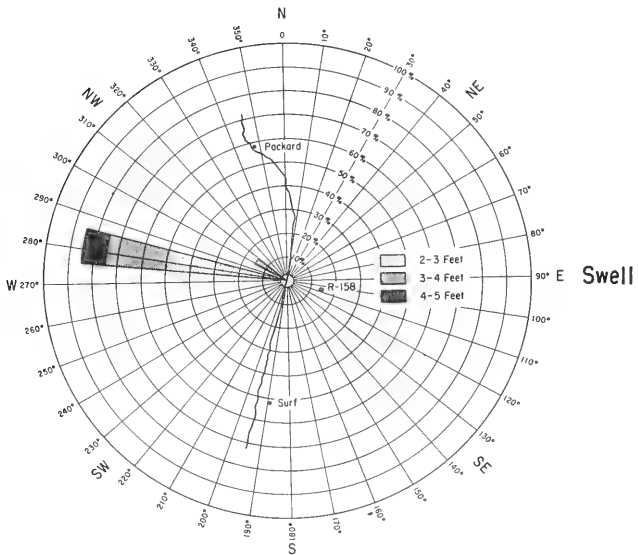
Figure 14. Sea and swell summary, xenon experiments. Height in feet and direction from which the waves are advancing.
