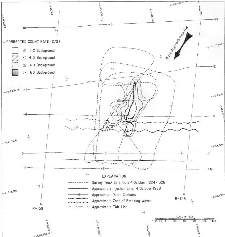
Figure 16. Dispersal pattern of gold-tagged sand approximately 2 hours after injection.
