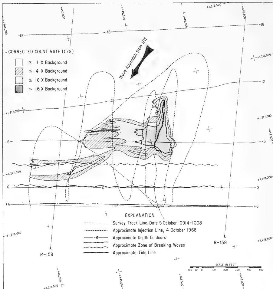
Figure 18. Dispersal pattern of gold-tagged sand approximately 23 hours after injection. Note the rather abrupt upcoast (north) truncation of the pattern and the minor movement shoreward.
