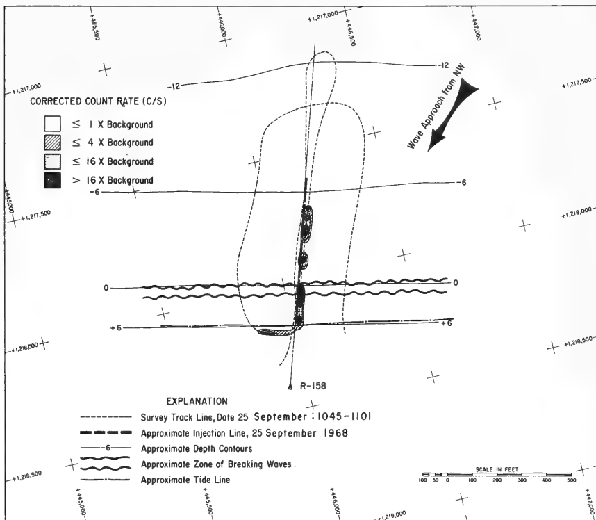
Figure 11. Pattern of xenonated sand immediately after release. The detector was operating and towed behind the LARC XV during emplacement of the sand.
