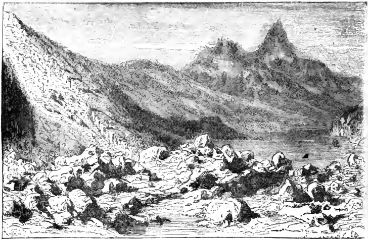
GOLDAU VALLEY BEFORE AND AFTER THE LANDSLIDE.
