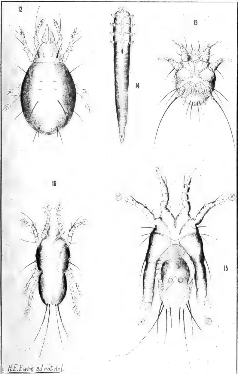
DIVERGING ADAPTATION.
