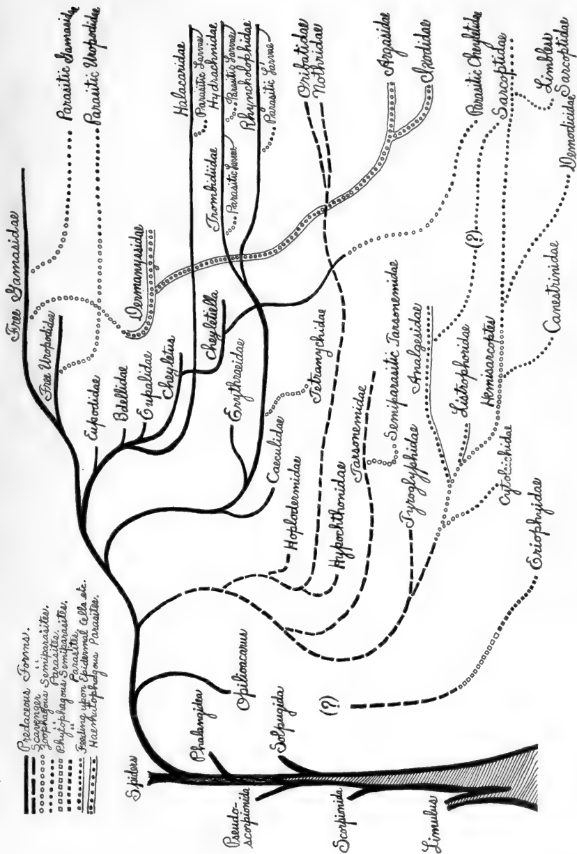
PHYLOGENETIC TREE.
