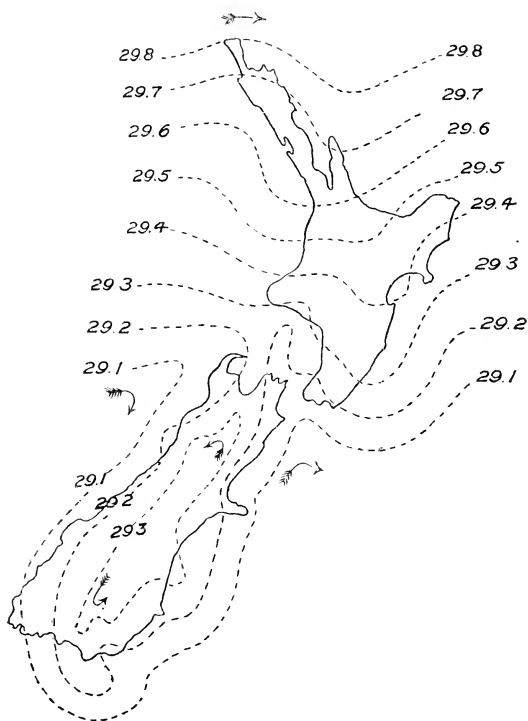
ISOBARS Schaw
