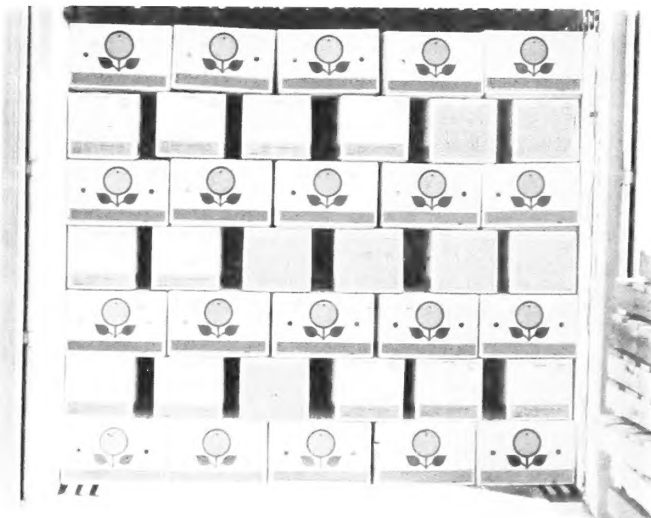
PN-5426 FIGURE 2.—Oranges in test van at Irvine, Calif., showing air-stack loading pattern.
