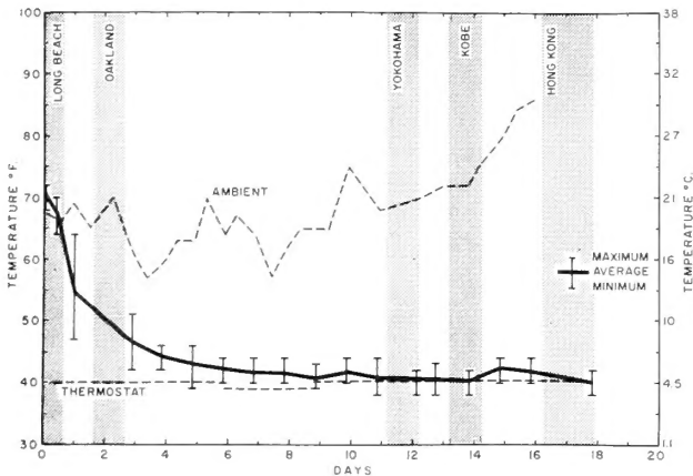
FIGURE 7.—Temperatures of oranges shipped from California to Hong Kong in a No. 2 type refrigeration van.
