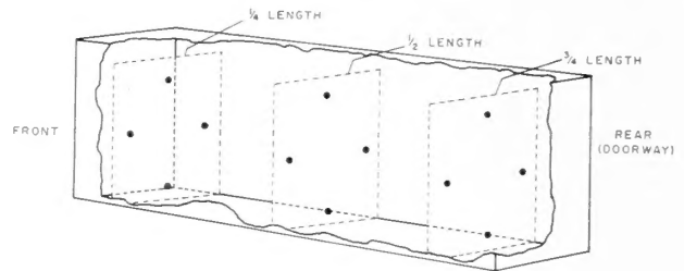
FIGURE 4.—Position of thermocouple sensing points in produce of each test load.
