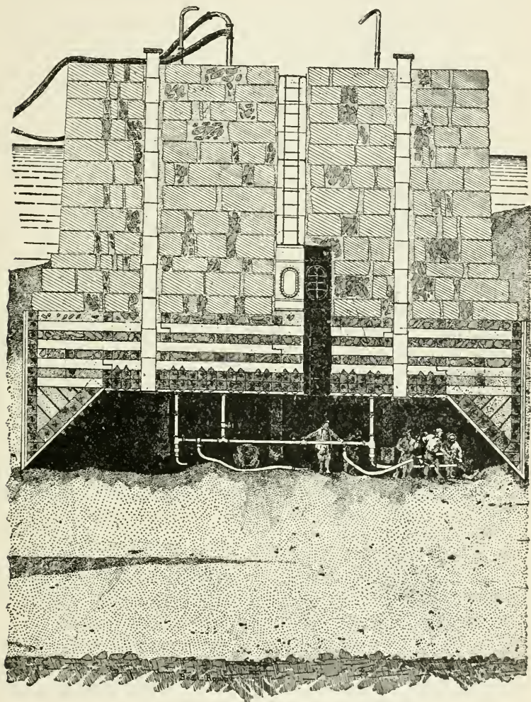
FIG. 65.—PNEUMATIC CAISSON.—BLAIR BRIDGE.
