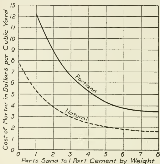
FIG. 7a.—COST OF CEMENT MORTAR.
