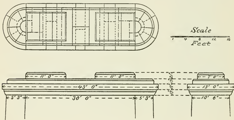
FIG. 88.—TOP OF PIER, HENDERSON BRIDGE.
