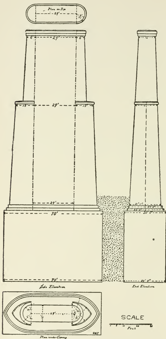
FIG. 85.—CHANNEL PIER, CAIRO BRIDGE.
