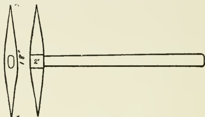
FIG. 12.—PICK.
