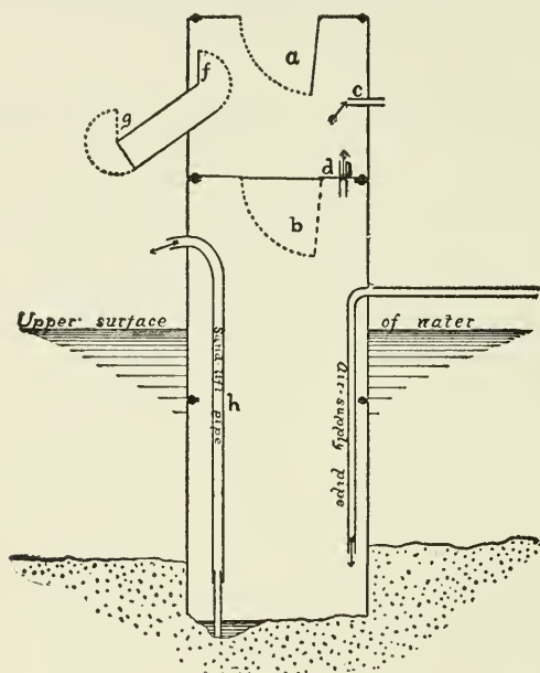
FIG. 63.—PNEUMATIC PILE.
