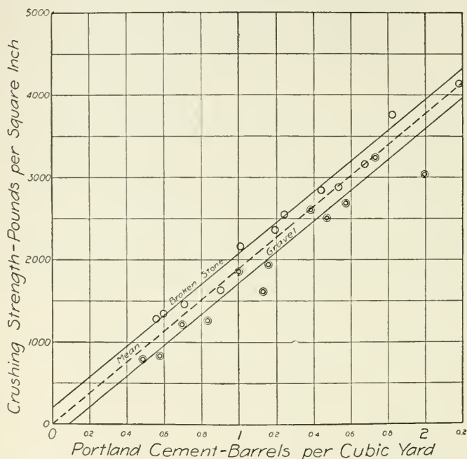
FIG. 8.—RELATION BETWEEN THE STRENGTH OF THE CONCRETE AND THE AMOUNT OF CEMENT.
