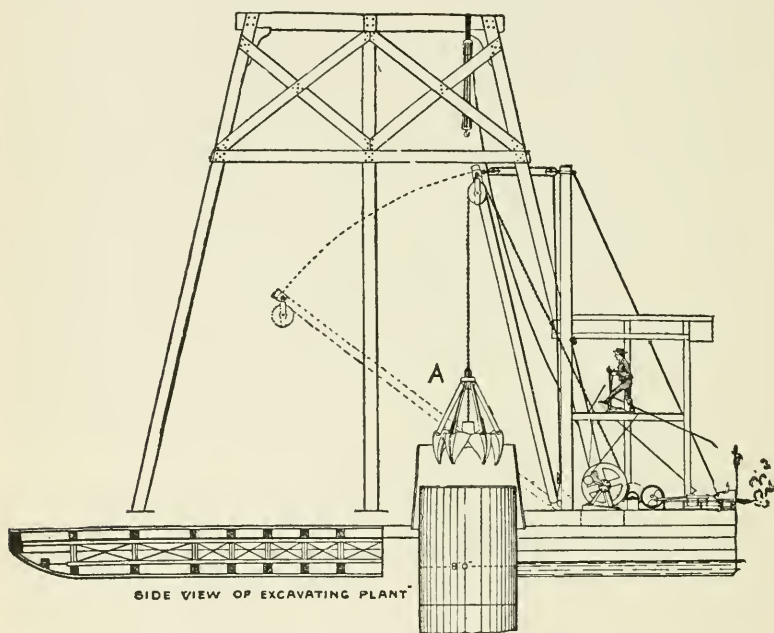
FIG. 62.—SINKING IRON PILE BY DREDGING.
