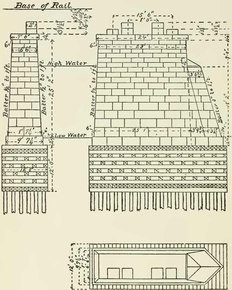
FIG. 90.—PIER OF ST. CROIX RIVER BRIDGE.
