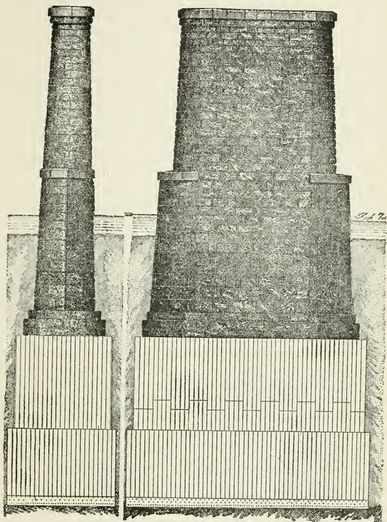
FIG. 87.—SHORE PIER, BLAIR BRIDGE.
