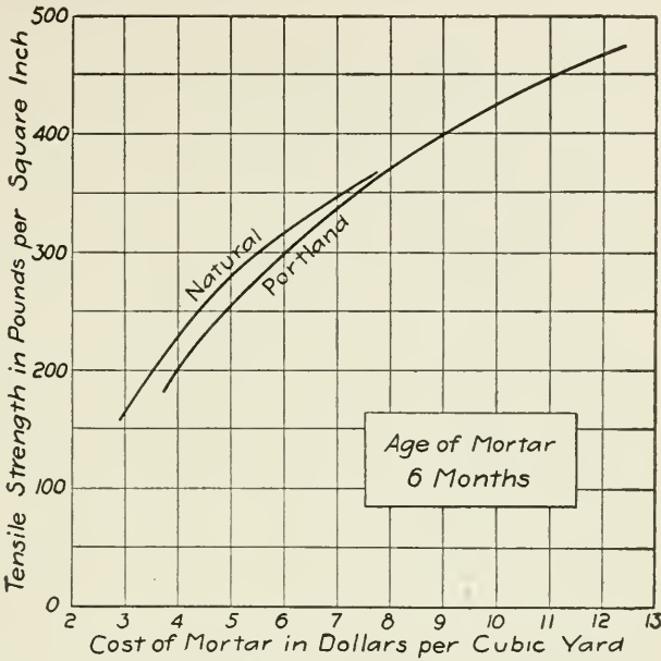
FIG. 7b.—RELATIVE ECONOMY OF NATURAL AND PORTLAND CEMENTS.
