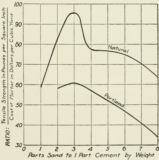
FIG. 7c.—ECONOMIC PROPORTION OF SAND.
