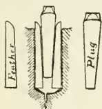
FIG. 25. PLUG AND FEATHERS.
