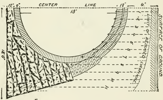
Fig. 148.—Brick Arches for Large Sewers.—Philadelphia Standard
