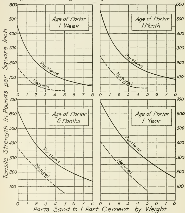
FIG. 6.—DIAGRAM SHOWING RELATIVE STRENGTH OF CEMENT MORTARS.
