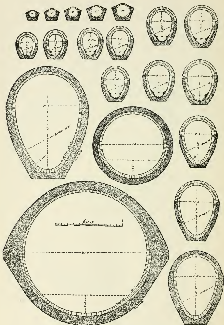
FIG. 149.—Standard Forms of Brick Sewers.—Washington, D. C.
