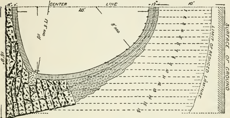
Fig. 148.—Brick Arches for Large Sewers.—Philadelphia Standard
