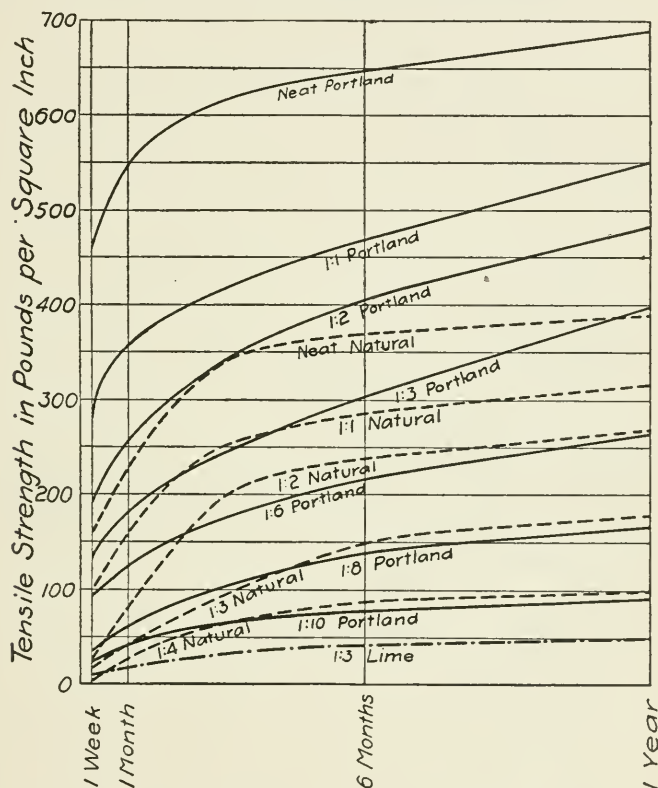
FIG. 5.—DIAGRAM SHOWING EFFECT OF TIME ON STRENGTH OF MORTARS.
