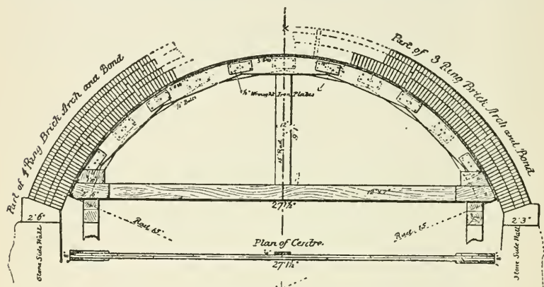
FIG. 147.—Bond and Center of Vosburg Tunnel.
