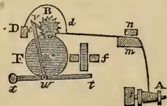
Fig. 18. DOUBLING MACHINE.
